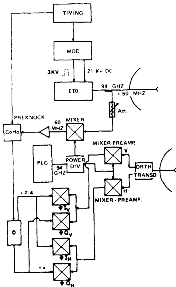
Fig.1 Radar Block Diagram.
