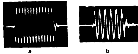
Fig.3 IF signal at the output of the phase lock mixer. IF frequency is approximately 50 MHz. Time exposure is 2 seconds. a. 300 ns pulse. b. 100 ns pulse. Note that the signal noise in the beginning and the end of the pulse does not exceed 10 ns.
