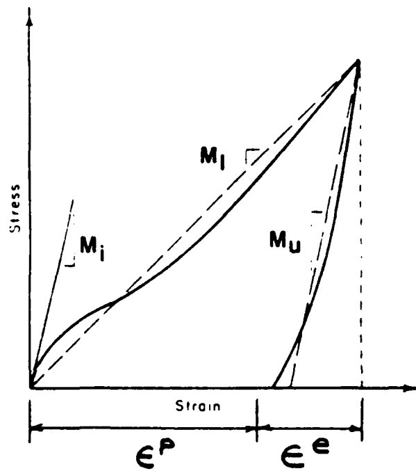
Figure 2. Typical Stress-Strain Response Under Uniaxial Conditions
