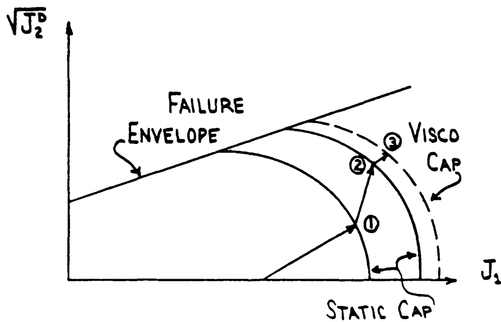
Figure 3. Plasticity surfaces for Visco-Plastic Cap Model
