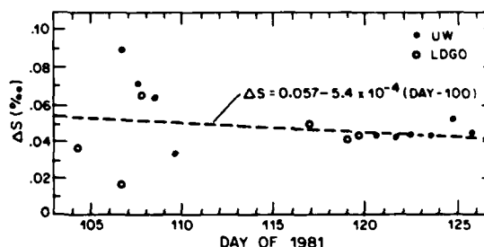
Figure 4. The difference, \Delta S , between sample bottle salinities and SALARGOS buoy salinities at Fram III plotted versus day of 1981. \Delta S = S_{\text{Bottle}} - S_{\text{Buoy}} . A least squares linear fit to the data is shown as a dashed line. The buoy salinities average 0.05 o/oo less than the bottle salinities.
