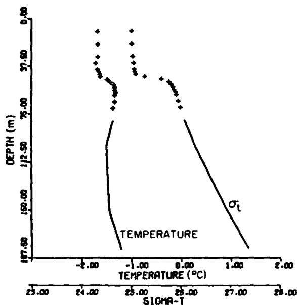
Figure 2. Typical temperature and \sigma_t profiles from T-3. Note the temperature maximum below the mixed layer. The profile was made 4/26/70.
