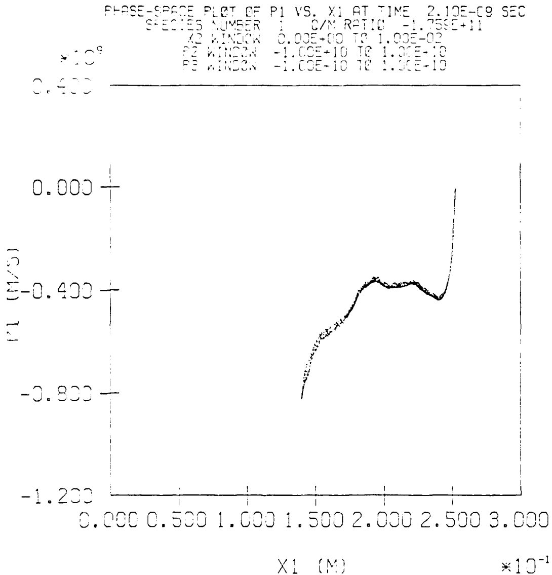
Figure 24. Phase-Space Plot of Central Beam Electrons for Low Current Test at t = 2.1 \text{ nsec.}
