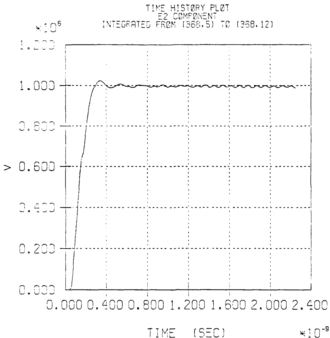
Figure 27. Temporal History of Voltage Pulse Applied to Rod Cathode for New Model Benchmark Case.
