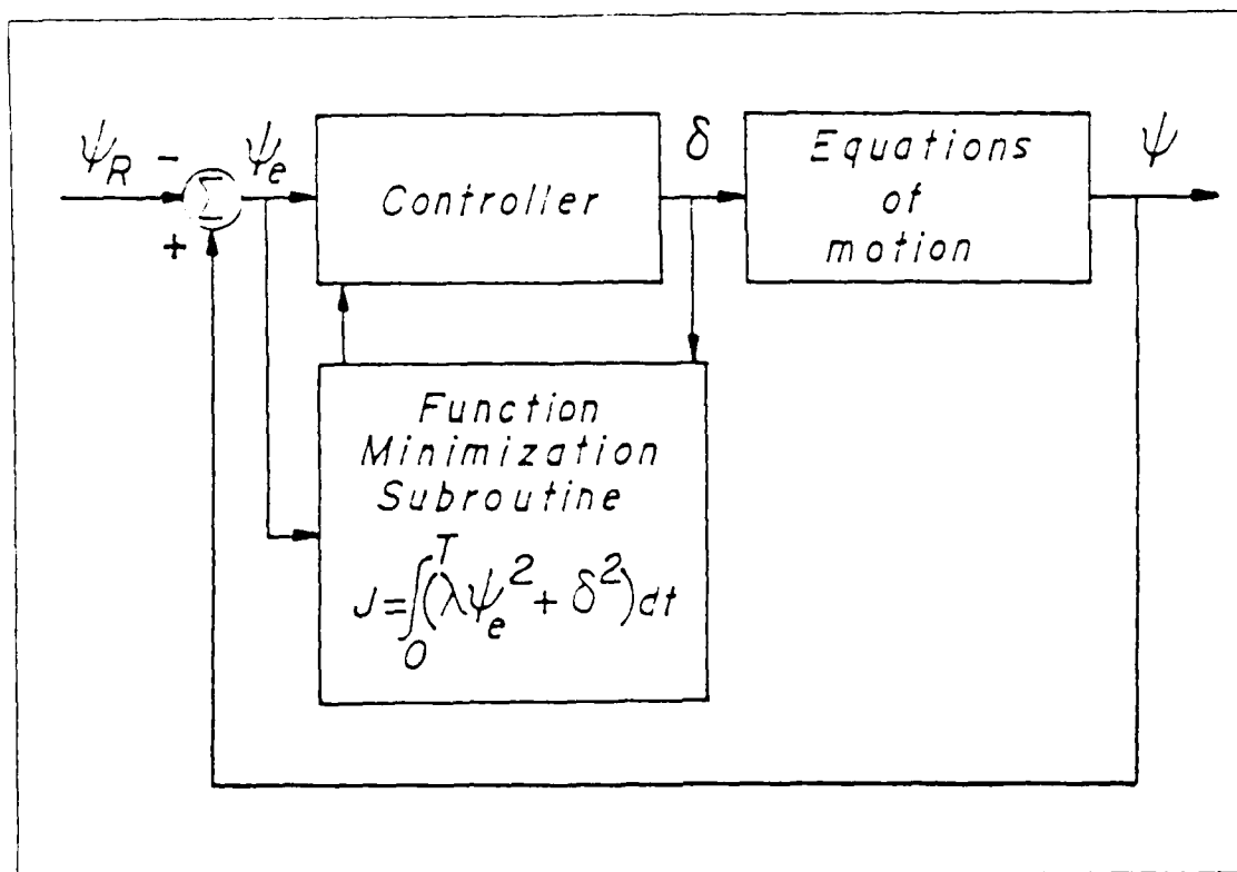
Figure 2.1 Controller Optimization Scheme
