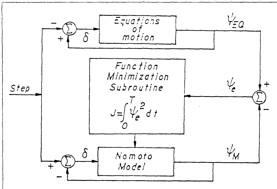
Figure 2.3 Nomoto Model Determination Scheme
