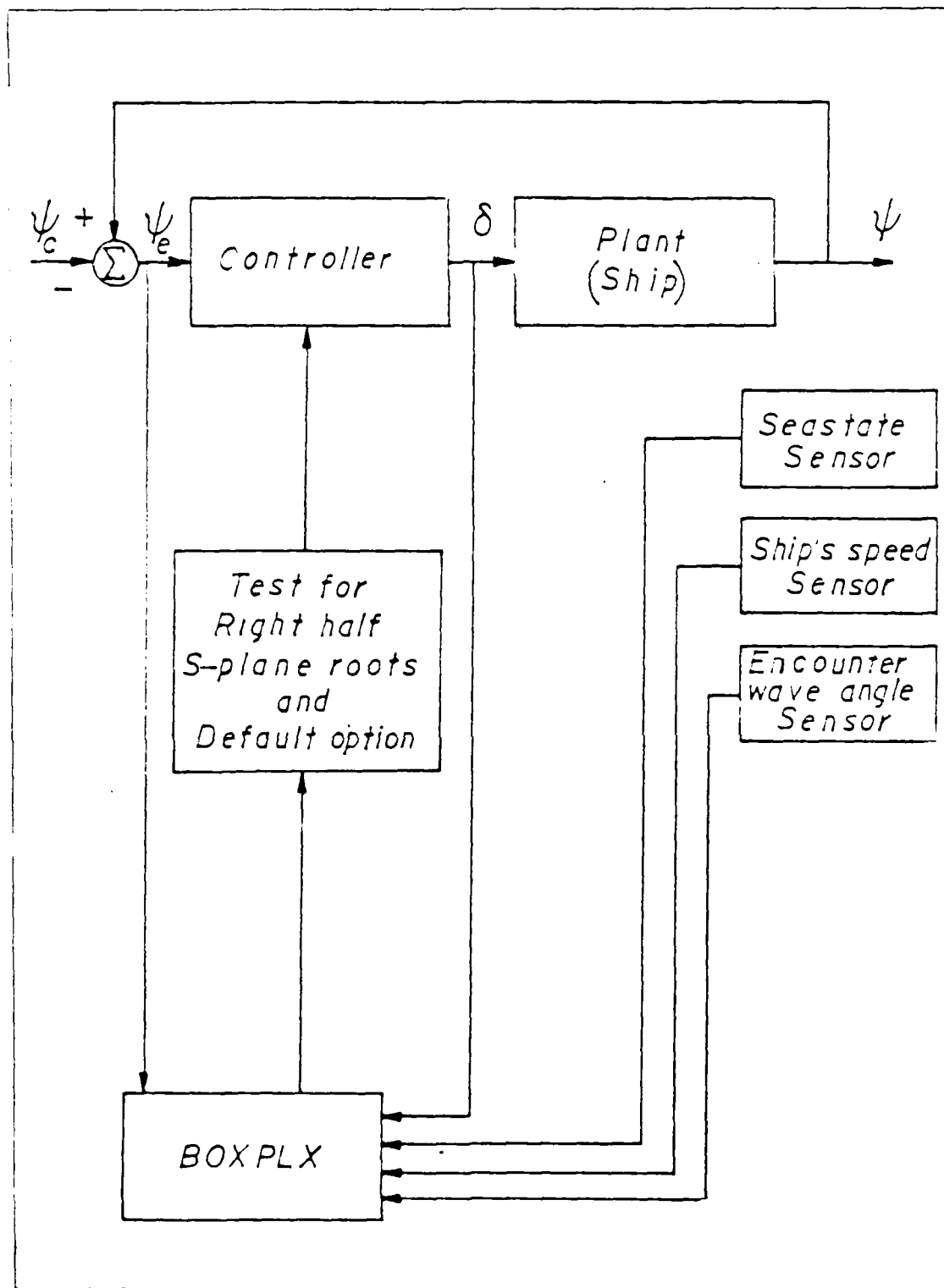
Figure 7.2 On Line Adaptive Scheme
