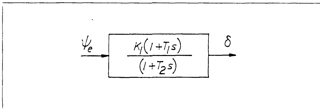
Figure 4.1 Controller Used in this Study
