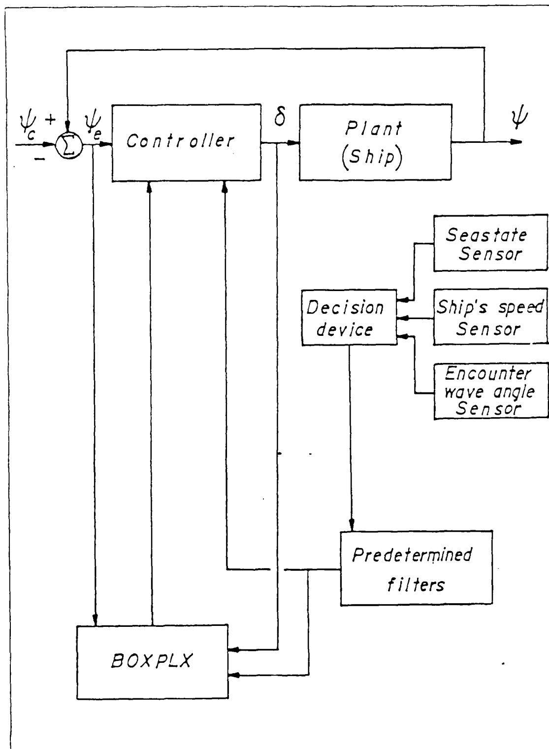
Figure 7.1 Adaptive Control Scheme
