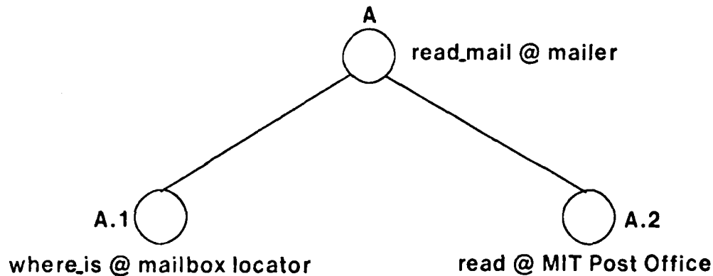
Figure 3-5: Action Tree of an Example Computation
