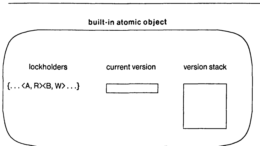
Figure 2-1: A Stylized Picture of a Built-in Atomic Object
