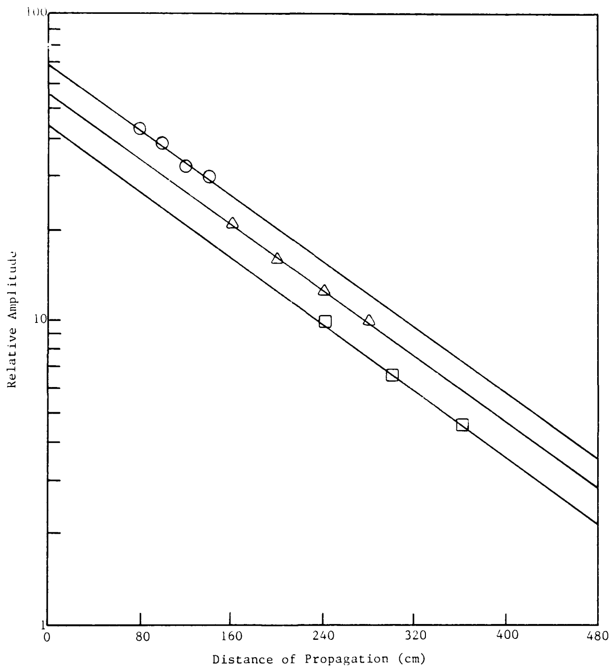
FIGURE 3. Sound amplitude vs distance of propagation in stable N_2 at pressure = 20 Torr; frequency = 2 kHz; tube radius = 1.27 cm. \circ - m=1 (first reflection); \Delta - m=2 (second reflection); \square - m=3 (third reflection).
