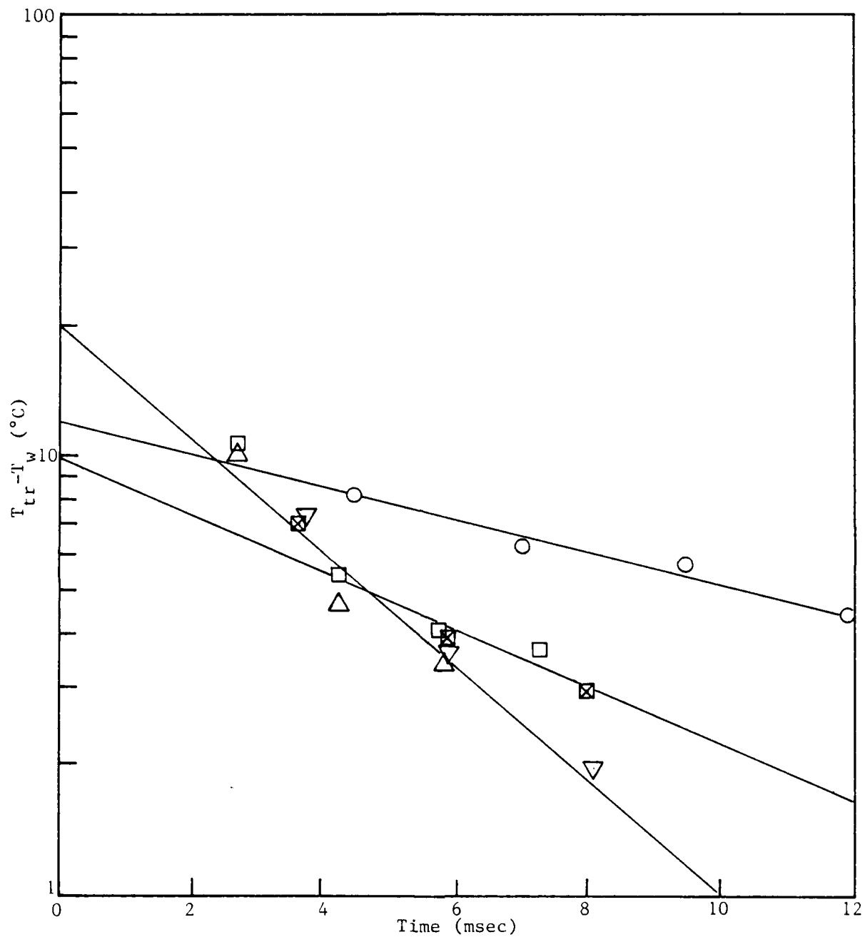
FIGURE 8. The difference between translational and wall temperature ( T_{tr} - T_w ) as a function of time observed in 25% He - 75% N_2 mixture. \Delta T_w^{tr} pressure (P) = 20 Torr; tube radius (R) = 0.615 cm; tube length (L) = 30 cm. \nabla - P = 20 Torr; R = 0.615 cm; L = 43 cm. \square - P = 40 Torr; R = 0.615 cm; L = 30 cm. \boxtimes - P = 40 Torr; R = 0.615 cm; L = 43 cm. \circ - P = 20 Torr; R = 1.27 cm; L = 50 cm. Solid lines are least squares fit to data.
