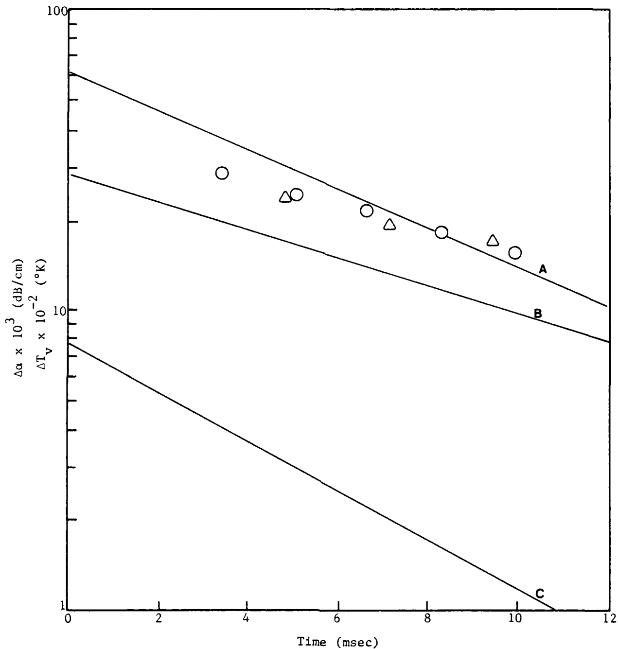
FIGURE 10. Gain ( \Delta\alpha ) as a function of time observed in 10% H_2 - 90% N_2 mixture at pressure = 40 Torr; tube radius = 0.615 cm; discharge energy = 48.8 \times 10^5 joule/mole. Data points, O - observed at tube length = 30 cm; \Delta - observed at tube length = 43 cm. Curve A is calculated gain setting d(\ln \tau_v^{-1})/dT = 0.05 . Curve B is \Delta T_v \times 10^{-2} computed from Equation 37. Curve C is the calculated gain by setting d(\ln \tau_v^{-1})/dT = 0.01 .
