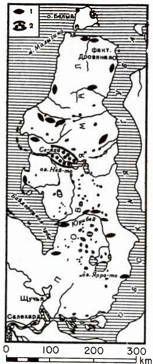
Figure A9. Distribution of injected fossil ice on the Yamal Peninsula. (From Dubikov and Kopeyska 1964.) 1 -individual deposits of ice; 2 - region where many ice deposits are located.
