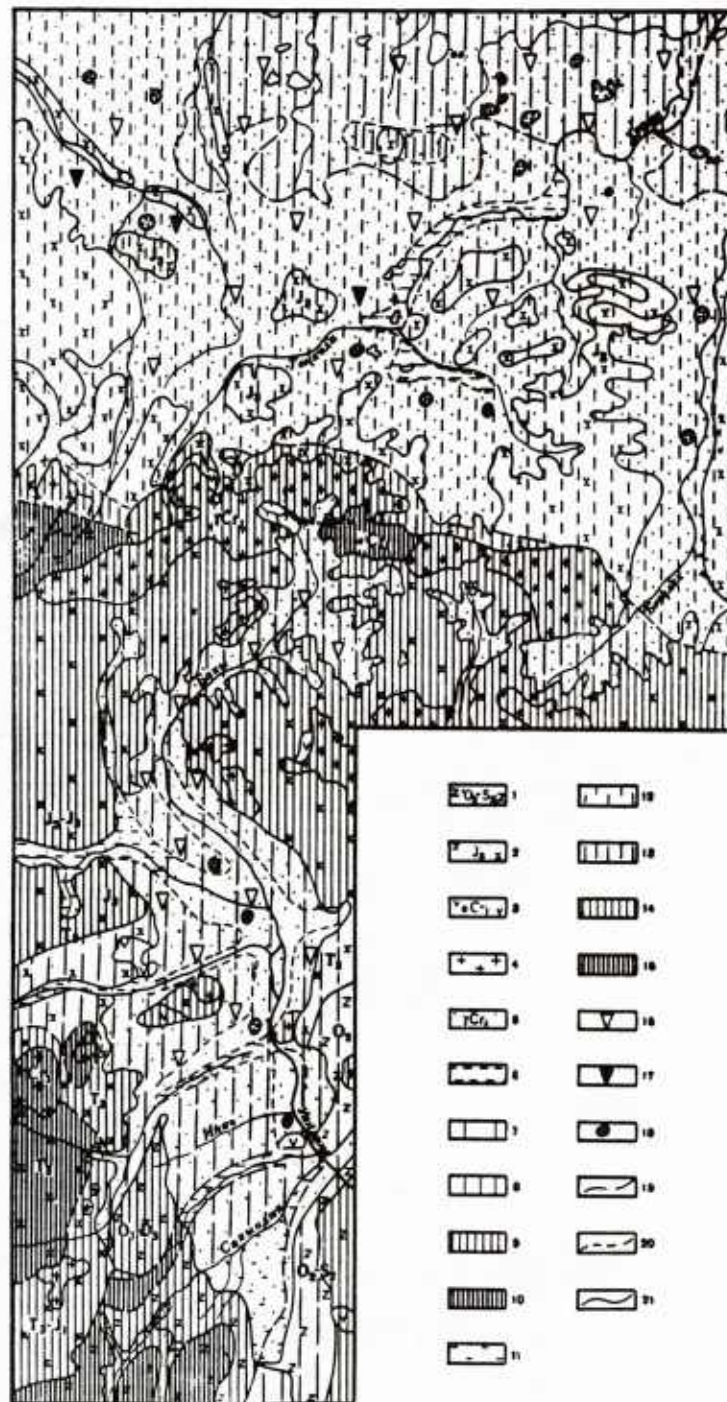
Figure Al8a. Permafrost and age and composition of rock in the Iana-Indigirka depression. (From Kudriavtsev et al. 1973.)
