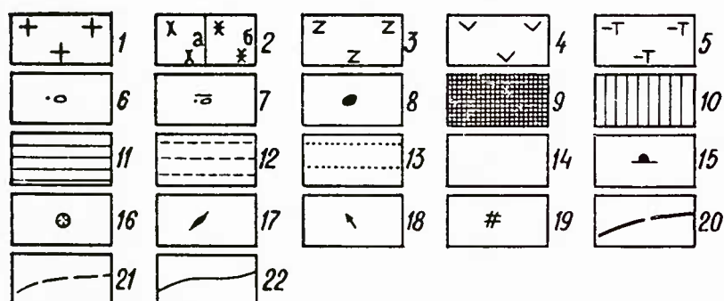
Figure A41. Permafrost of the southern part of the Far East. (From Zamolotchikova and Smirnova 1978.)
