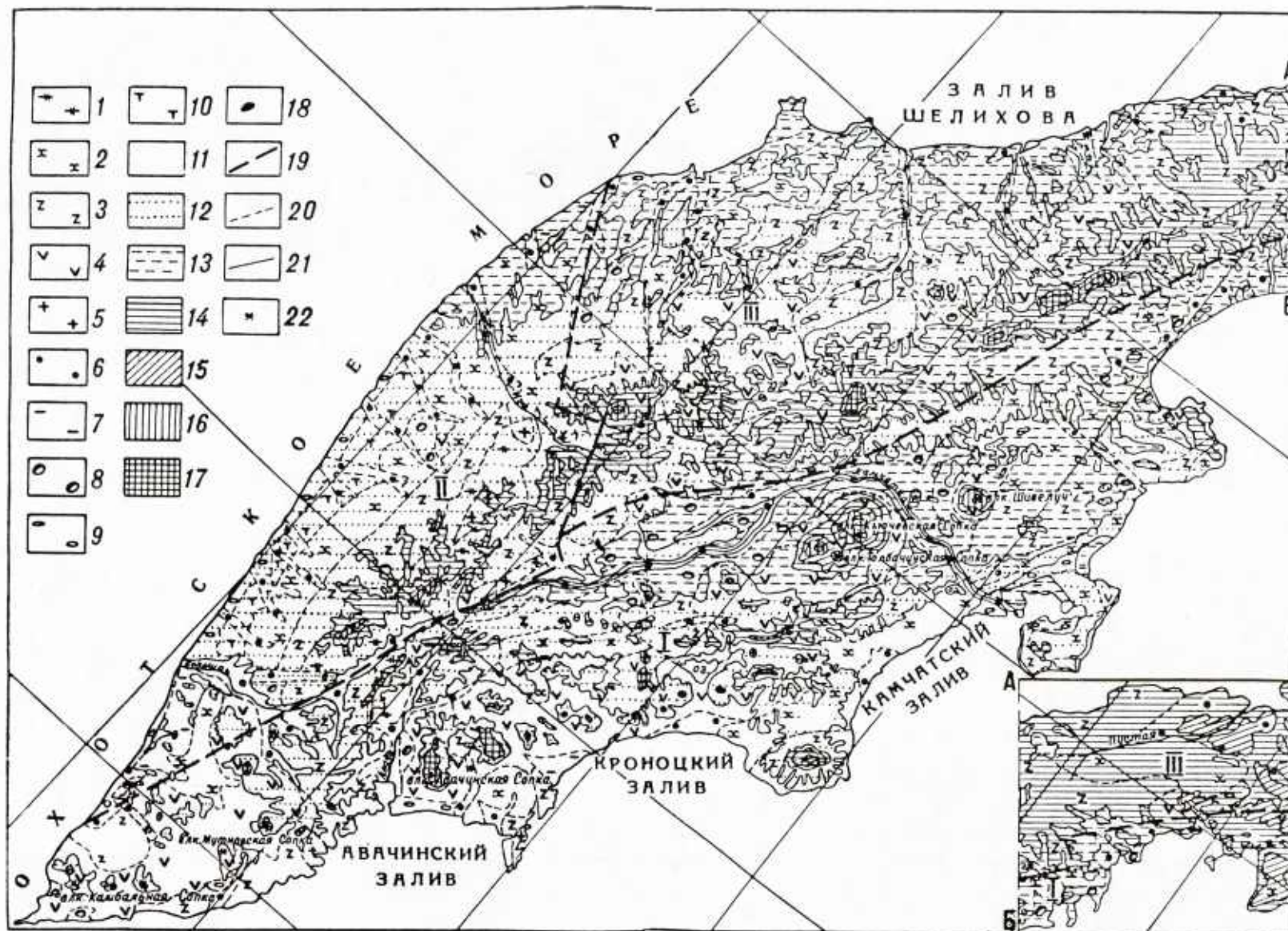
Figure A42. Kamchatka rock temperatures. (From Zamolotchikova and Smirnova 1979.)
