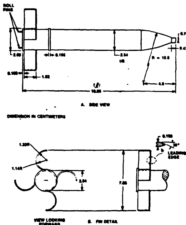
Figure 1. Model Configuration
