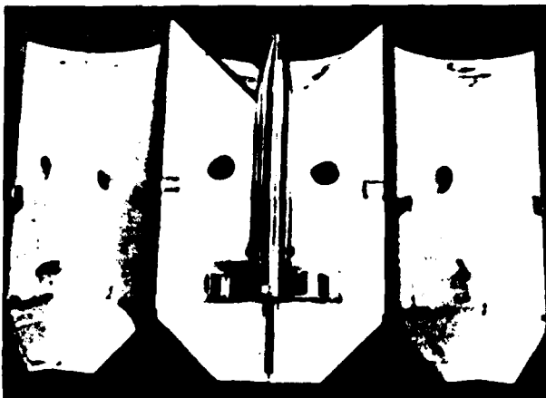
Figure 2. Model/Sabot Package
