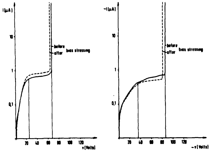
Current-voltage characteristic: Preevaporation etchant: H_2SO_3 + H_2O_2 + H_2O positively bias-stressed
