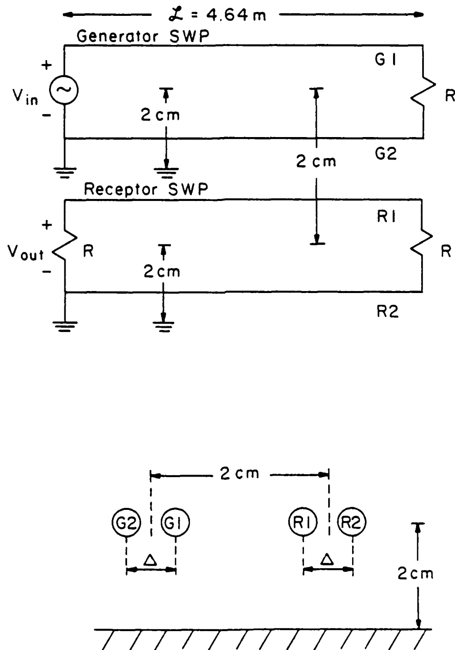
FIGURE 4-2. THE SWP TO SWP EXPERIMENT. (a) LONGITUDINAL VIEW. (b) CROSS-SECTIONAL VIEW.
