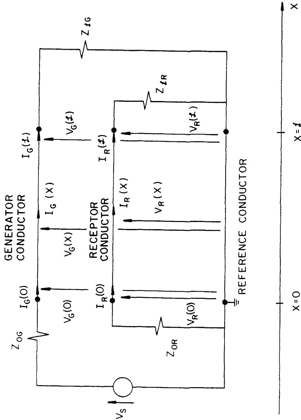
FIGURE 2-2. THE THREE-CONDUCTOR TRANSMISSION LINE.
