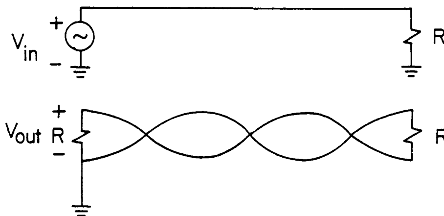
(a) The Unbalanced, Twisted Pair
