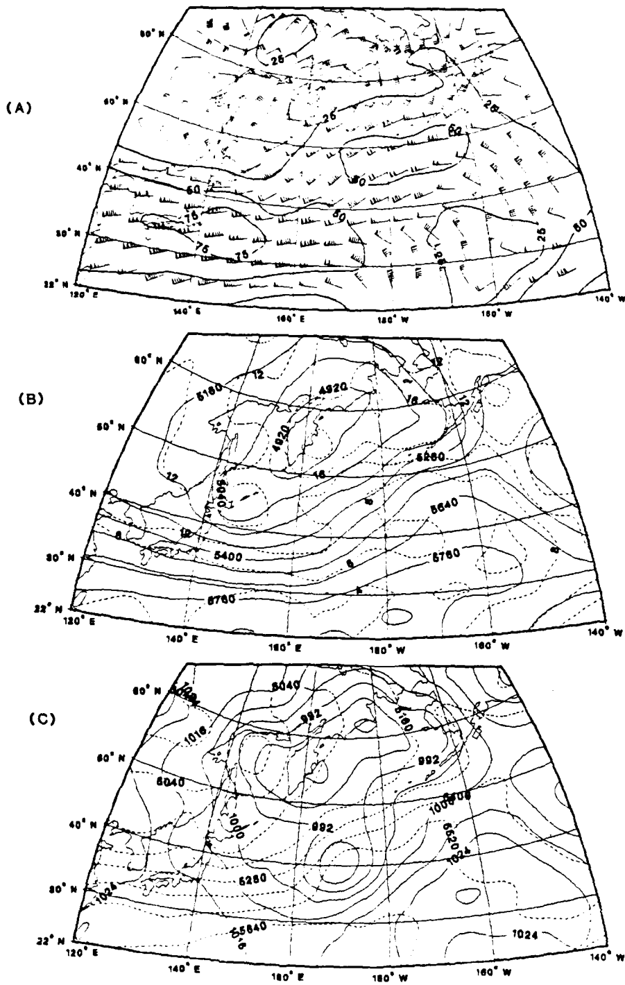
Figure 4. As in Figure 2 except for GLAS Analysis 0000 GMT 14 January
