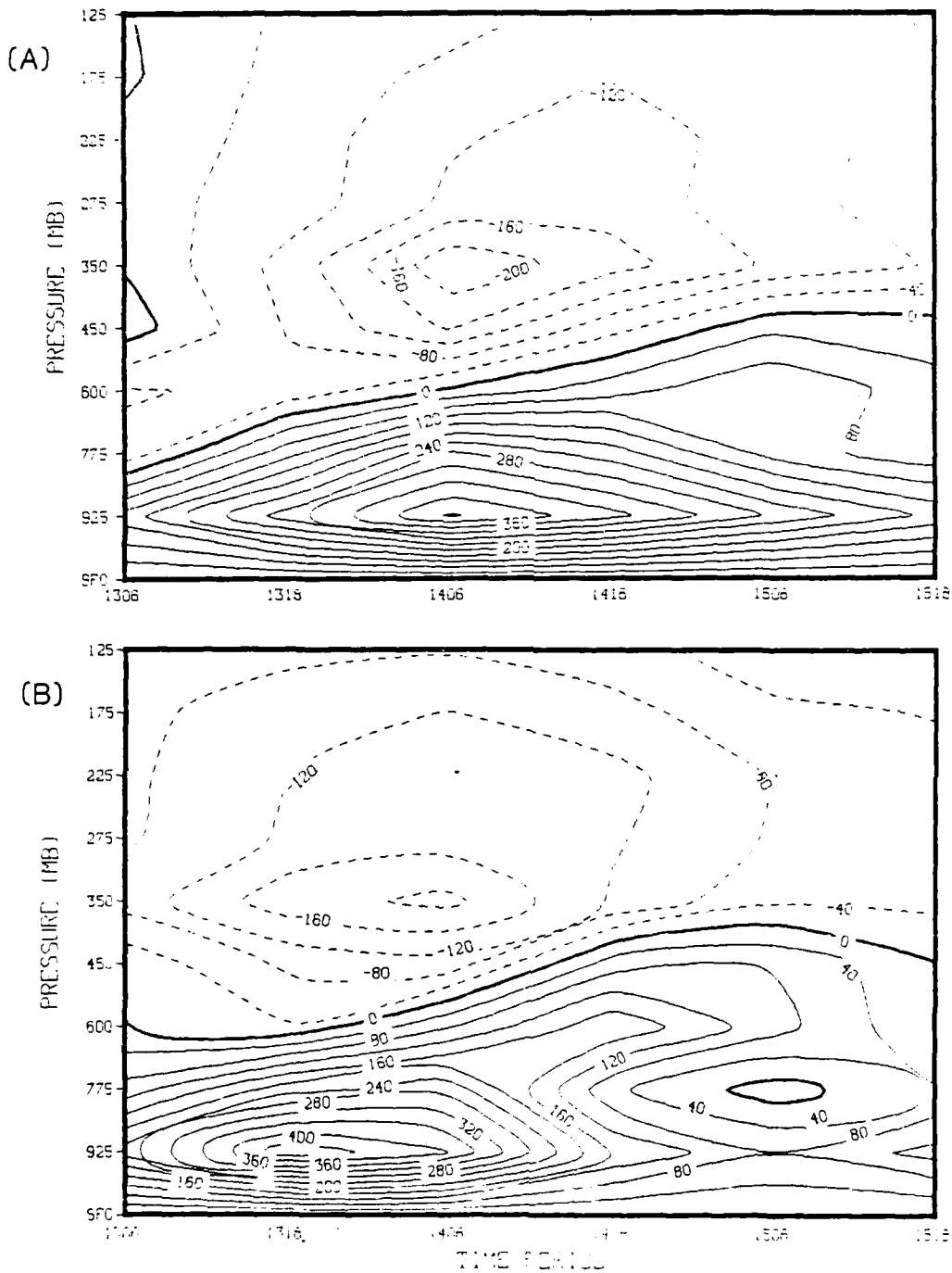
Figure 30. Analyses Corrected Lateral Mass Transport Time Sections (A) GLAS (B) ECMWF. Contour Interval is 40 \times (10^{11}) . Negative Values (DASHED) Indicate Flux out of the Volume. Units are in gm/sec-100 mb. Period 1300 Refers to 00-12 GMT 13 January.
