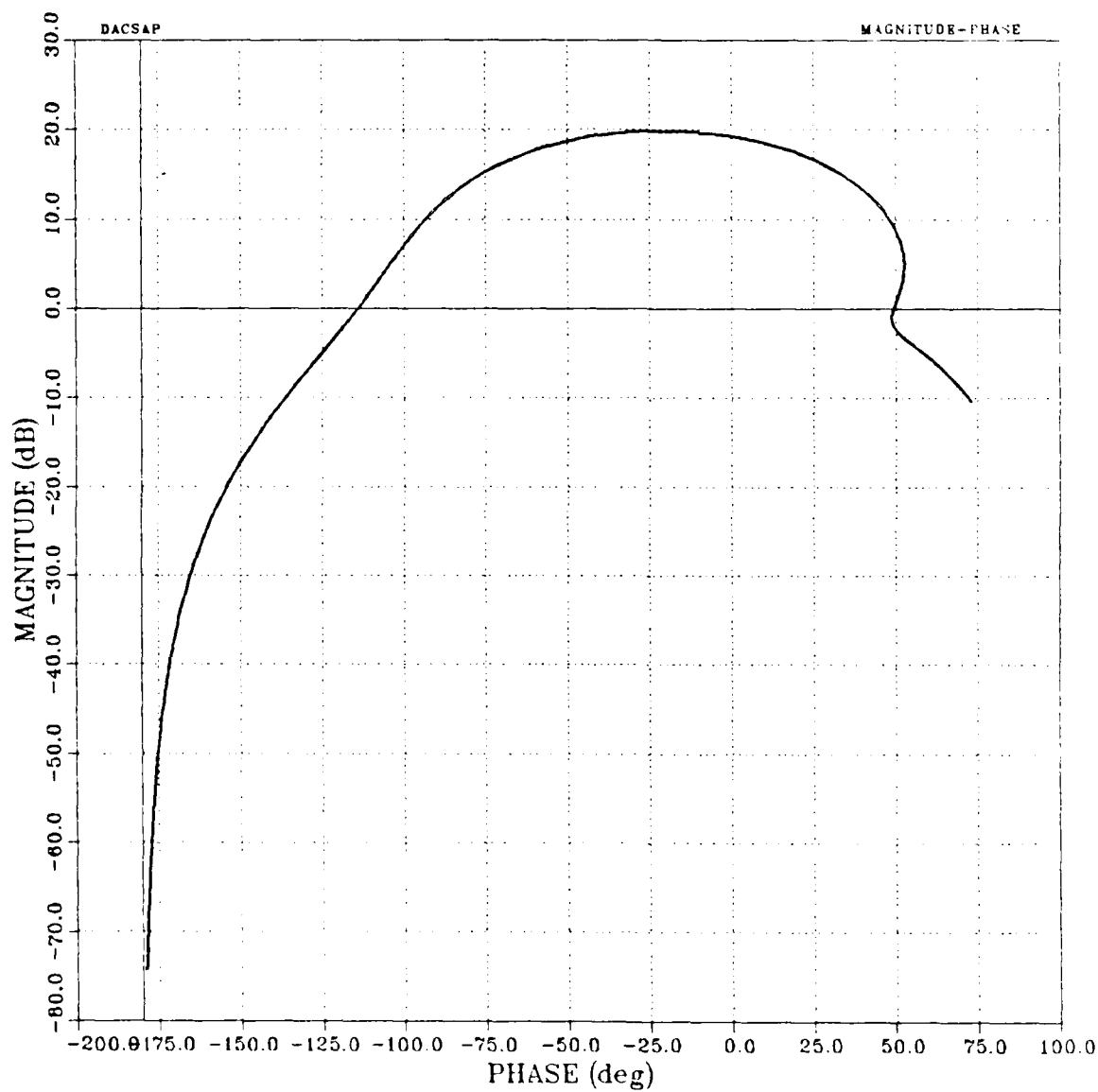
Figure 3.12 Log Magnitude-Phase Plot.
