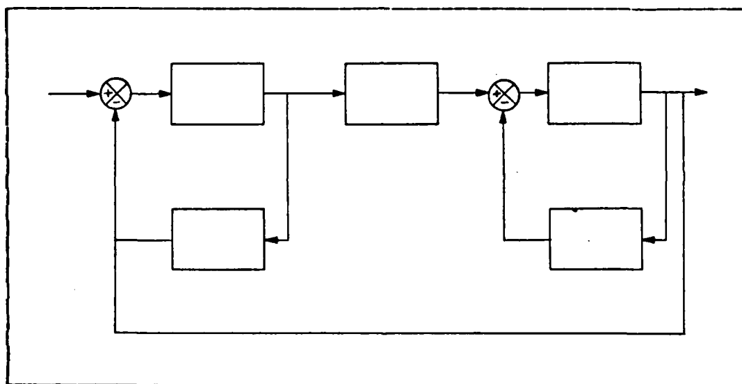
Figure A.9 Inner Loops in Series.
