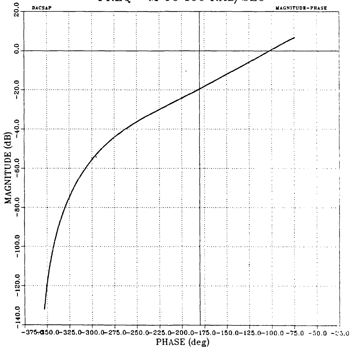
Figure A.5 Sample Log Magnitude-Phase Plot.
