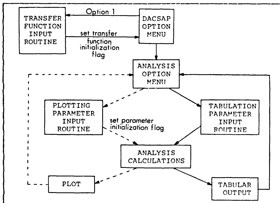
Figure 3.2 Control Structure Before Parameter Initialization.
