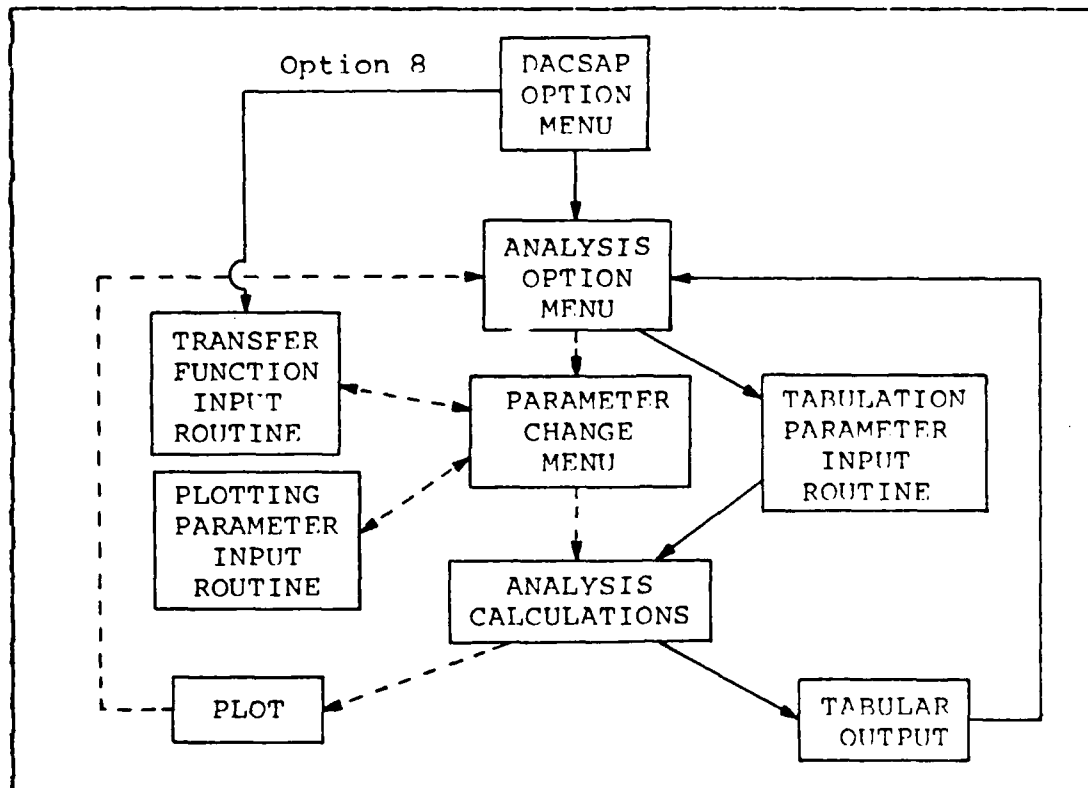
Figure 3.3 Control Structure After Parameter Initialization.
