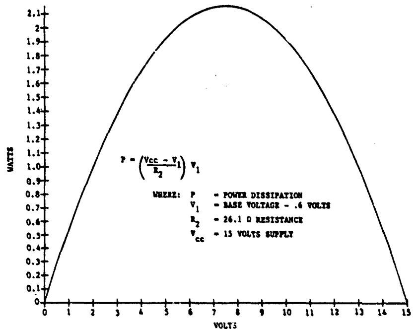
Figure 79. Power Dissipation Circuit
