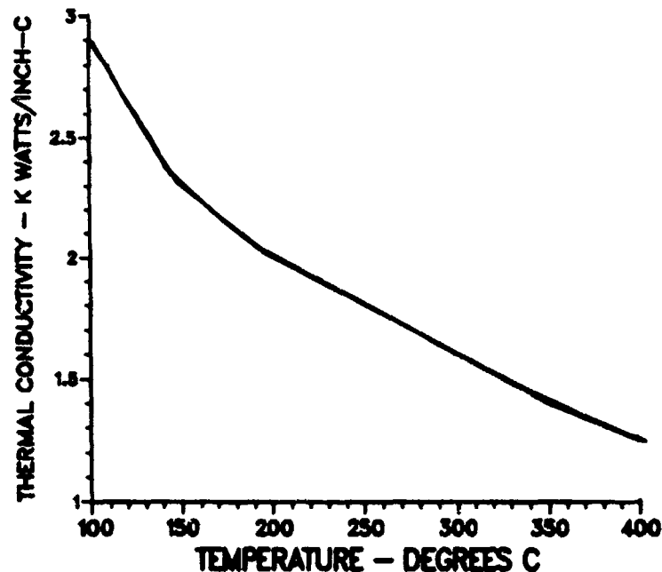
Figure 76. Silicon Thermal Conductivity versus Temperature
