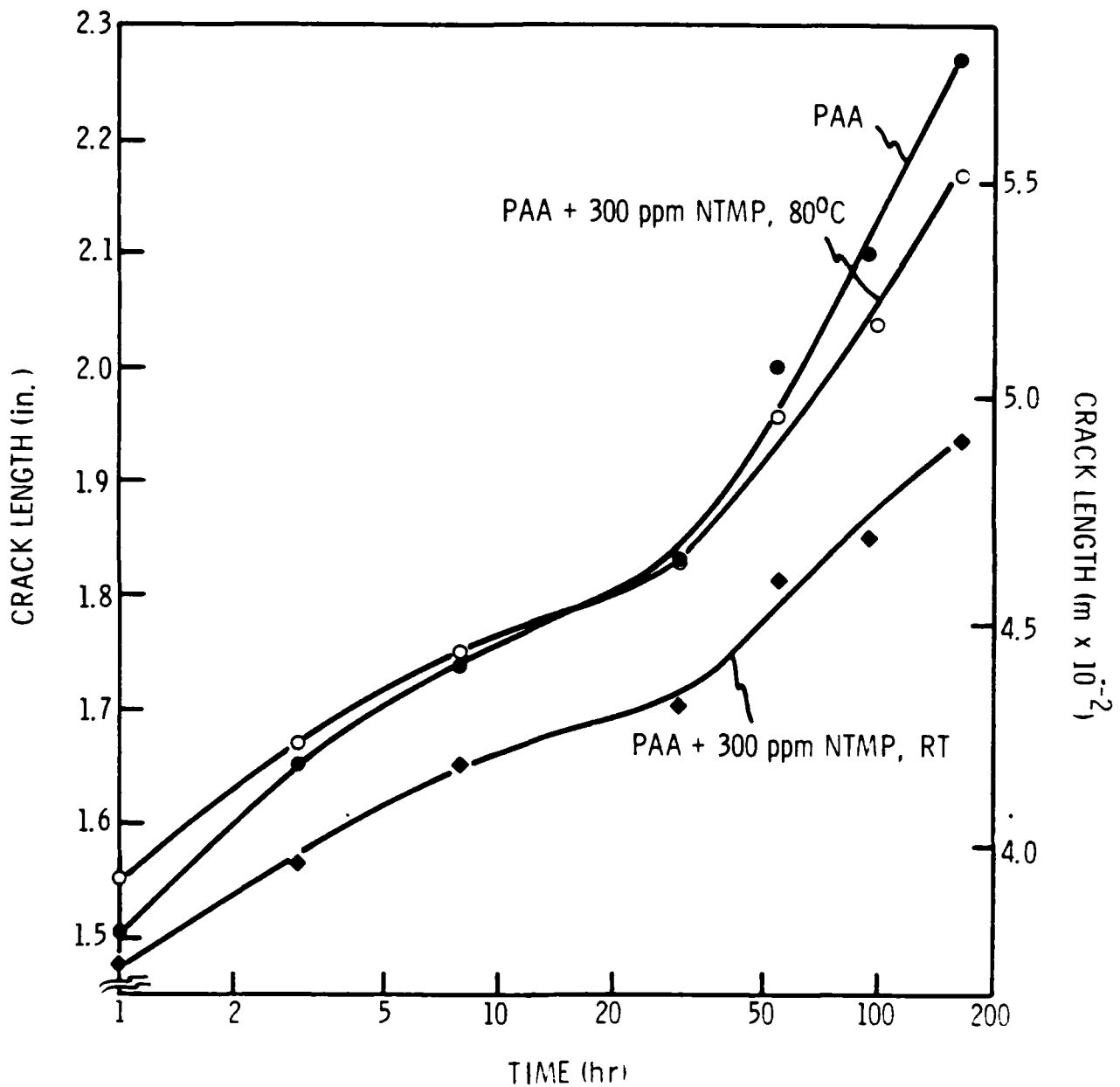
Figure 24. Wedge test results (crack length as a function of time) for untreated PAA adherends and PAA adherends treated in 300-ppm NTMP solutions at either room temperature or 80°C. (18)
