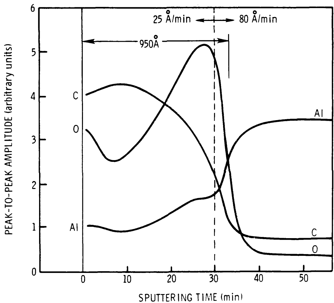
Figure 31. AES depth profile of "shiny" region on Al side of PAA wedge-test. (18)
