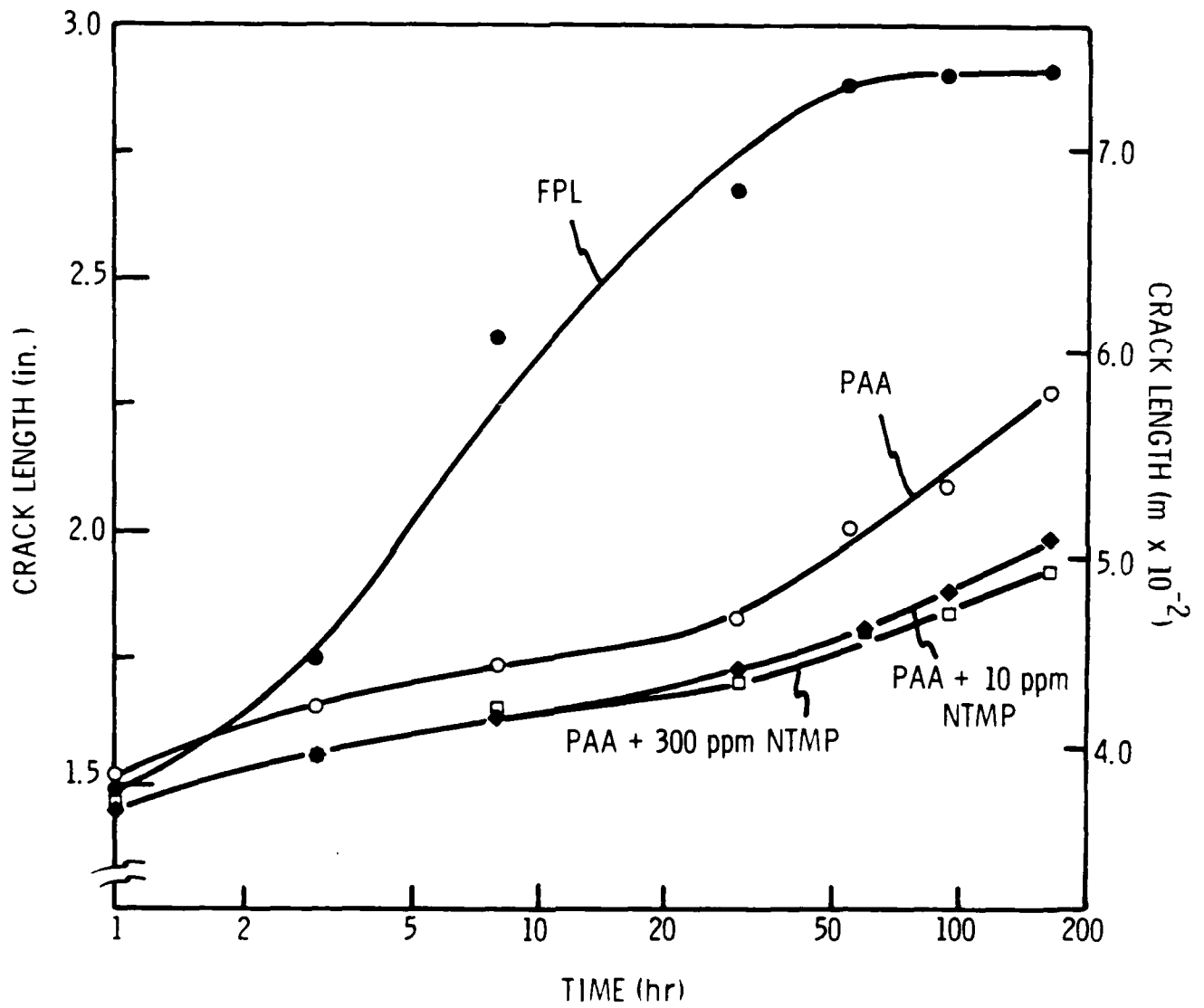
Figure 23. Wedge test results (crack length as a function of time) for untreated FPL and PAA adherends and PAA adherends treated with 10-ppm and 300-ppm NTMP solutions. (18)
