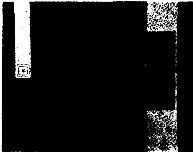
Figure 13. Photomicrograph of failure site in Al-metallized, mode-2 mainstream failure: contact L, contact 1, and vicinity at 500X magnification.
