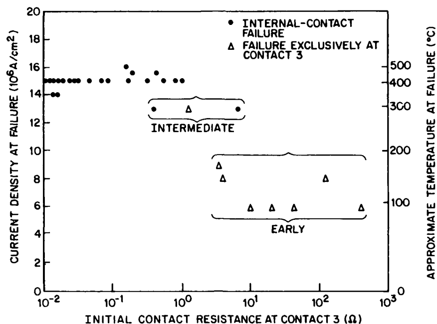
Figure 20. Current density at failure (and approximate temperature at failure) versus initial contact resistance at contact 3 for early, intermediate, and mainstream mode-2 failures.
