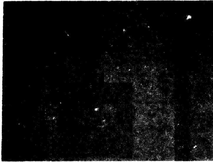
Figure 25. Photomicrograph of Al-1%Si metallized CRTV in which the Al-Si interconnect has been stripped, but in which the interconnect pattern is still visible as Si precipitates (freckles) on interlevel dielectric surface: contacts L, 1, and 2 and vicinity at 200X magnification.
