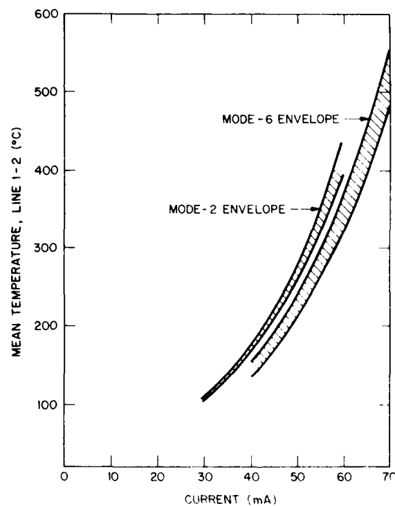
Figure 26. Mean line temperature of CRTV line segment 1-2 versus current for units during 10-minute mode-6 testing, with corresponding mode-2 envelope repeated from Figure 10 for comparison.
