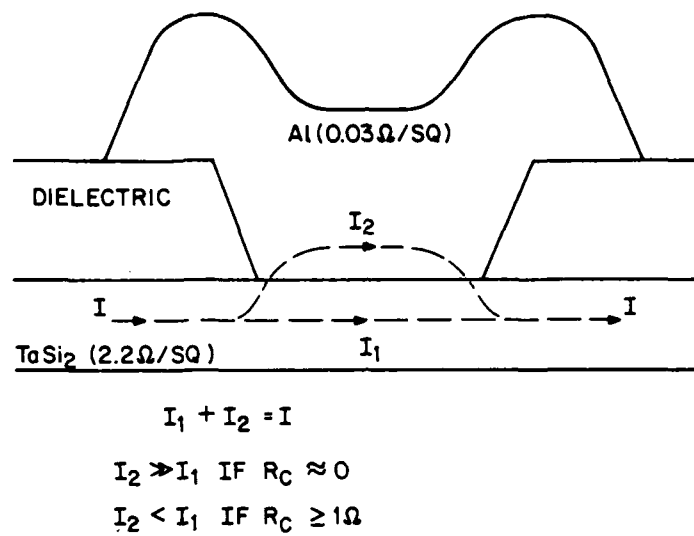
Figure 21. Schematic cross-section diagram showing probable current paths for polycide-line current crossing an internal contact.
