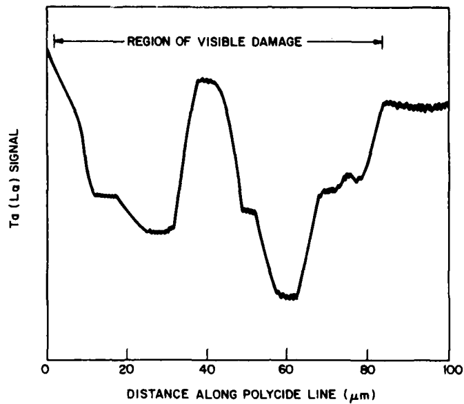
Figure 32. Ta ( L\alpha ) EPM x-ray counts versus distance along polycide line of failed CRTV unit.
