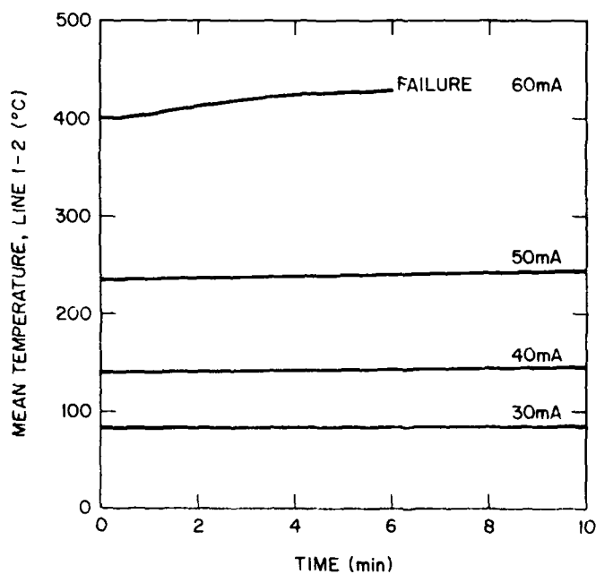
Figure 9. Mean temperature of CTV line segment 1-2 versus time during 10-minute mode-2 testing increments at the currents as labelled.
