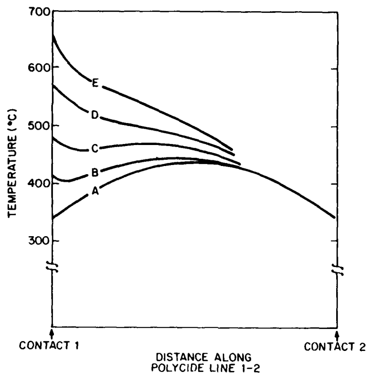
Figure 17. Speculative temperature distribution along line segment 1-2 during powering for undamaged line (curve A), and during the thermal runaway process leading to failure and Al melting at contact 1 (curves B to E).
