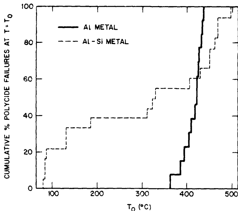
Figure 12. Cumulative polycide-line failure distribution plots versus mean line-segment temperature for Al- and Al-Si metallized units under 10-minute testing in mode 2.
