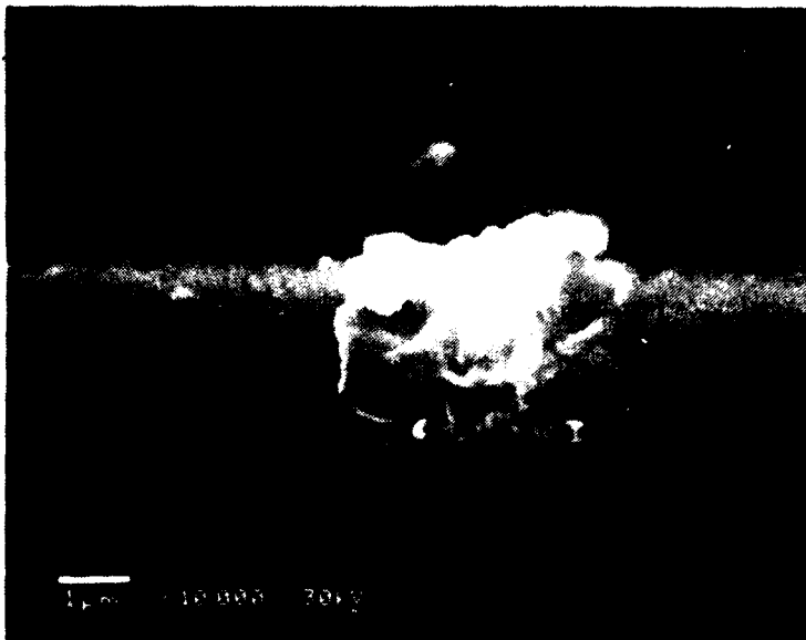
Figure 37. Scanning-electron micrograph of CRTV mode-2 early failure from which Al-1%Si film has not been stripped: contact 3 and vicinity at 10,000X magnification.
