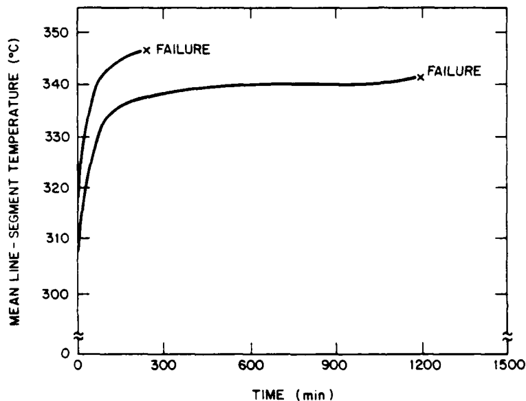
Figure 28. Mean temperature of line segment 1-2 versus time for two CRTV units powered to failure at a current density of 1.5 \times 10^7 \text{ A/cm}^2 in mode 6.
