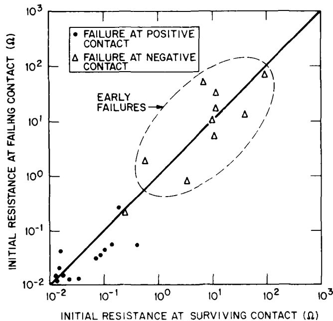
Figure 27. Logarithmic plot of initial contact resistance at failing contact (in mode-5 or mode-6 testing) versus initial contact resistance at surviving contact. Diagonal line at 45^\circ is line of equality of these two resistances.
