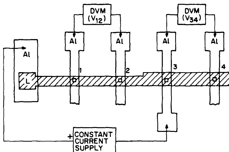
Figure 8. Schematic diagram of CTV mode-2 electrical connections.
