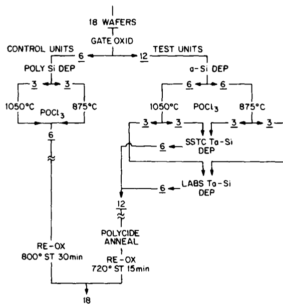
Figure 2. QMOS process flow diagram: control and test branches.
