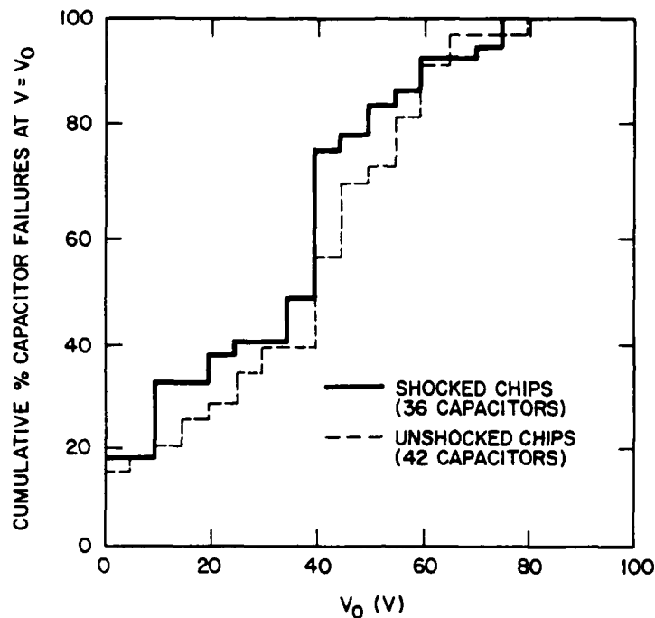
Figure 7. Cumulative gate-breakdown-voltage failure distribution plots for thermally shocked and unshocked CRTV polycide capacitors with a 500 Å steam-grown gate oxide.
