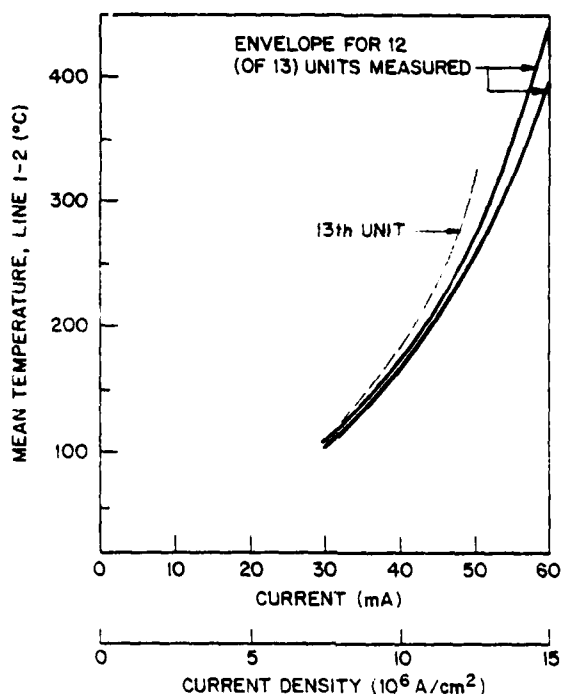
Figure 10. Mean temperature of CRTV line segment 1-2 versus current and current density for 13 units during 10-minute mode-2 testing.
