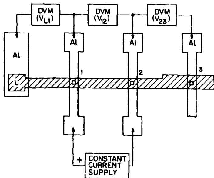
Figure 23. Schematic diagram of CRTV mode-6 electrical connections.
