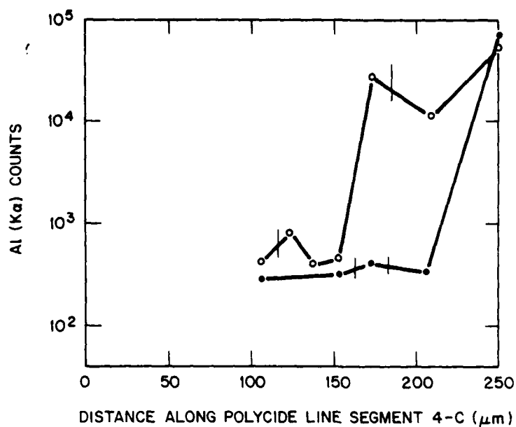
Figure 39. Al (K \alpha ) EPM x-ray counts versus distance along polycide line for the CRTV mode-7 failures pictured in Figures 29 and 30.
