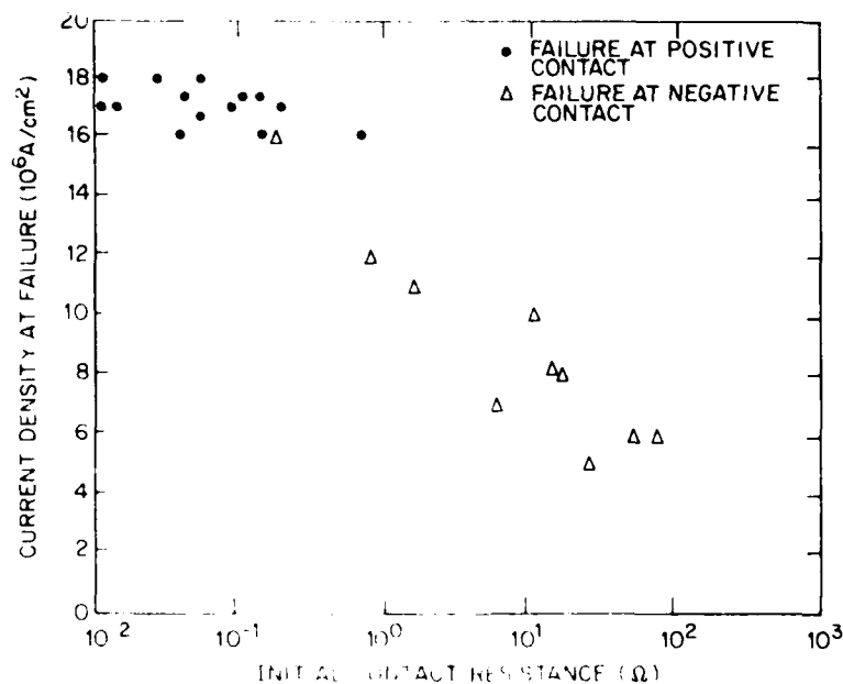
Figure 24. Current density at failure versus the initial contact resistance of the contact which eventually experiences failure. Includes "early" failures at negative contact, and mainstream failures at positive contact.
