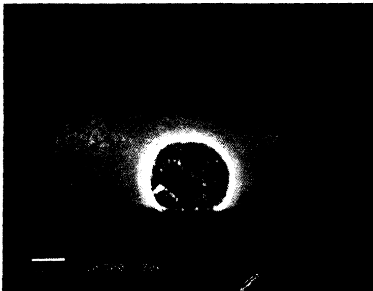
Figure 36. Scanning-electron micrograph of the same CRTV unit shown in Figure 33, contact 4 and vicinity at 10,000X magnification.
