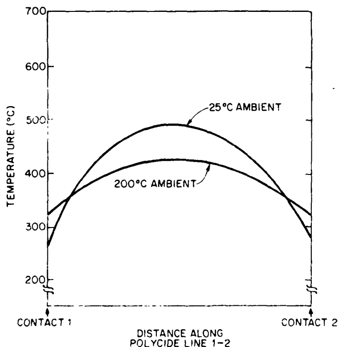
Figure 22. Speculative temperature distributions along line segment 1-2 during mode-2 powering at 25°C-ambient and 200°C-ambient temperatures.
