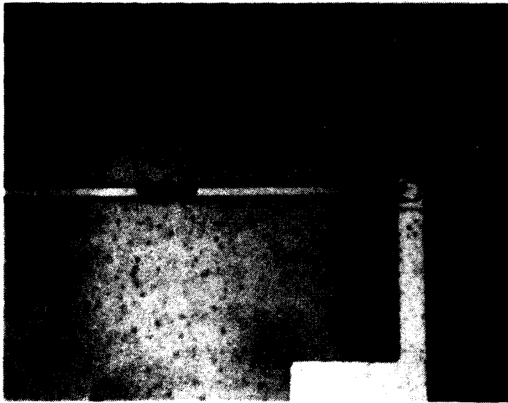
Figure 29. Photomicrograph of failure site in Al-metallized mode-7 failure: contact C and vicinity at 760X magnification.
