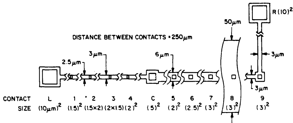
Figure 3. Schematic diagram of CRTV polycide line showing TaSi 2 /Al contacts.
