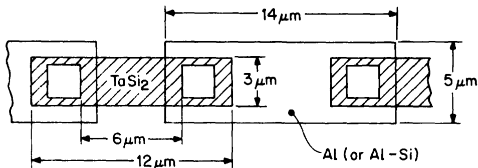
Figure 4. Schematic diagram of portion of CRTV series-contact string.
