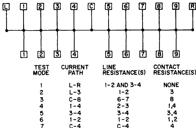
Figure 5. Schematic diagram of CTV polycide line, contacts and bond pads, with tabulations of electrical connections used in test modes 1 to 7.
