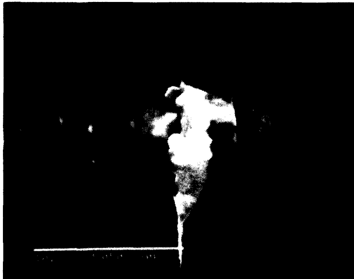
Figure 33. Scanning-electron micrograph of CRTV mode-2 mainstream failure at contact 1, in which Al film had been stripped: contact 1 and vicinity at 5000X magnification.
