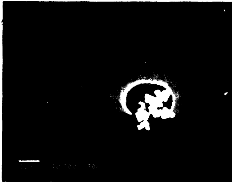
Figure 34. Scanning-electron micrograph of the same CRTV unit shown in Figure 33: contact 2 and vicinity at 10,000X magnification.
