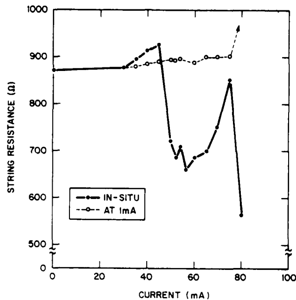
Figure 31. Series-string terminal resistance versus current: in-situ measurements, and measurements at 1mA after 10-minute powering increments at each current.
