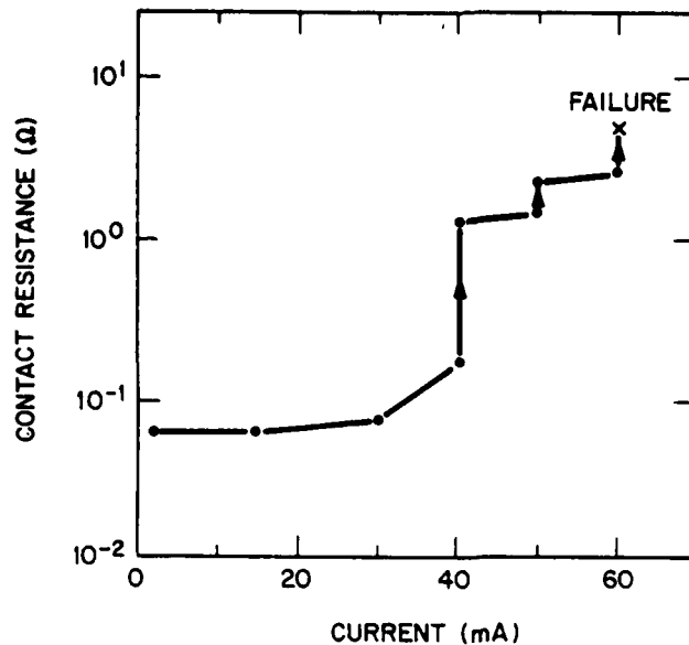
Figure 11. Contact resistance of contact 3 versus current for a unit which experienced contact degradation during 10-minute mode-2 testing.
