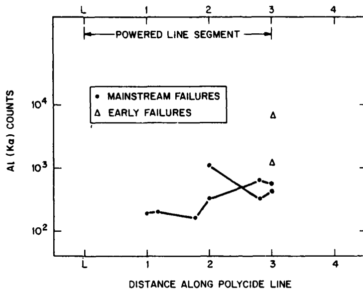
Figure 38. Al ( K\alpha ) EPM x-ray counts versus distance along polycide line for CRTV mode-2 mainstream failures and early failures in which the Al (or Al-Si) film had been stripped.
