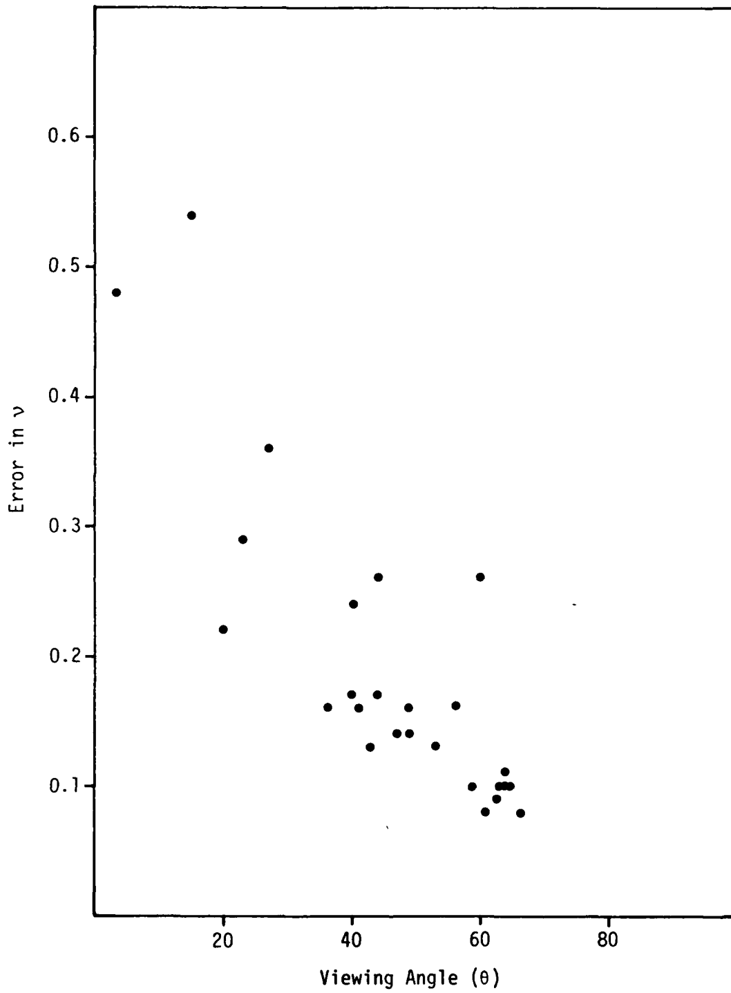
Figure 4. Variation of Error in v , Due to Channel 2 Error, With Viewing Angle (From Table 1).
