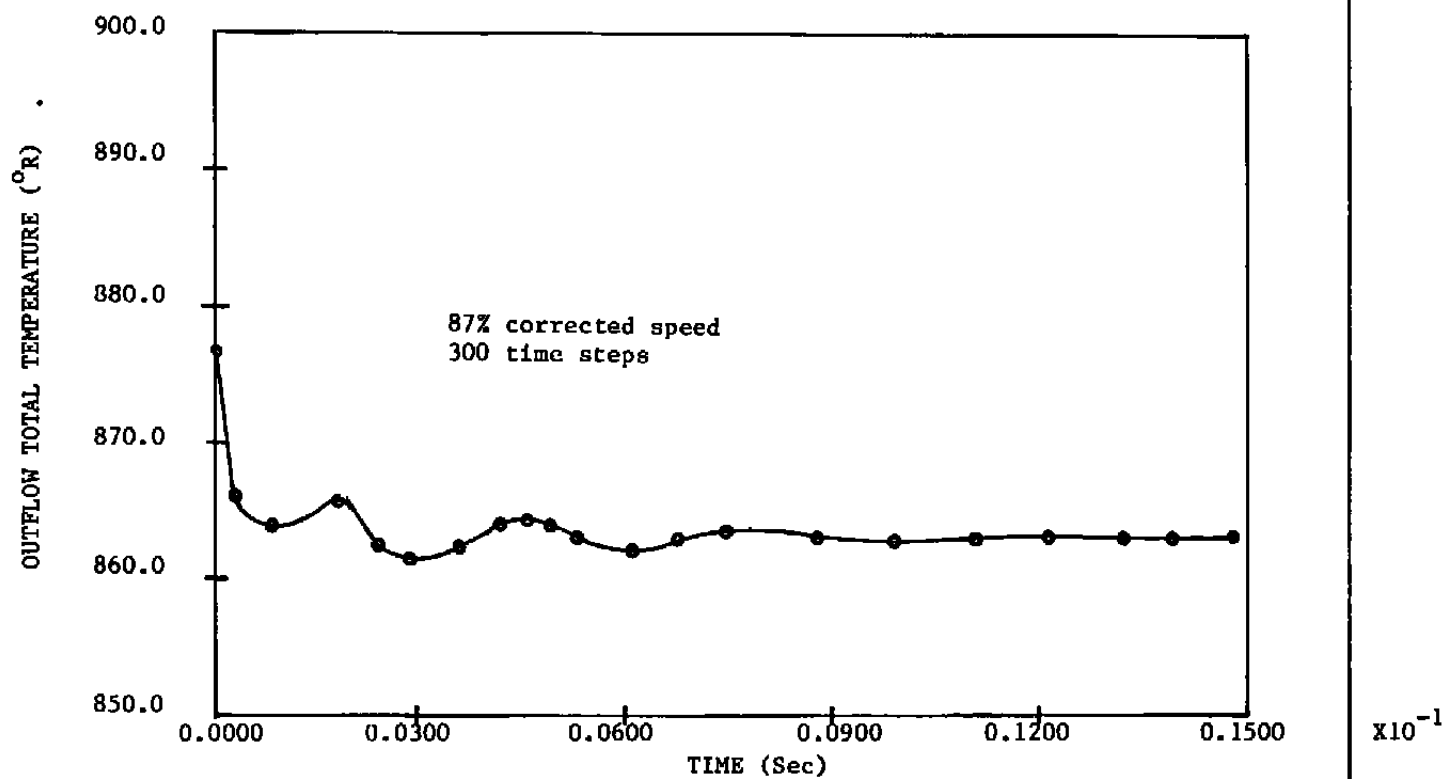
Figure 9. Outflow total temperature versus time with changes 1, 2, and 3 (COMP2SP).
