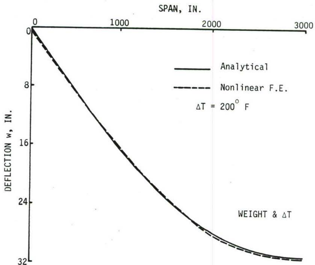
Fig. 15 Comparative deflections for cable loaded by its own weight and subjected to a temperature rise.
