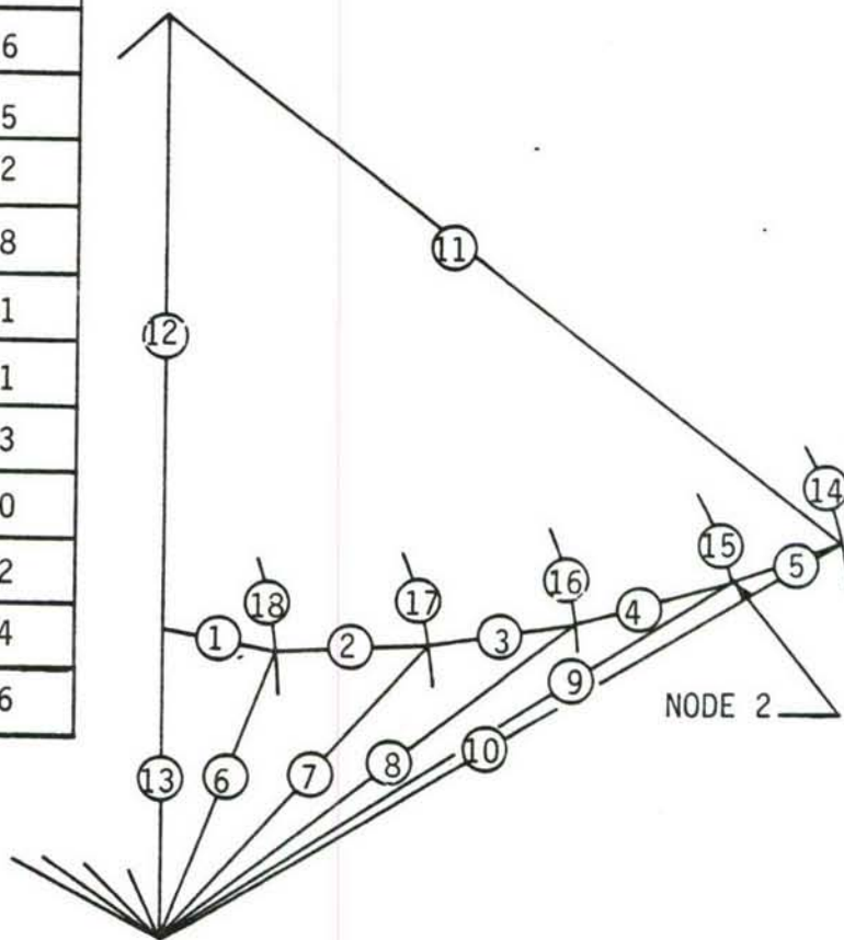
Fig. 28 Member prestresses for prestressed hoop column antenna.
