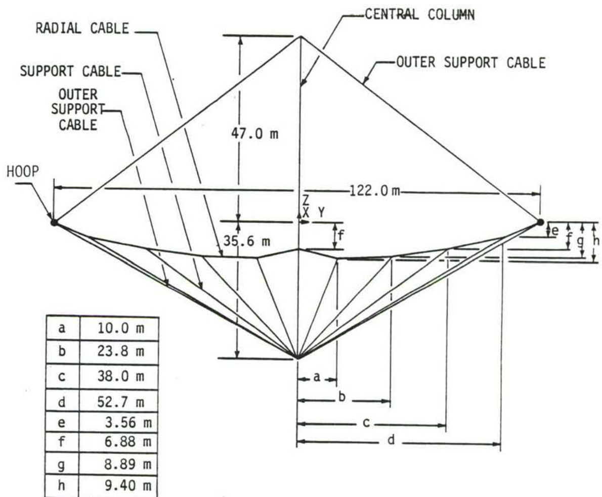
Fig. 25 Front section of the hoop column antenna.
