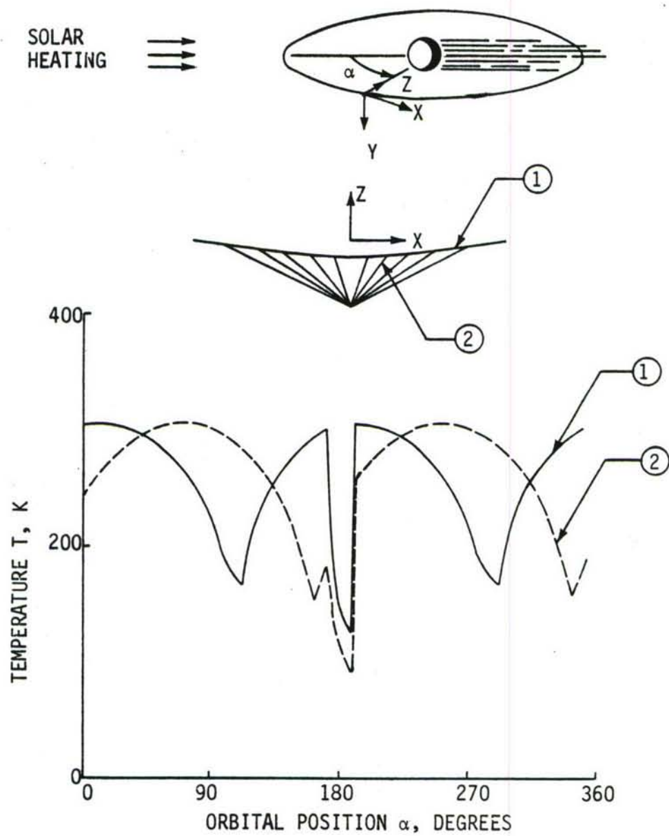
Fig. 19 Temperature histories of typical members of simplified pretensioned cable system.
