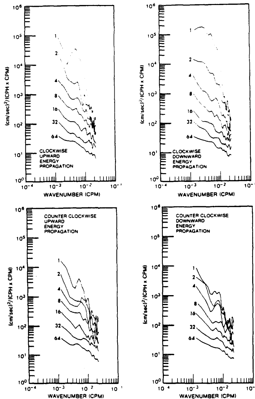
FIG. 15. Cross sections of the clockwise and counterclockwise wavenumber-frequency spectra. Sections are taken at frequencies of 1, 2, 4, 8, 16, 32 and 64 cpd. Averaging across frequency is done to improve the statistical stability of the sections. The spectral estimates are formed at 20, 36, 68, 132, 260, 516 and 1028 degrees of freedom.
