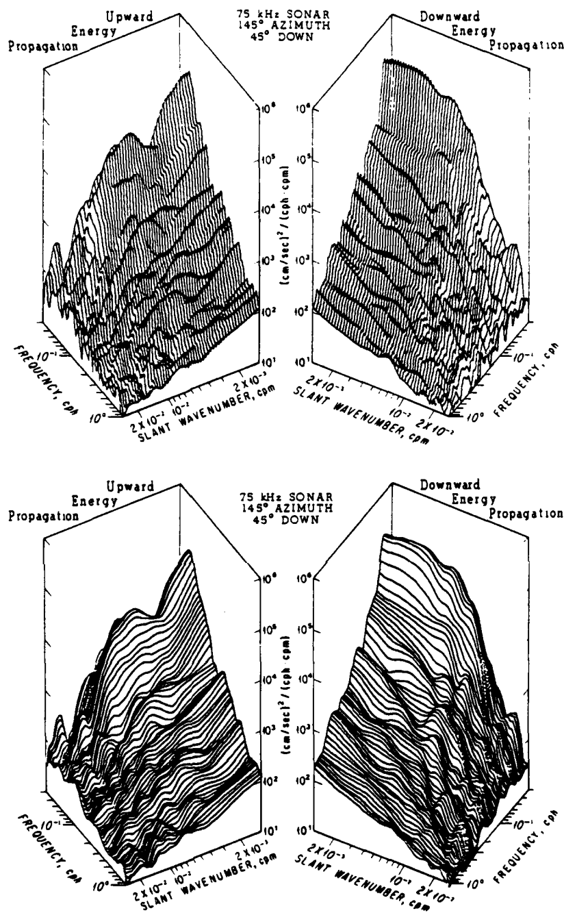
FIG. 3. As in Fig. 2 but from the 75 kHz sonar (direction 145°).
