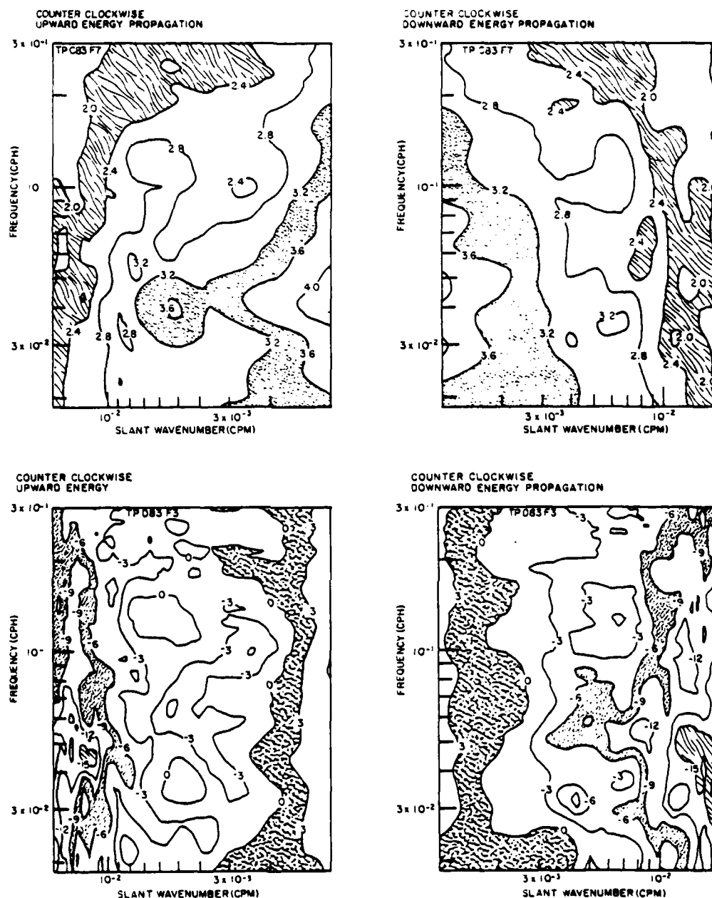
FIG. 14. As in Fig. 13 except for a counterclockwise sense of rotation. Note that neither the upward nor downward spectral estimate exhibits a significant change in bandwidth with frequencies.
