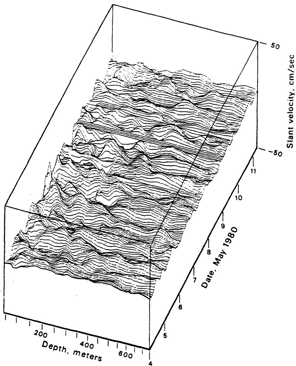
70 kHz VELOCITY PROFILE: 7 DAY RECORD
