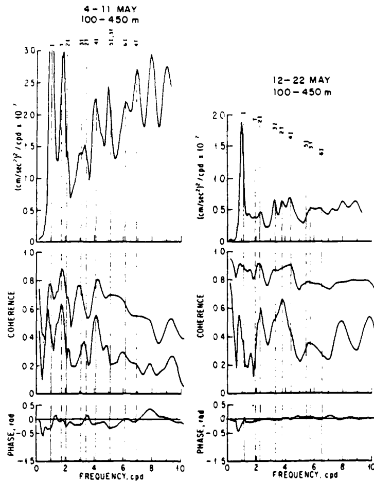
FIG. 9. Depth-averaged clockwise slant-acceleration spectra, slant coherence and phase, 100–450 m average. The power spectra are identical to those in Fig. 8, except plotted on linear scales. Note that the large inertial peak in the 4–11 May data has been truncated. It actually reaches a value of 9 \times 10^{-4} (cm/s 2 ) 1/2 /cpd. Coherences are plotted for slant separations of 20 and 40 m in the 4–11 May data, 15 and 45 m for the 12–22 May data. Coherence values at the smaller of these separations are slightly overestimated. This results from the finite length of the acoustic pulse, which averages over 30–40 m in space.
