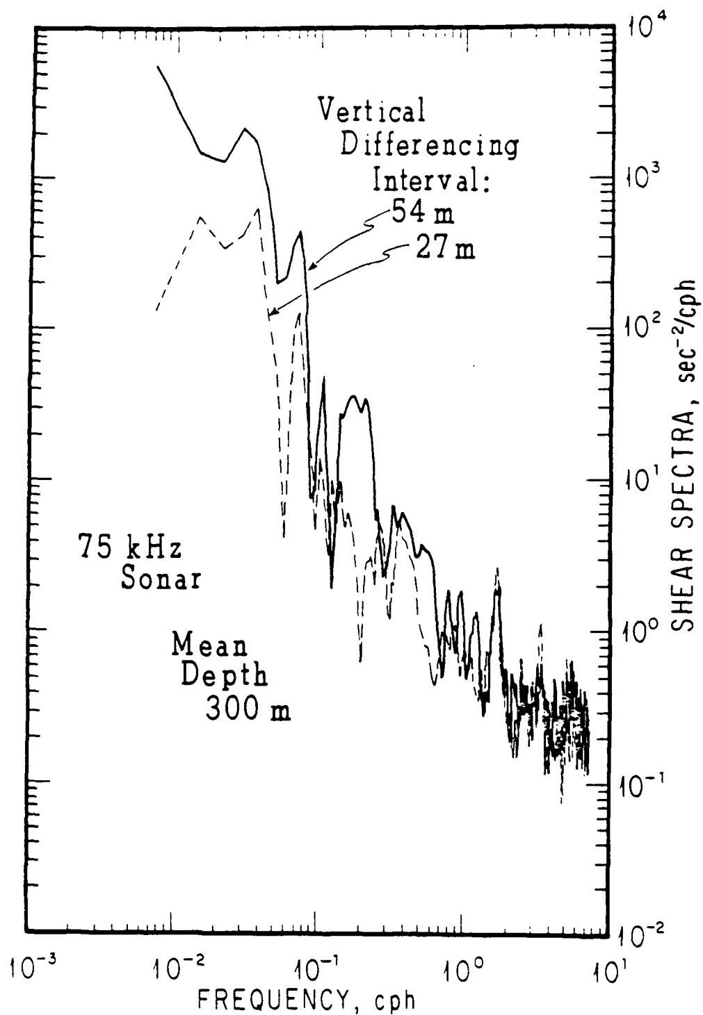
Fig. 4. Spectra of velocity shear obtained by differencing the Doppler velocity range-time series (Fig. 2) with respect to range. Spectra are presented for a depth centered at 300 m with differencing intervals 27 m and 54 m. The low frequency form of the spectrum with 54 m separation is very nearly \omega^{-2} . With the smaller separation the slope is more gradual. The spectra fall into the noise at approximately 2 cph.
