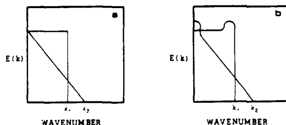
FIG. 10. (a) Spectral cross sections of two hypothetical wavenumber-frequency spectra. The cross sections are associated with nearly identical values of coherence over small separations \Delta z . (b) Slightly perturbed variants of these spectral forms having only slightly different coherence. Yet, qualitatively, one would not be inclined to say that they have the same bandwidth. While coherence is an appropriate way to quantify spectral bandwidth, it is not very sensitive.
