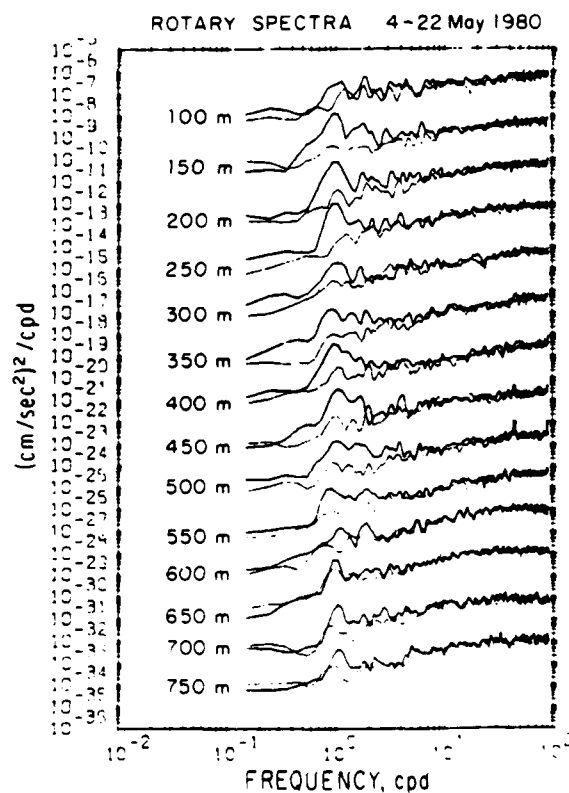
FIG. 7. Rotary slant-acceleration spectra. The clockwise spectra are indicated by the heavy line. The same smoothing is employed as in Fig. 6.
