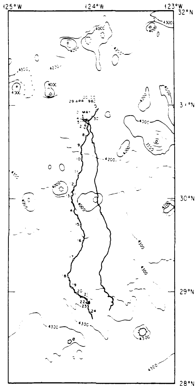
FIG. 3. A map of FLIP's drift. The left-most line represents the time series of FLIP's position as determined by Loran C. Numbered circles indicate the date. The right track is the progressive vector formed by time-integrating the 200–550 m depth-averaged Doppler velocities sensed by the sonars.
