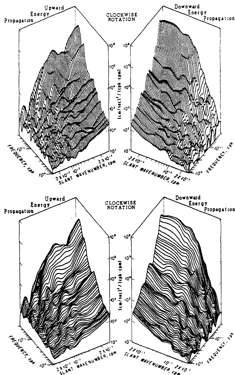
FIG. 11. Clockwise rotary wavenumber-frequency spectral estimates obtained from combining 70 and 75 kHz sonar information. The upper spectrum has been logarithmically averaged in both wavenumber and frequency. The lower spectrum has been additionally smoothed in frequency to suppress the series of ridges that parallels the wavenumber axis.
