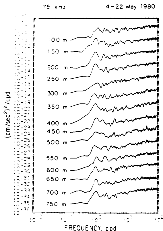
FIG. 6. Slant acceleration spectra from the 75 kHz sonar. The sonar was pointed in the direction 145°T. The spectra are estimated at approximately 8 degrees of freedom to 2.5 cpd, 24 degrees of freedom to 5 cpd. Above 5 cpd the spectral averaging is progressively increased, reaching approximately 1200 degrees of freedom between 10 and 100 cpd. The averaging was achieved by low-pass filtering the spectral estimate. Adjacent spectral points are not independent.
