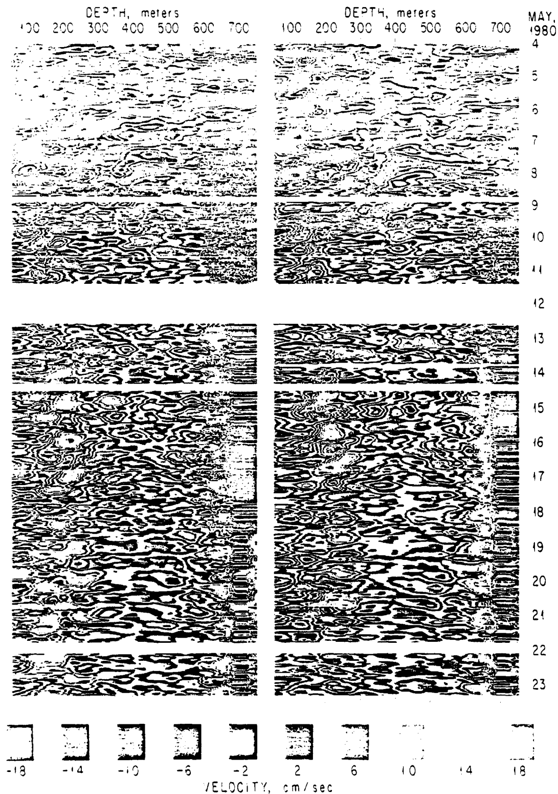
FIG. 4. A contour map of the observed velocity field. The 70 kHz (left) and 75 kHz (right) sonar velocities are positive toward 55°T and 325°T, respectively. In this plot the mean velocity in the layer 200–550 m has been removed, to minimize the effects of FLIP's drift. Gaps in the data are indicated by the horizontal white bands. The very fine scale structure at great range is instrument noise.
