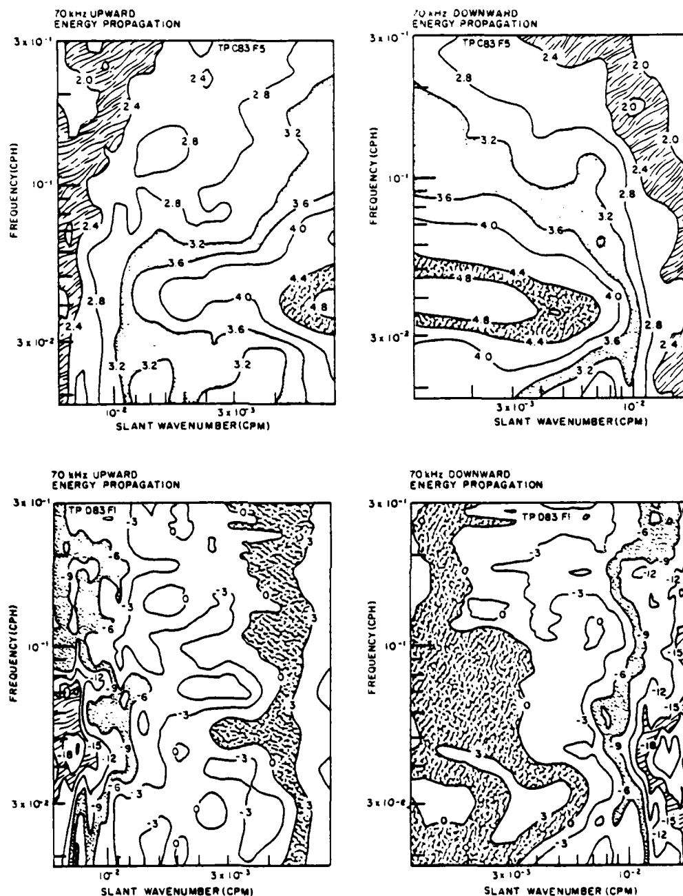
FIG. 4. Contour maps of the frequency-smoothed log-log averaged spectrum from the 70 kHz sonar. The upper maps represent the estimate of the slant velocity spectrum, (\text{cm s}^{-1})^2/(\text{cpm} \cdot \text{cph}) , contoured at logarithmic intervals. The lower maps give the spectral estimate normalized such that
