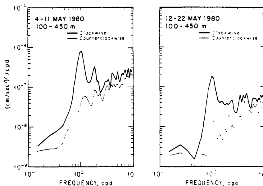
FIG. 8. Depth-averaged rotary slant-acceleration spectra, 4-11 May and 12-22 May 1980. Eight spectra, at 50 m intervals between 100 and 450 m, are combined to form each spectral estimate. There are nominally 64 degrees of freedom below 2.5 cpd, 192 degrees of freedom below 5 cpd. The actual statistical stability of this estimate is less than indicated by the number of degrees of freedom, as adjacent depths are not statistically independent. The clockwise spectra are indicated by the heavy lines.
