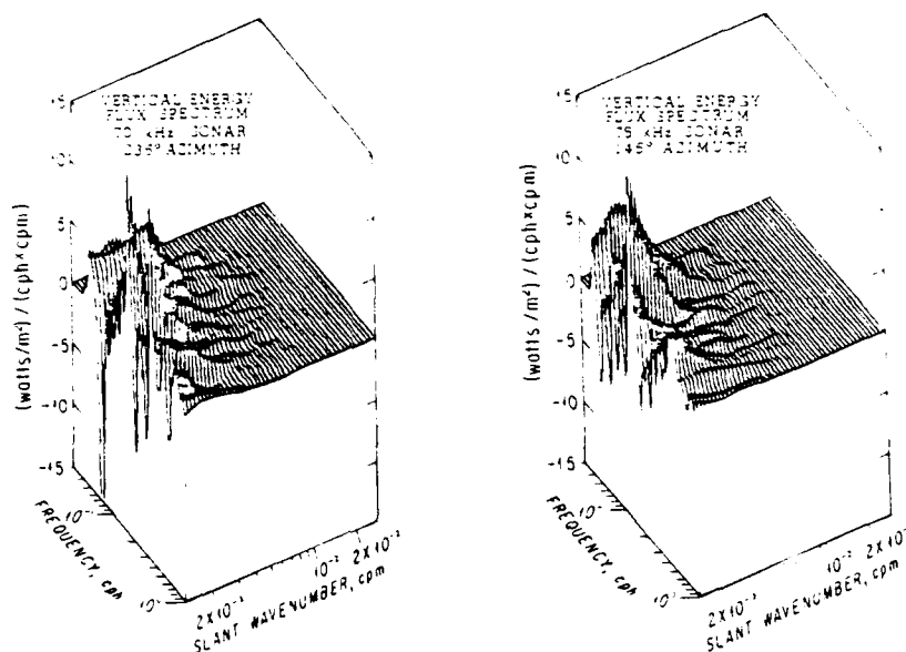
FIG. 8. Deformed surface plots of energy flux spectrum F(k, \omega) for the 70 and 75 kHz sonars. The spectra are log-log averaged, and presented so as to preserve the visibility of the spectral ridges. Positive spectral values correspond to a downward energy flux. The 70 kHz spectrum has been truncated in the semidiurnal tidal band. The upward-flux spectrum peaks at approximately -25 \text{ W m}^{-2} (\text{cph} \cdot \text{cpm})^{-1} in this band. The upward-flux contribution from the higher-frequency waves, which dominates the net wavefield flux, is obscured by all of the detail in this figure.
