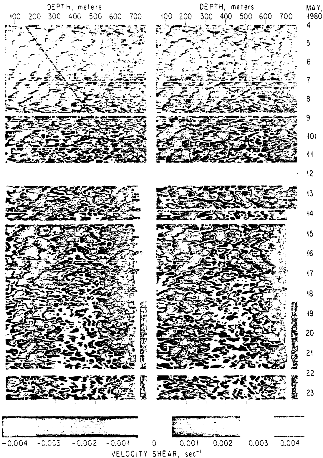
FIG. 5. A contour map of the observed shear field using the 70 and 75 kHz sonars as in Fig. 4. Positive shear implies velocity increasing toward 55°T (325°T) with increasing depth. The broken line on the 70 kHz plot indicates the downward expansion of a near-inertial group which dominates the shear field during the early part of the cruise.
