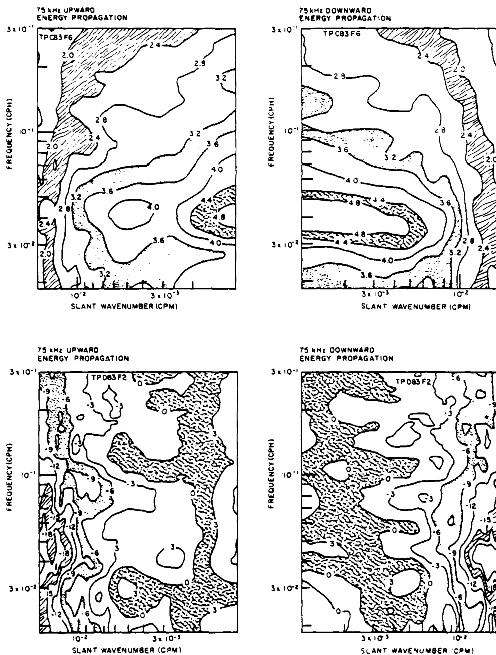
FIG. 5. As in Fig. 4 but from the 75 kHz sonar.
