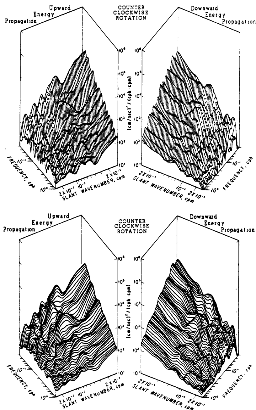
FIG. 12. As in Fig. 11 but for a counterclockwise sense of rotation.
