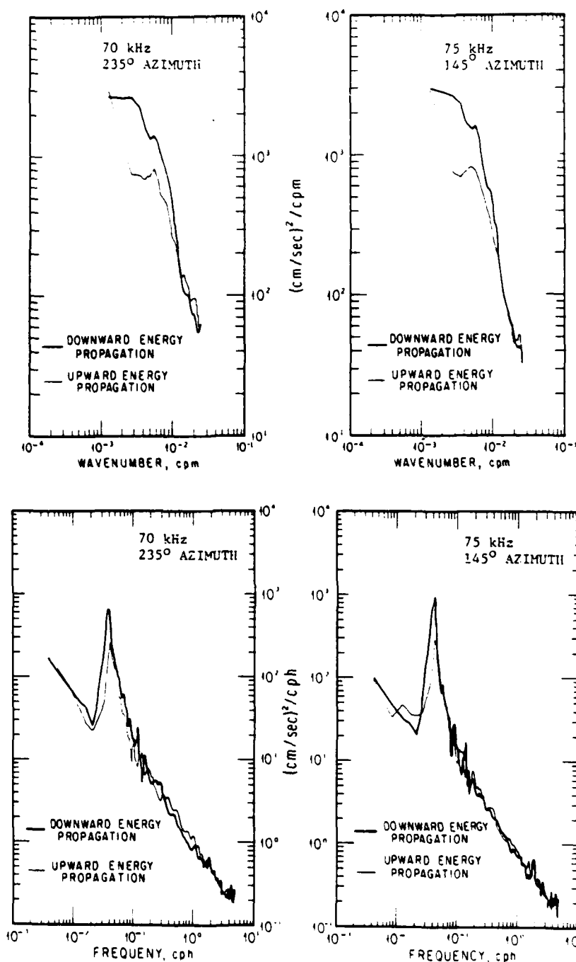
FIG. 7. Estimates of the wavenumber-frequency spectrum integrated in frequency, to produce a slant wavenumber spectrum (top), and in wavenumber, to produce a frequency spectrum (bottom). The dark line corresponds to the integrated downward spectrum, the light line to the upward. For comparison with conventional profiling measurements (top), or moored time series measurements (bottom), the upward and downward contributions should be summed. Note that the low-frequency, high-wavenumber cutoff, visible in Figs. 2, 3 and 6 is largely obscured when the spectrum is integrated over frequency (top). Also, the upward frequency spectra (bottom) tend to have more variance than the downward over a broad band of high frequencies. As these motions have a greater vertical group velocity than the more energetic near-inertial motions, they are the predominant contributors to the net upward energy flux of the wavefield.
