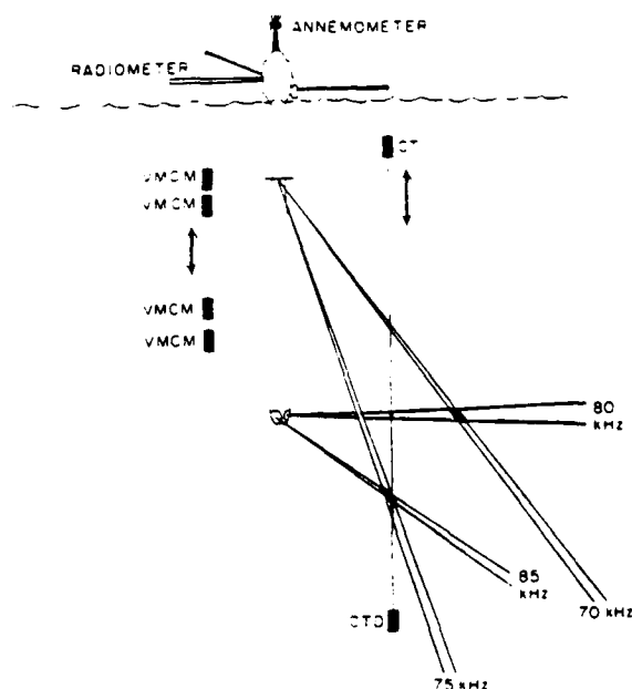
FIG. 1. Schematic diagram of the 1980 FLIP experiment. Sonar and profiling-CTD locations are indicated. The profiling current meter (VMCM) array was developed and operated by R. Weller. An array of surface-wave staffs is not shown in the figure.
