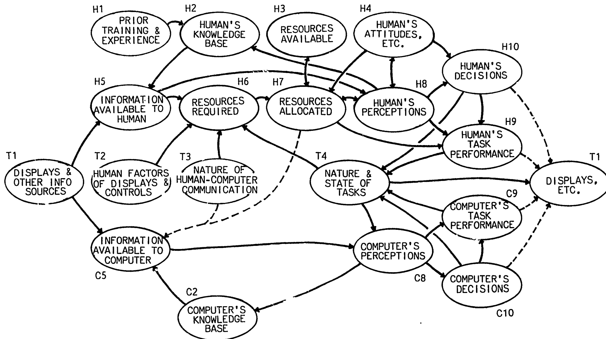
Figure 4. Model of human-computer interaction.
