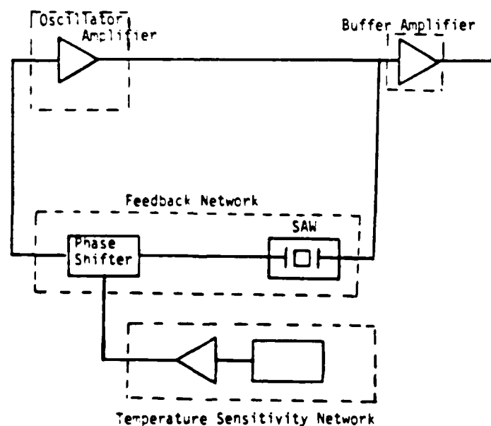
Fig. 2 Temperature compensated SAW resonator.
