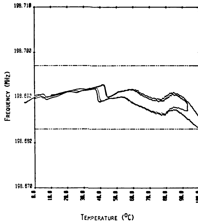
Fig. 3 Frequency deviation as a function of temperature.
