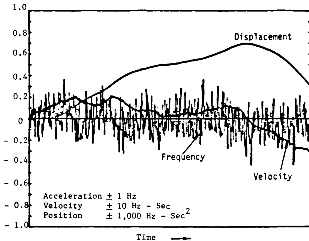
Fig. 5 Measured count output of SAW dual crystal sensor vs time. Total time was approximately 3 min with a 10 ms gate time. Also shown is the computed velocity from integrating once as well as the displacement as a result of integrating the counter output twice.
