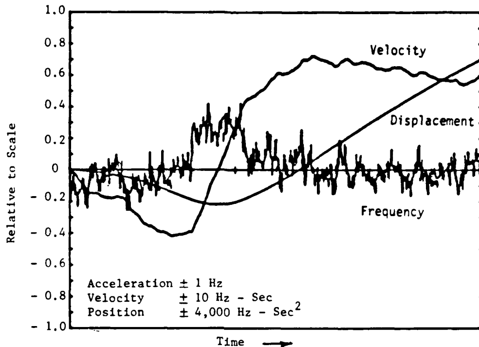
Fig. 4 Measured count output of a SAW dual crystal sensor vs time. Total time was approximately 18 min with a 2 s gate time. Also shown is the computed velocity from integrating once as well as the displacement as a result of integrating the counter output twice.
