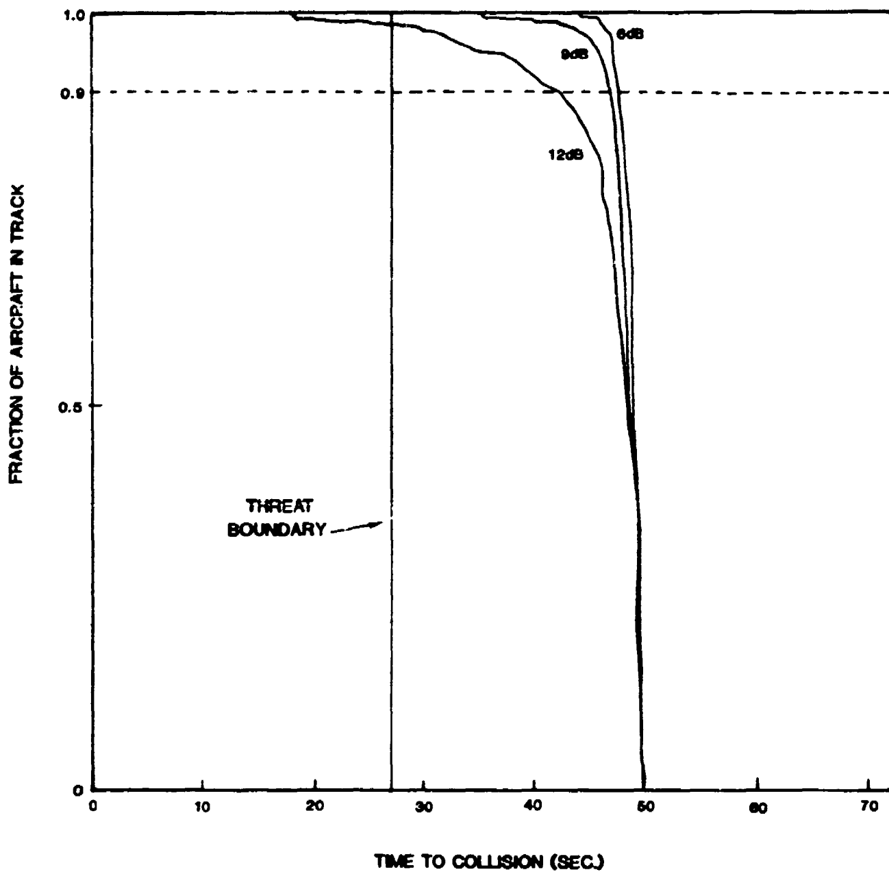
Fig. 4-11. Low altitude collision protection for normal operation with MTL's of 6, 9, and 12dB.
