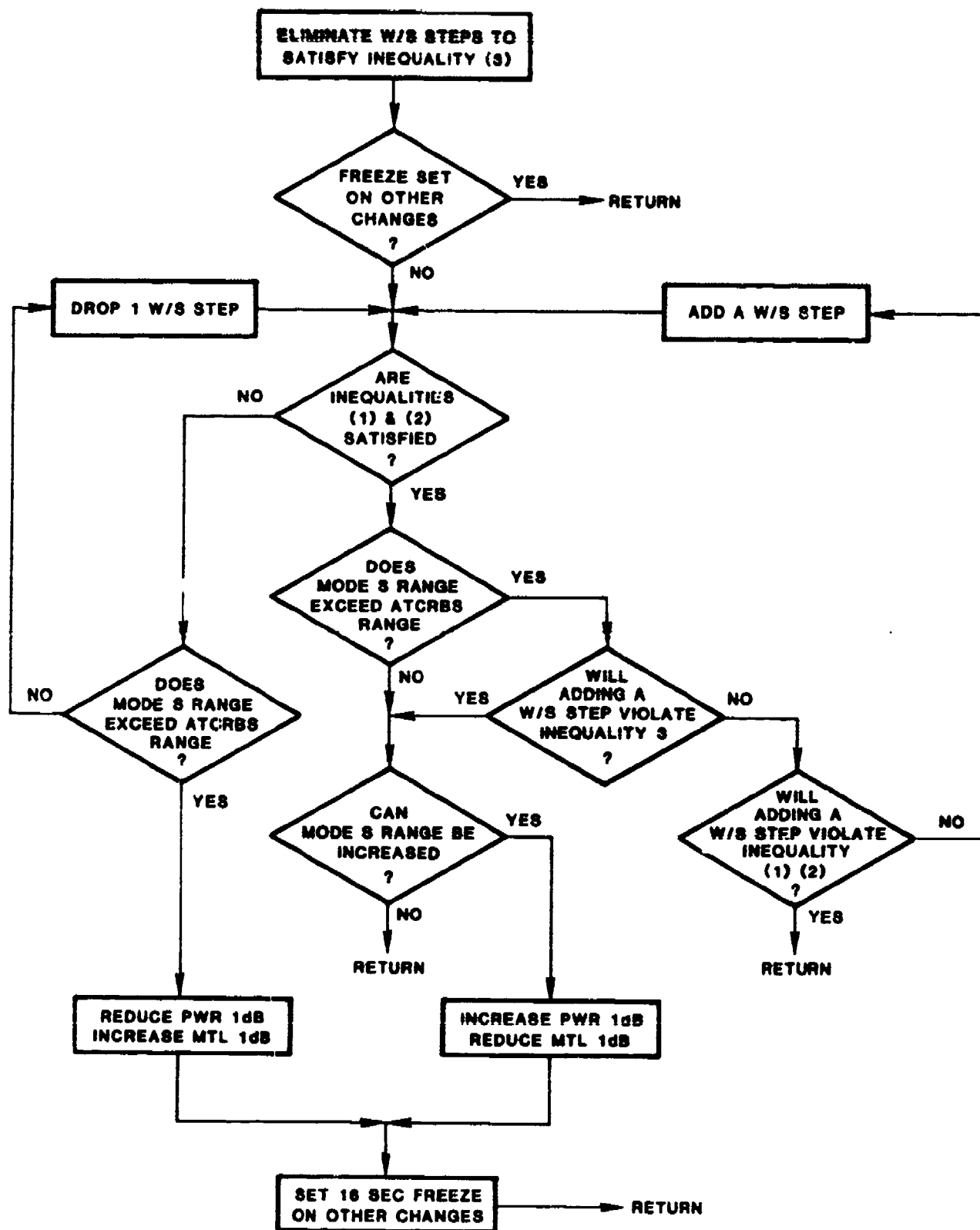
Fig. 5-3, Interrogation limiting flow diagram.
