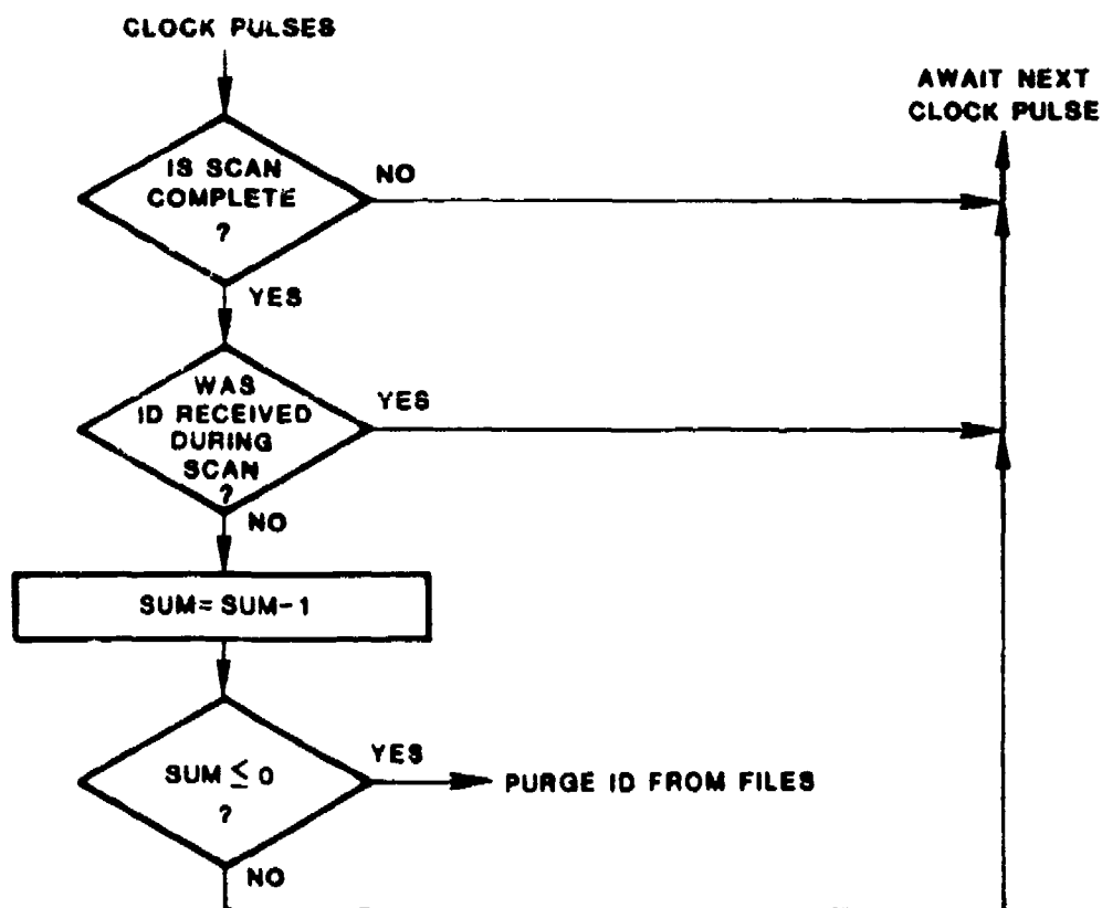
Fig.4-3. Monitor state processing algorithms.
