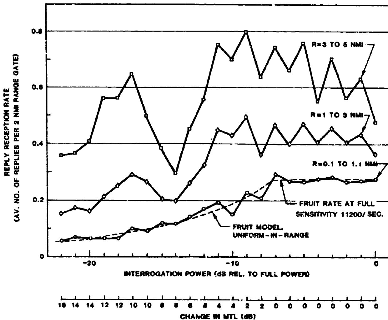
Fig. 3-24. Whisper-shout profiles for omnidirectional interrogator.
