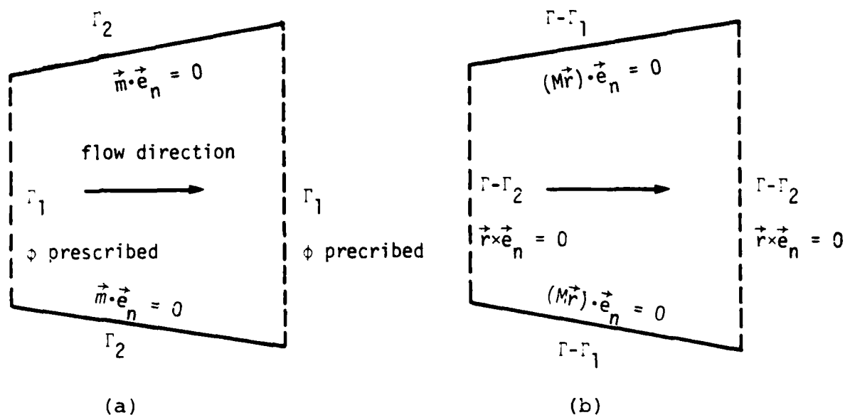
Figure 5. Subsonic Problem: (a) Physical Boundary Value Problem. (b) Boundary Value Problem for the Residual \vec{r} .
