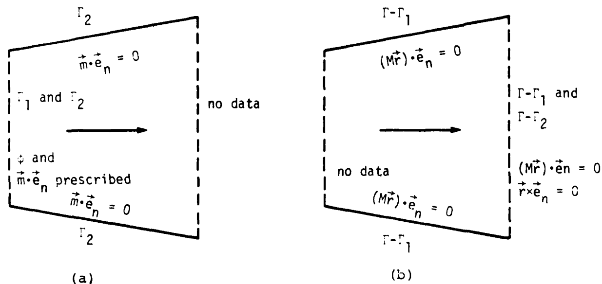
Figure 6. Supersonic Flow: (a) Physical Boundary Value Problem. (b) Boundary Value Problem for the Residual \vec{r} .
