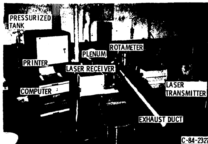
Figure 2. - Test facility.
