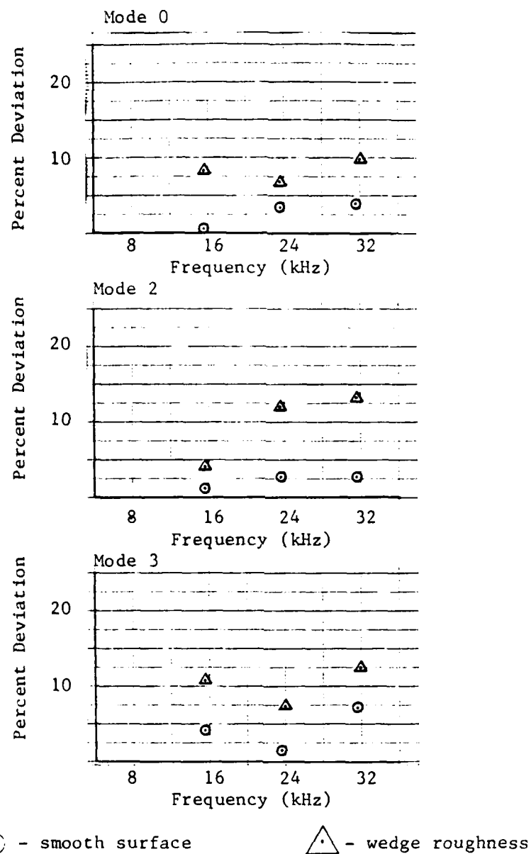
Figure 14b. Standard Deviation of Percent Energy in Modes Adjacent to Mode 1 (Mode 1 Driven).
