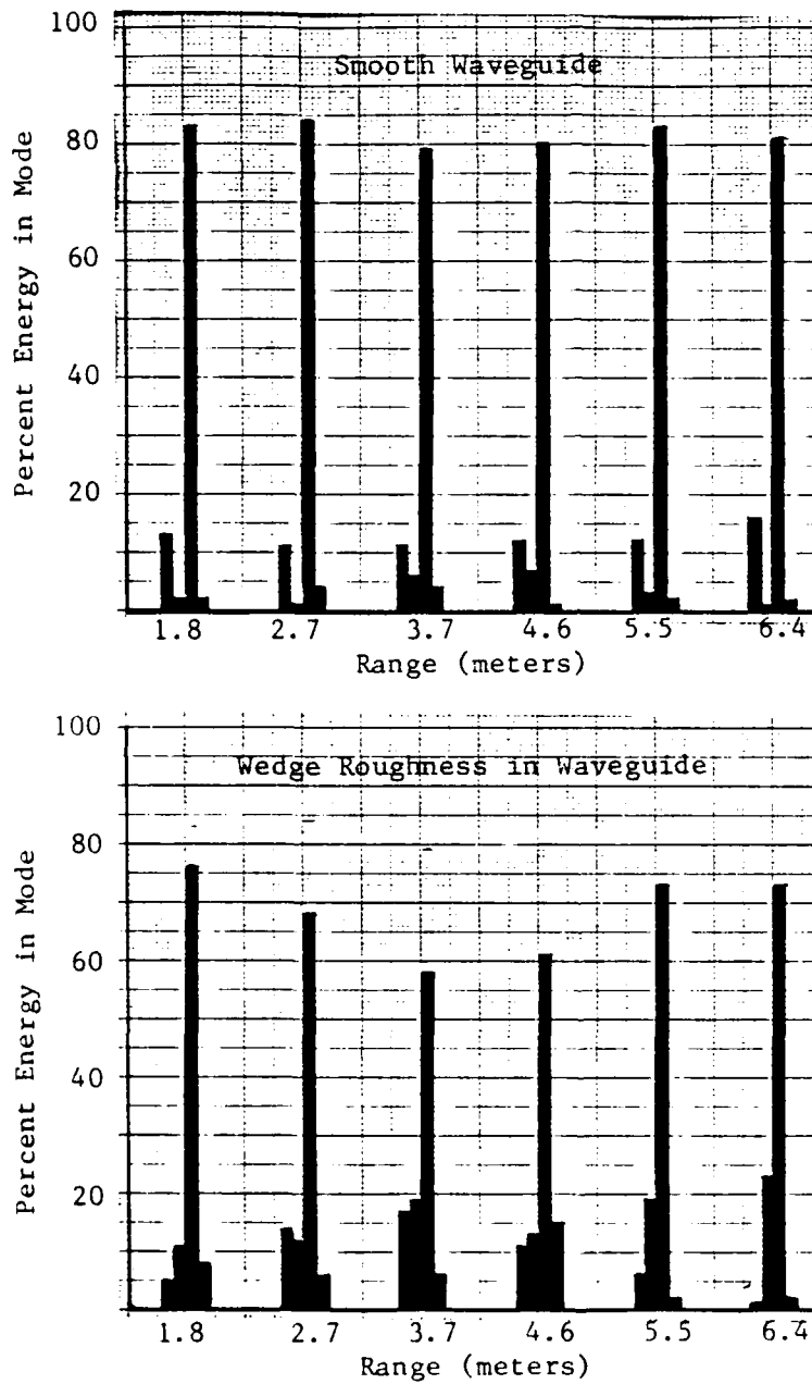
Figure 16b. Energy Distribution vs. Range at 15750 Hz, Mode 2 Driven
