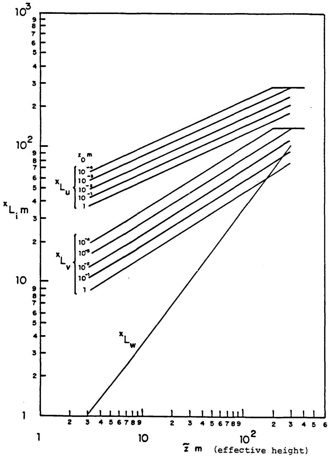
Figure 4.12 Values of Length Scale Parameter L_i (Reproduced from ESDU 74031).
