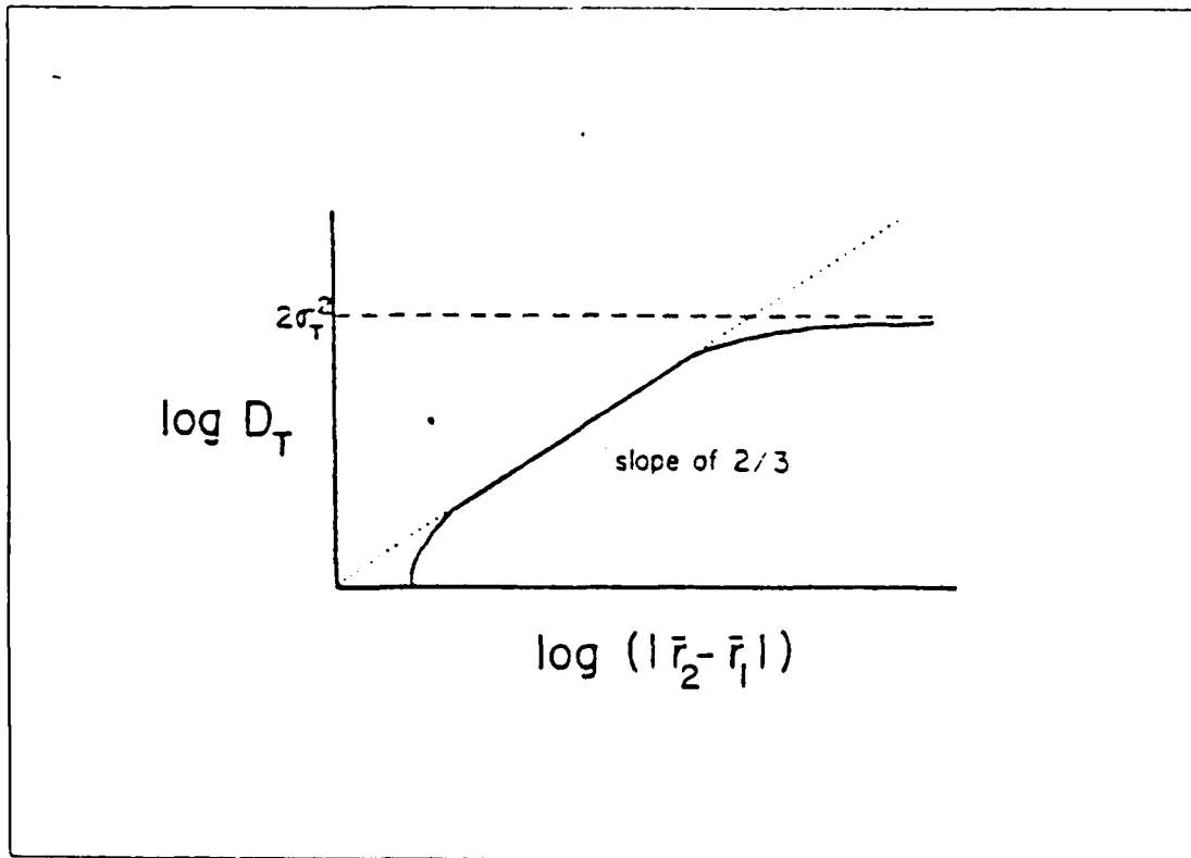
Figure 2.1 \log D_T vs \log(|r_2 - r_1|) .
