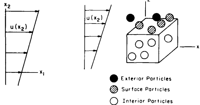
Figure 2. A control volume in a granular flow of uniform spheres.
