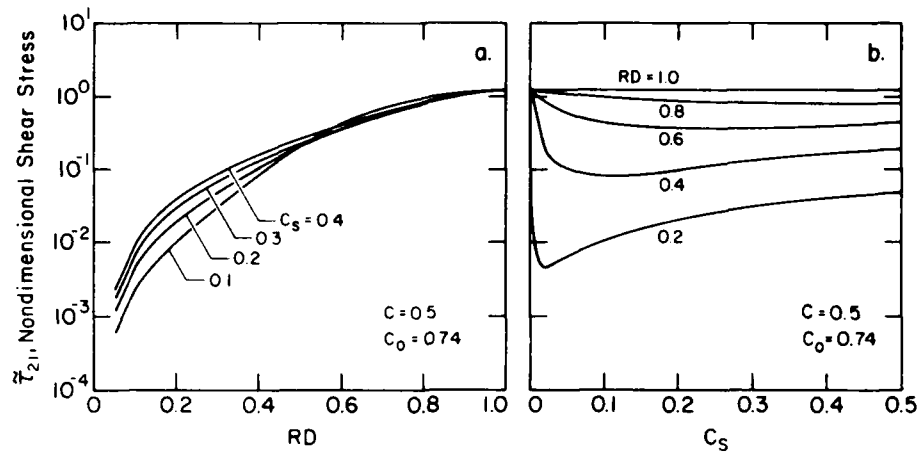
Figure 5. Particle size effect on shear stress.
