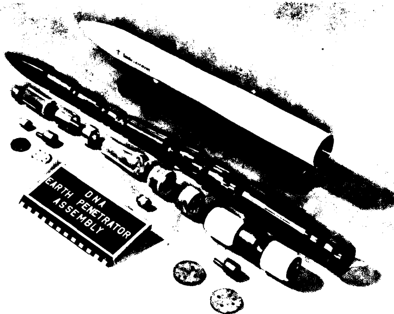
Figure 2. Case and internal components of an EP assembly
