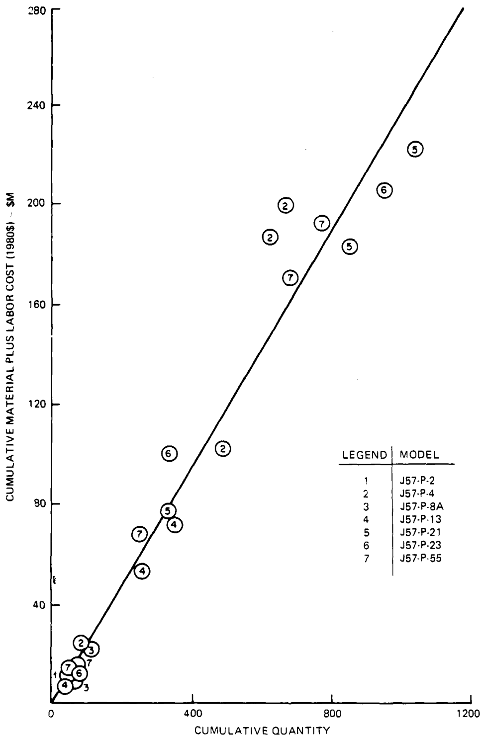
Figure 11. Cumulative Cost vs. Quantity. First Year Large Buy, Afterburning Engines
