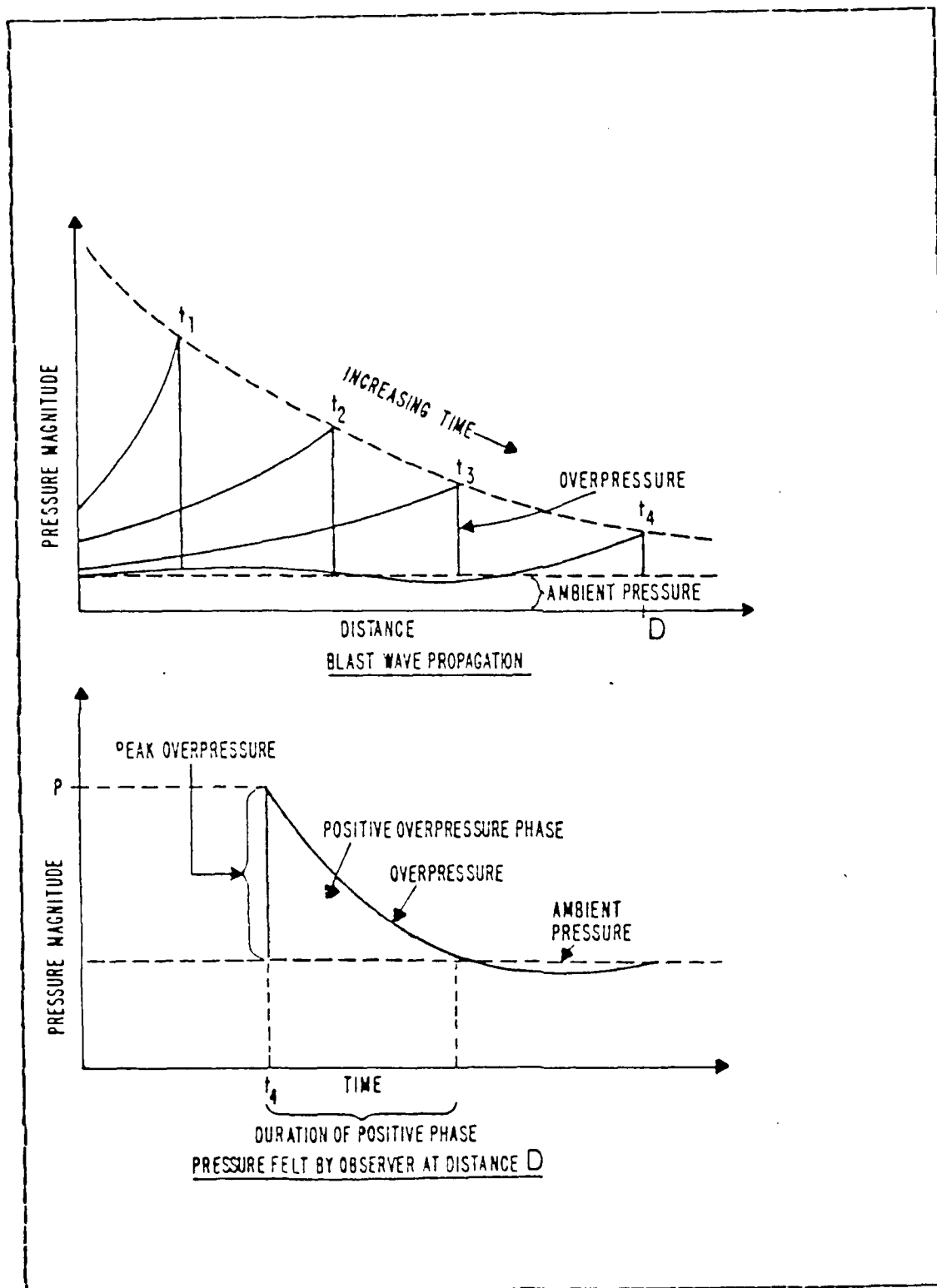
Figure 3.3 Typical Pressure Wave
