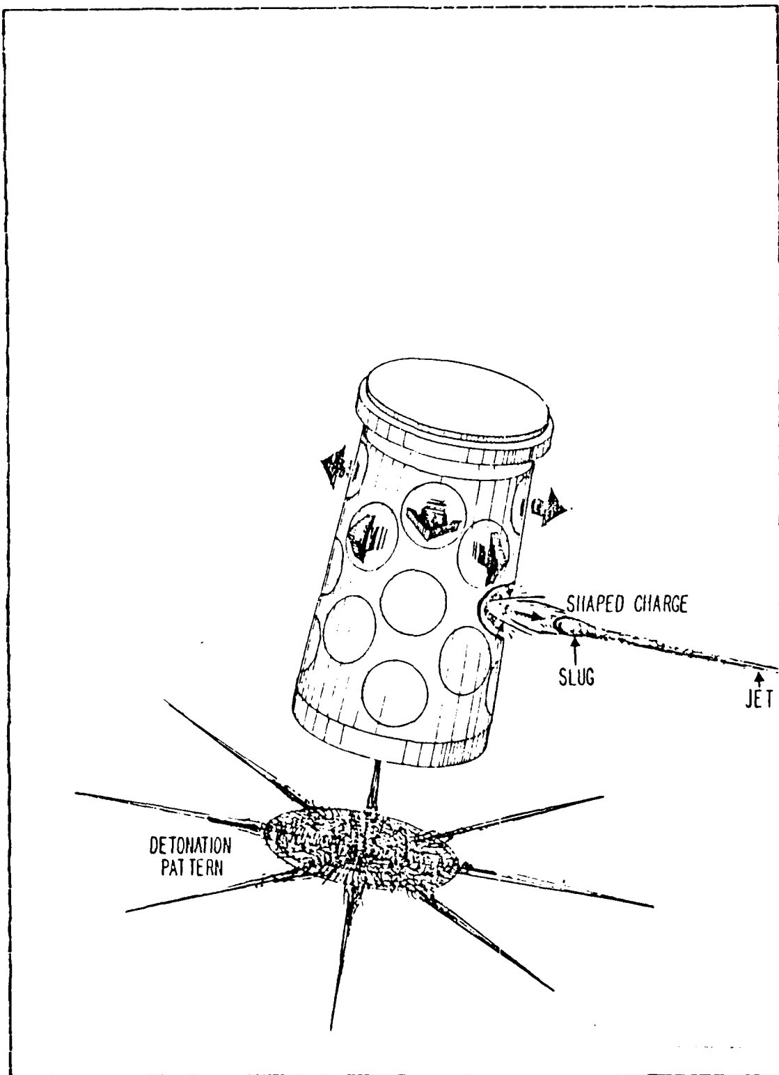
Figure 3.7 Typical Shaped Charge Warhead
