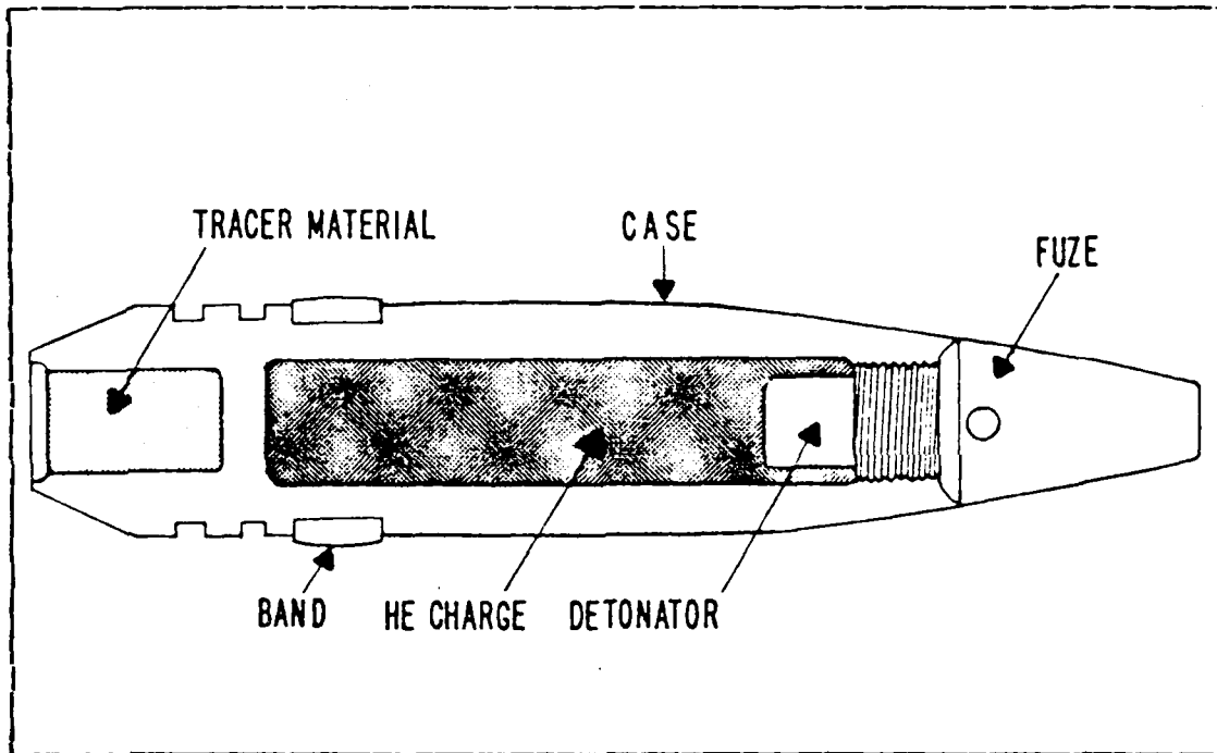
Figure 1.7 HE-T Projectile
