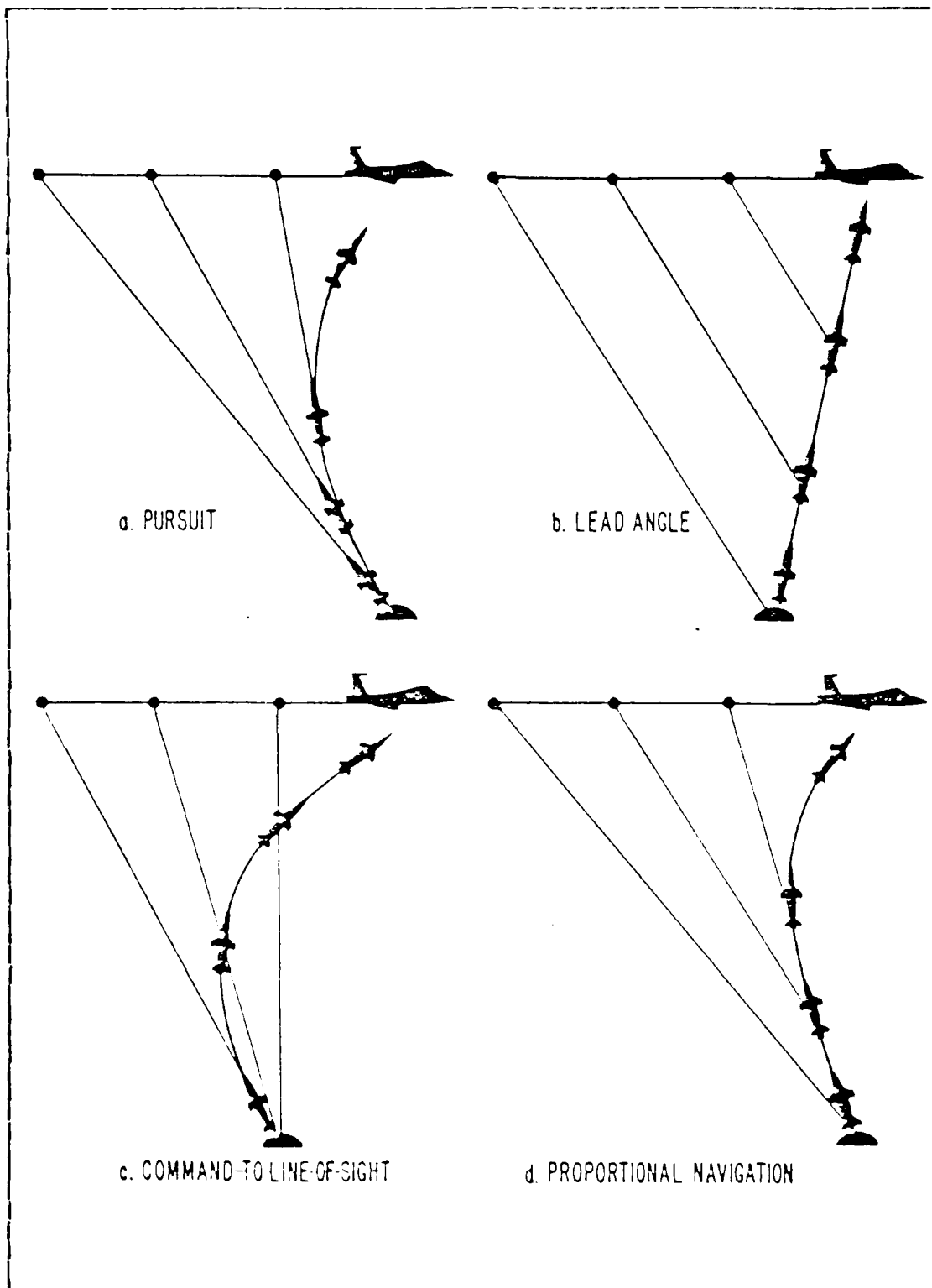
Figure 2.9 Missile Trajectories
