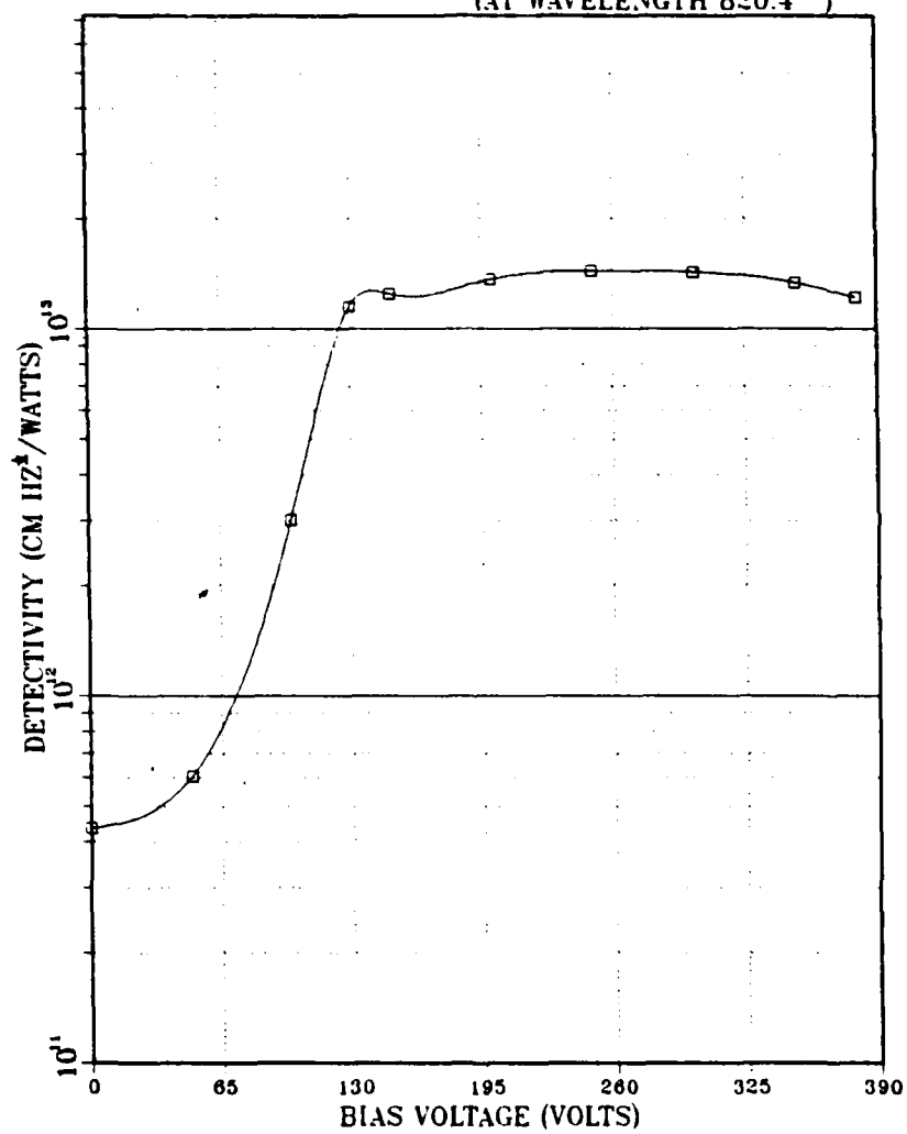
Figure 4.8 Detectivity versus Bias Voltage.
