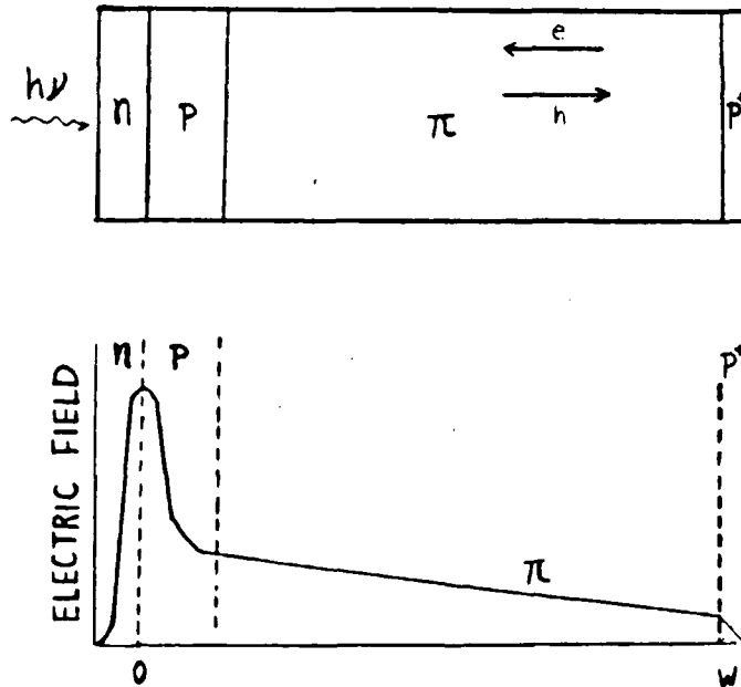
Figure 2.1 Standard RAPD Structure.
