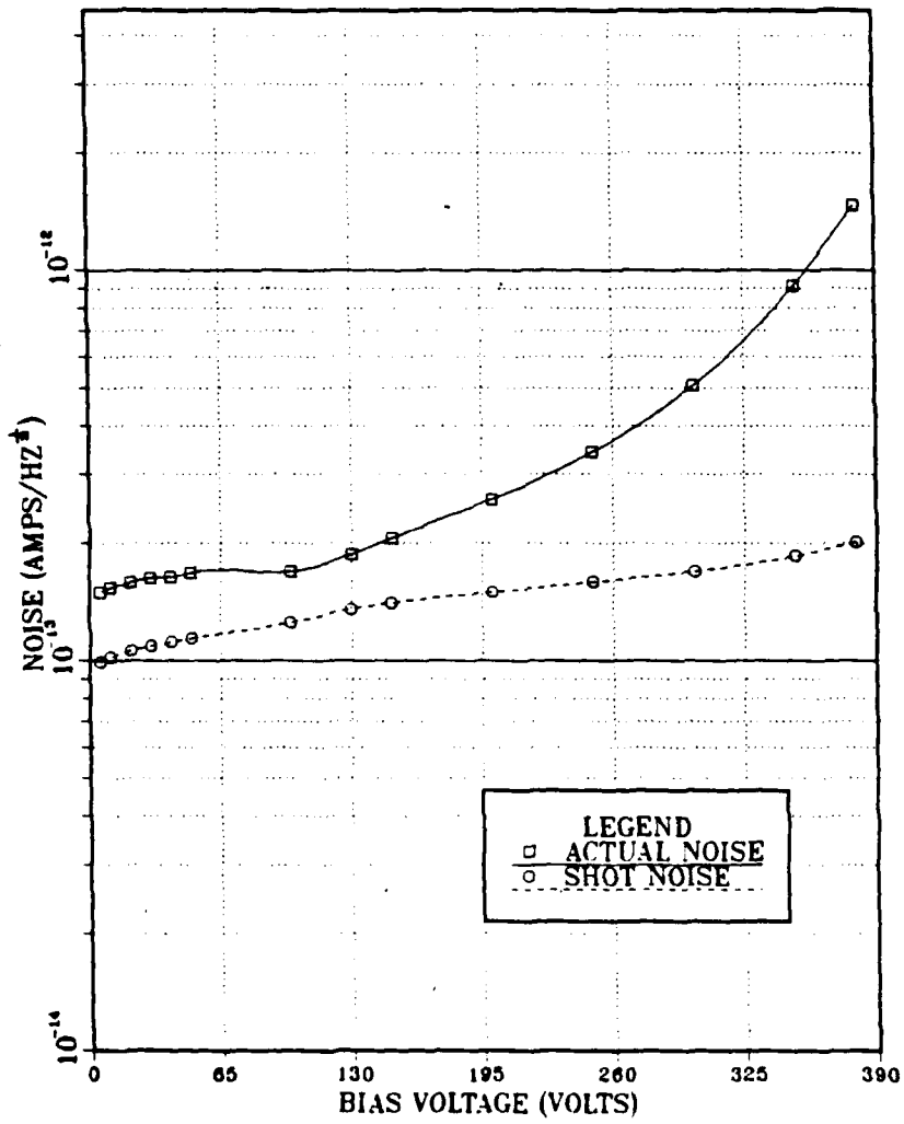
Figure 4.2 Noise versus Bias Voltage.
