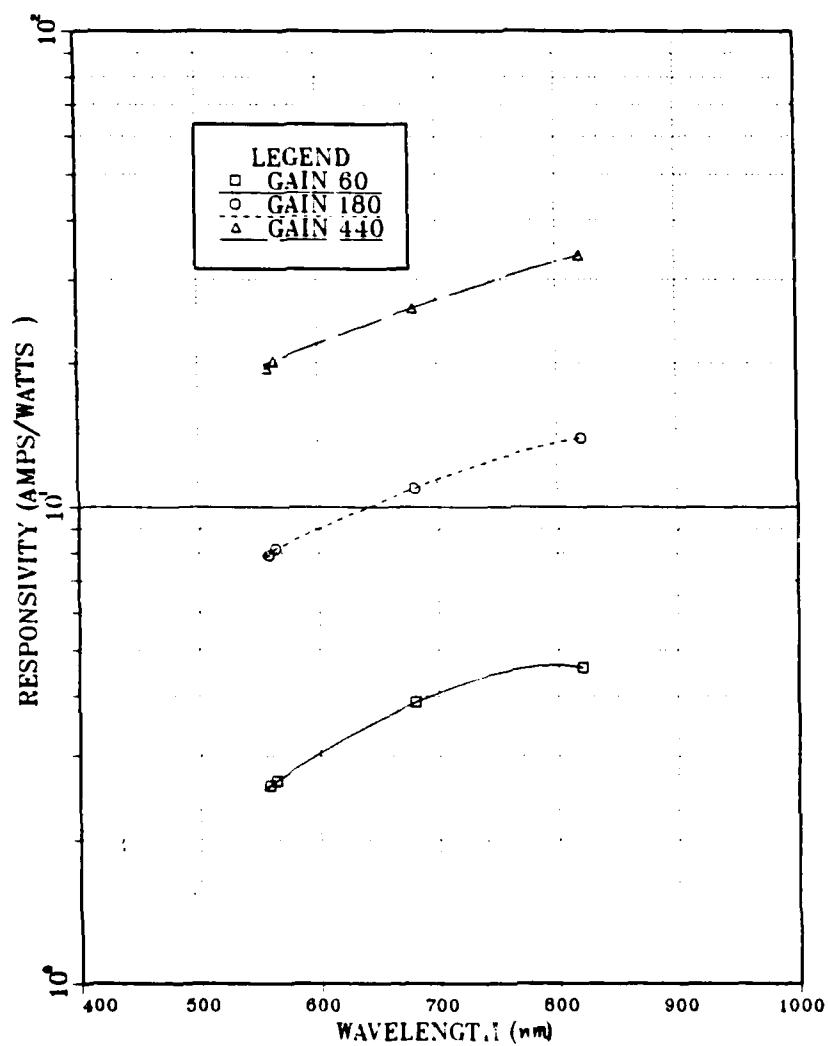
Figure 4.6 Responsivity versus Wavelength.
