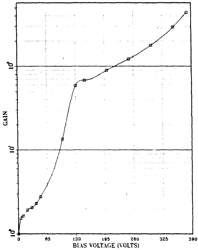
Figure 4.3 Gain versus Bias Voltage.
