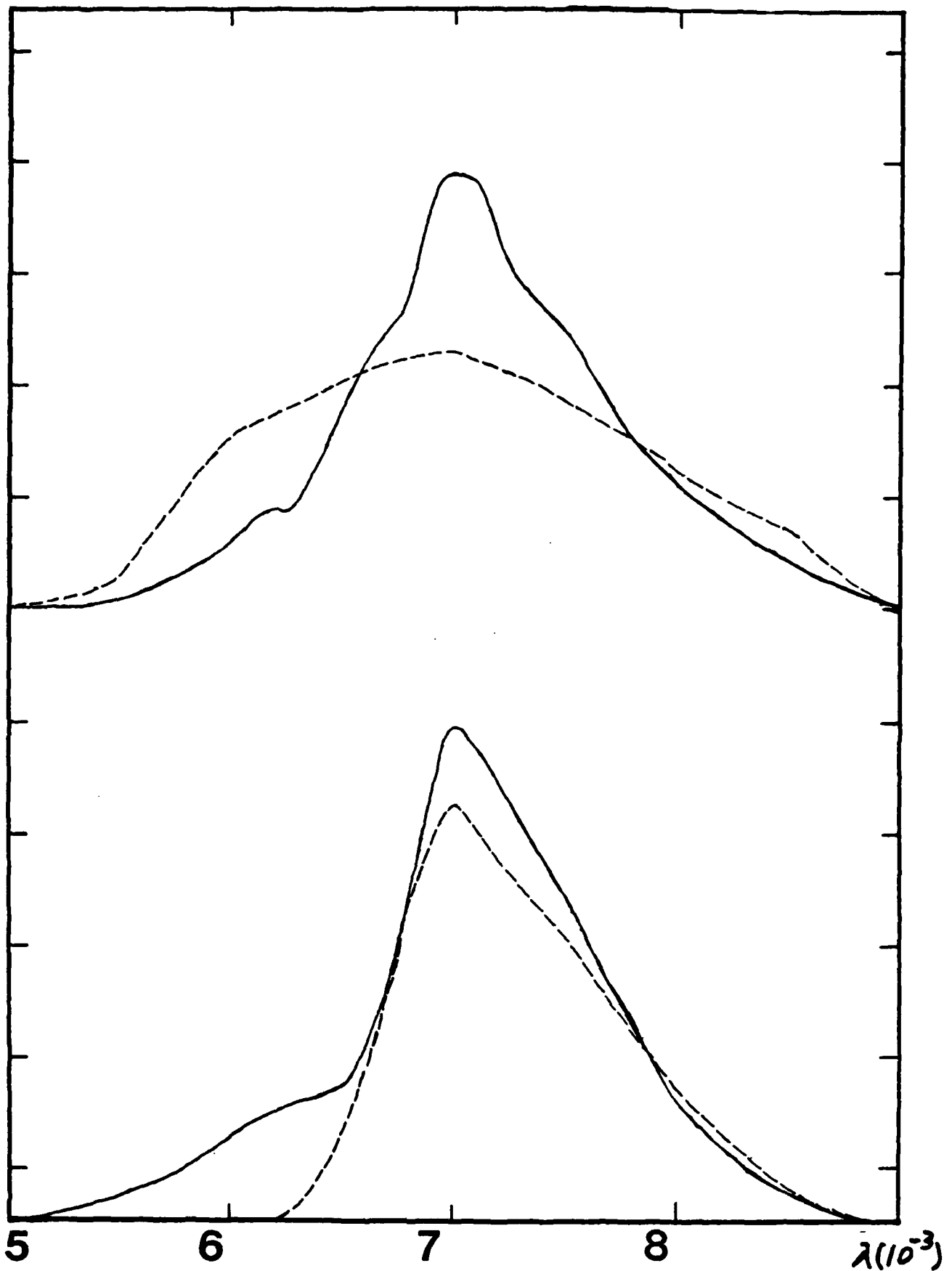
Fig. 3 Fluorescence spectra of \text{Rh}^{2+} in \text{Na } \beta''\text{-alumina} . TOP: T=10 K; solid line for 25 ps after excitation pulse; broken line for 200 ps after excitation pulse. BOTTOM: T=300 K; broken line for 25 \mu s after excitation pulse; solid line for
