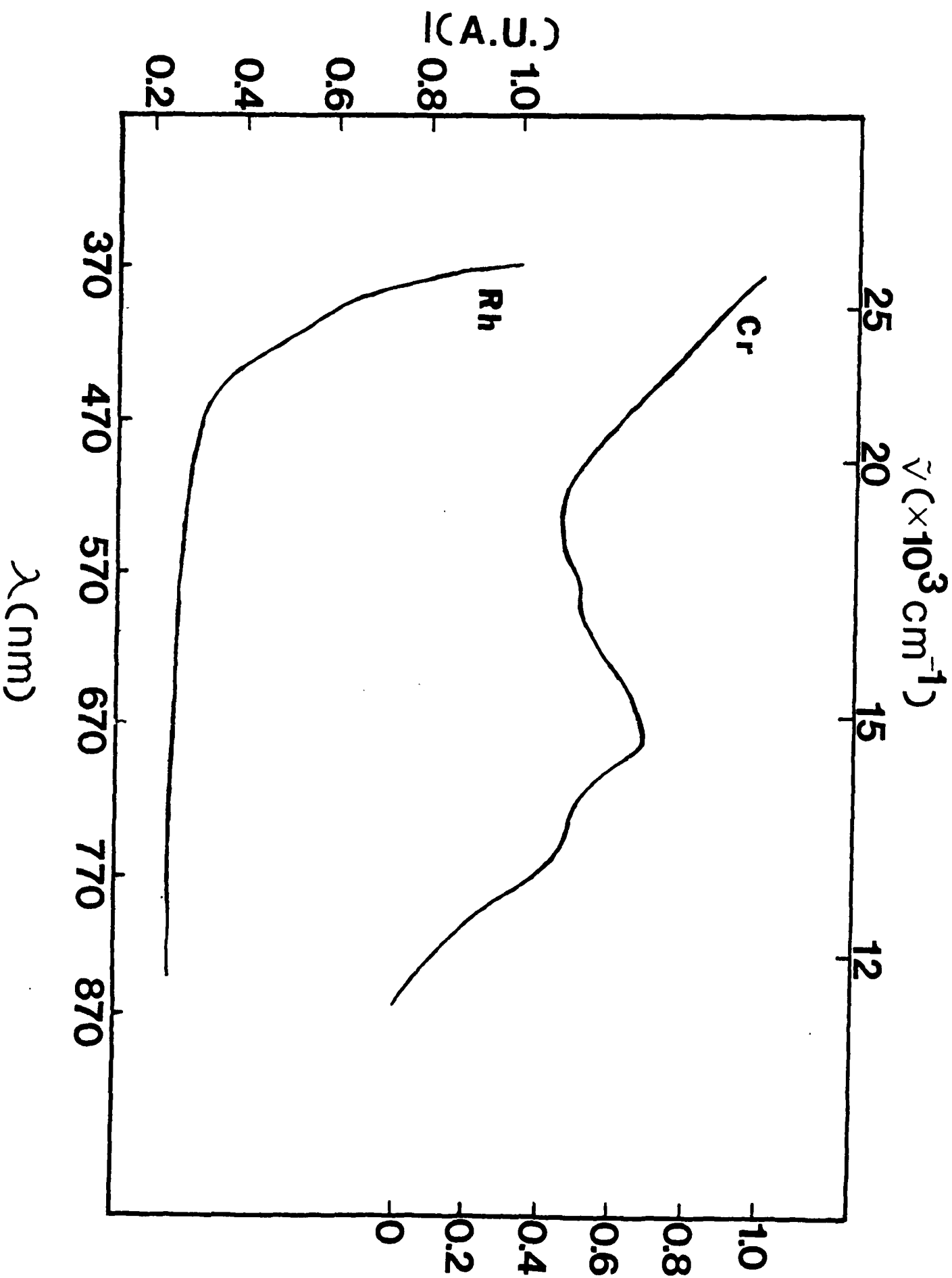
FIG. 1 Room temperature absorption spectra of Cr 3+ and Rh 2+ ions.
