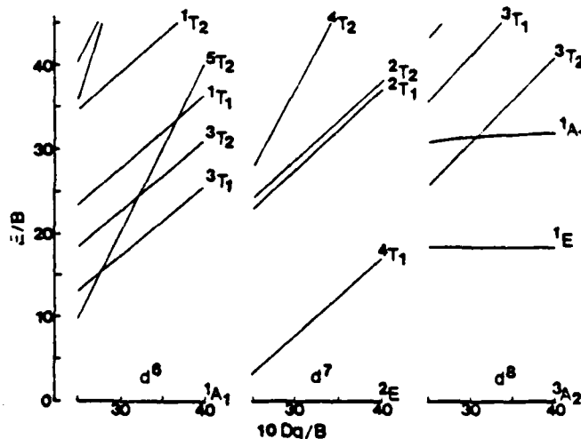
FIG. 1. Portions of crystal field energy level diagrams for d^6 , d^7 , and d^8 ions in octahedral environments.
