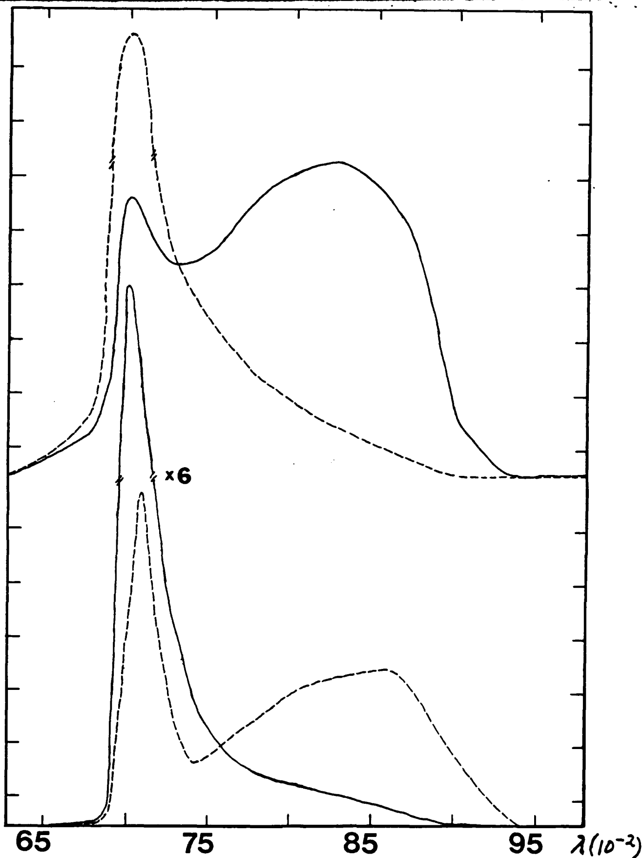
Fig. 2 Fluorescence spectra of \text{Cr}^{3+} in Na \beta -alumina. TOP: T=300 K; solid line for 25 \mu\text{s} after excitation pulse; broken line for 200 \mu\text{s} after excitation pulse. BOTTOM: T=10 K; broken line for 25 \mu\text{s} after the excitation pulse; solid line for 200 \mu\text{s} after the excitation pulse.
