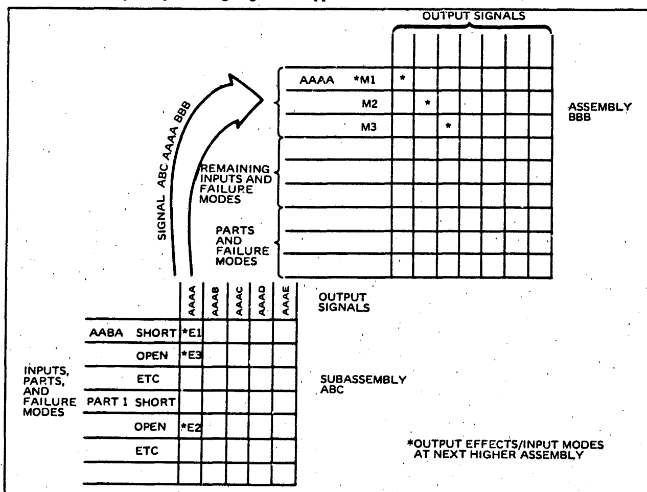
Figure 8. Traceability Between Hardware Indenture Levels in a Matrix FMEA
