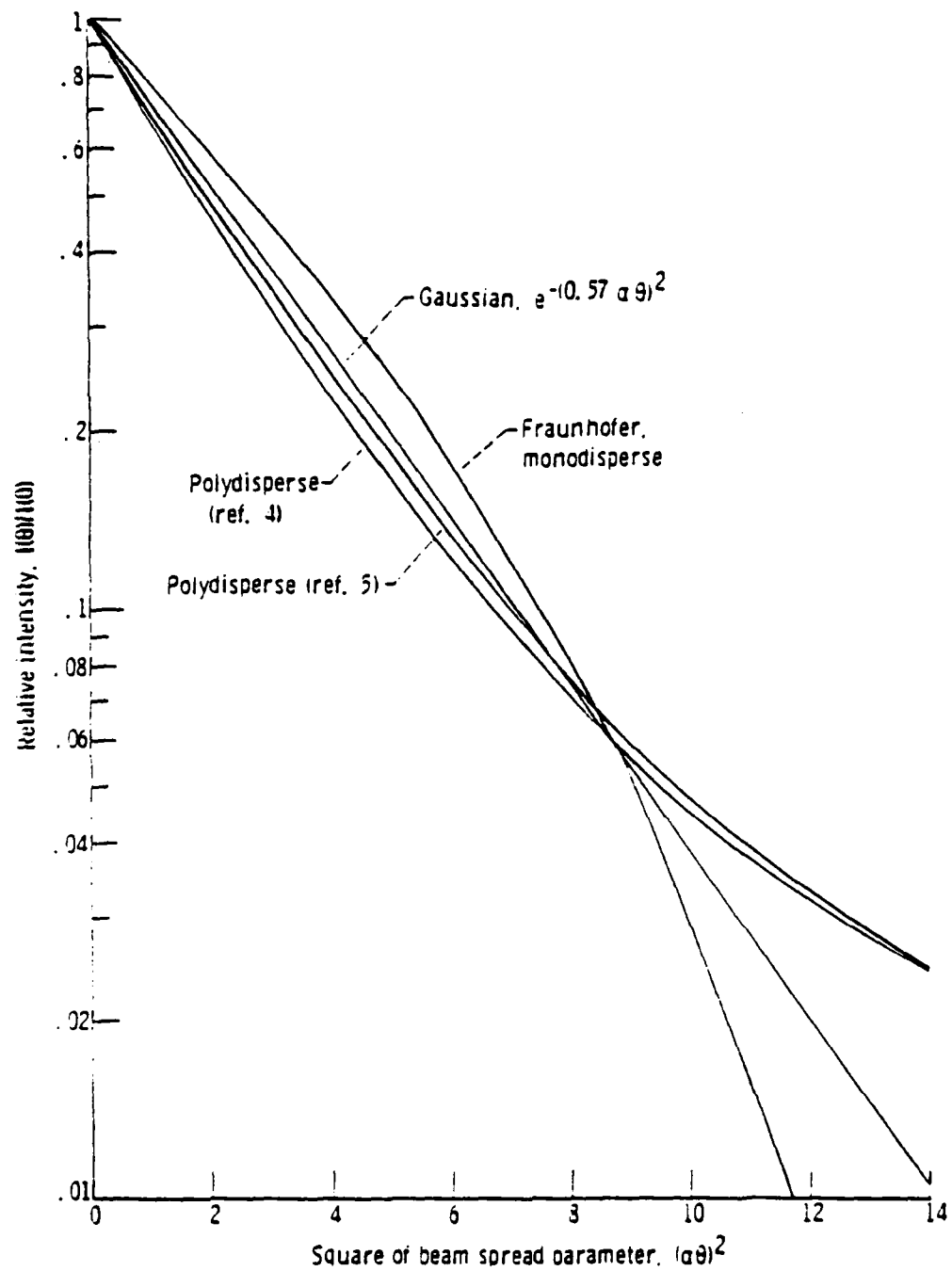
Figure 2.1 Distribution of Forward-scattered Light (Reproduced from [Ref. 5]).
