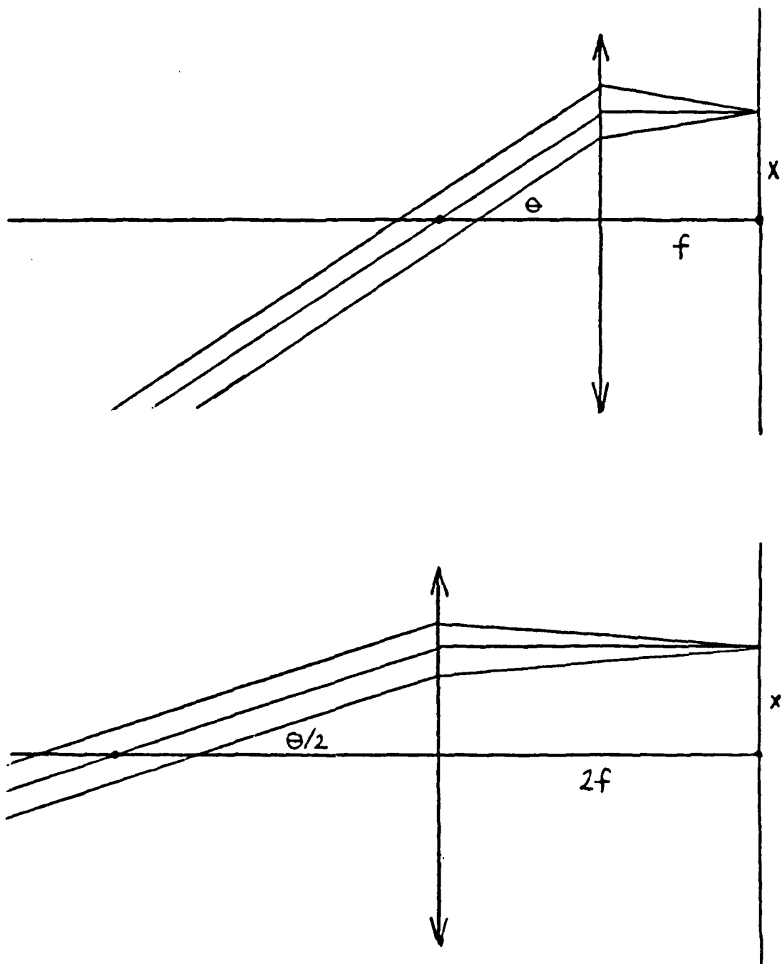
Figure 2.3 Optical System as Equivalent Thin Lens
