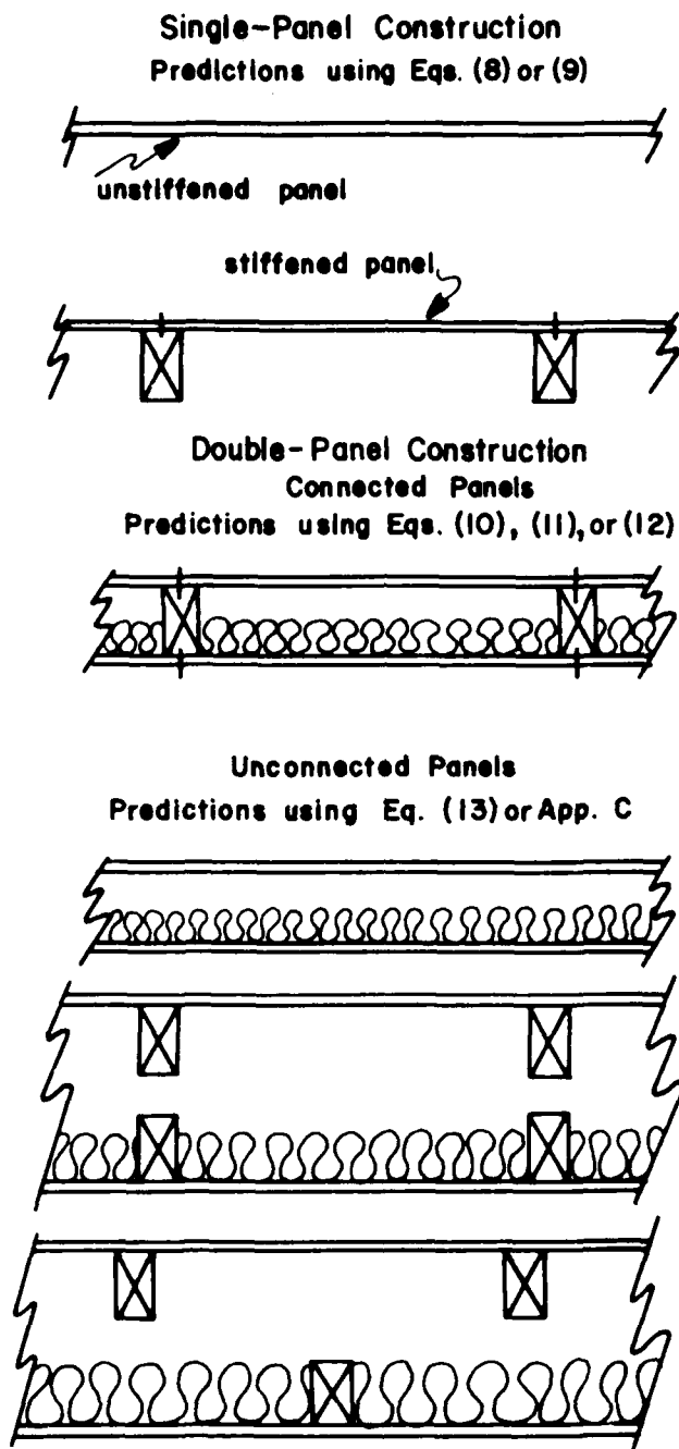
Figure 7.—Panel configurations for which prediction methods apply. ML84 5566)
