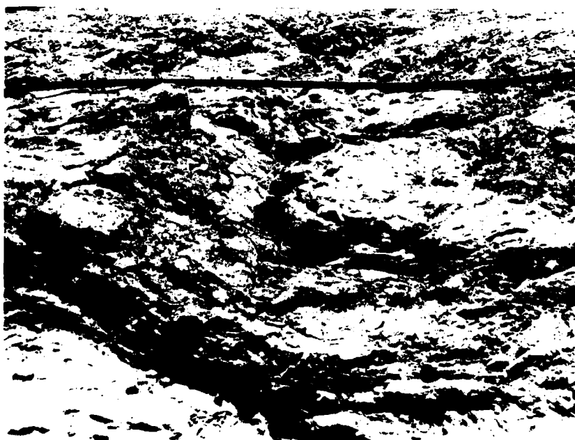
6. Harry S. Truman Dam, 27 July 1966, Neg. No. R-245-4. Cutoff Trench Sta. 50+80 to Sta. 51+00. Looking downstream.
