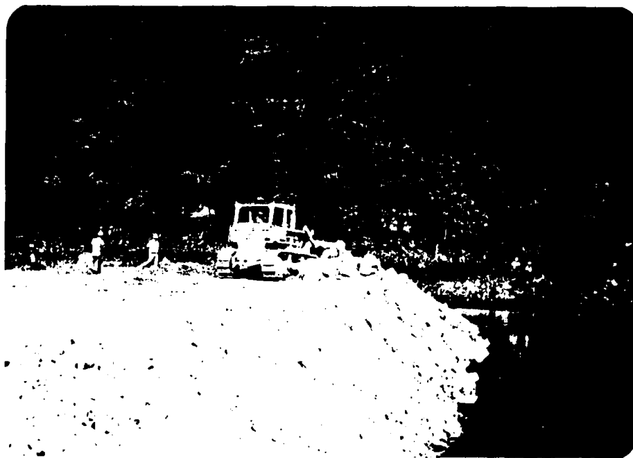
183. Harry S. Truman Dam, 21 July 1977, Neg. No. 77-390. Constructing upstream rock fill coffer dam for closure. Looking at left abutment.
