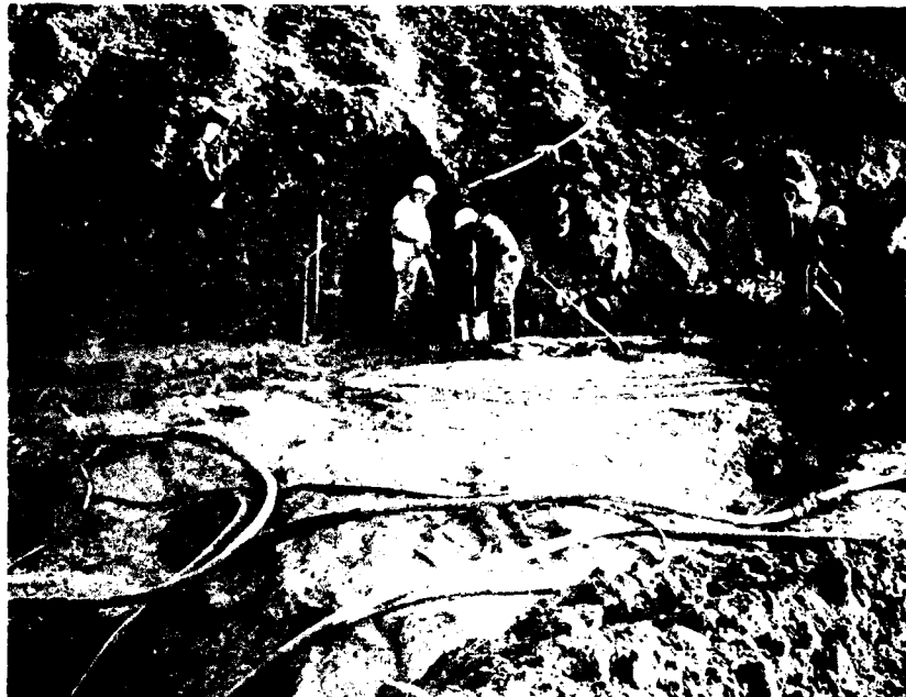
33. Harry S. Truman Dam, 14 November 1966, Neg. No. 82750. Cutoff Trench Sta. 25+00 downstream wall.
