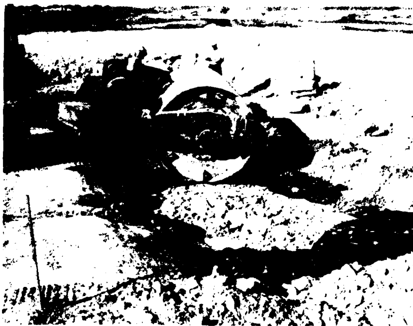
B-13. Sample beign compacted with roller. 30 September 1968, Neg. No. 1020-10
