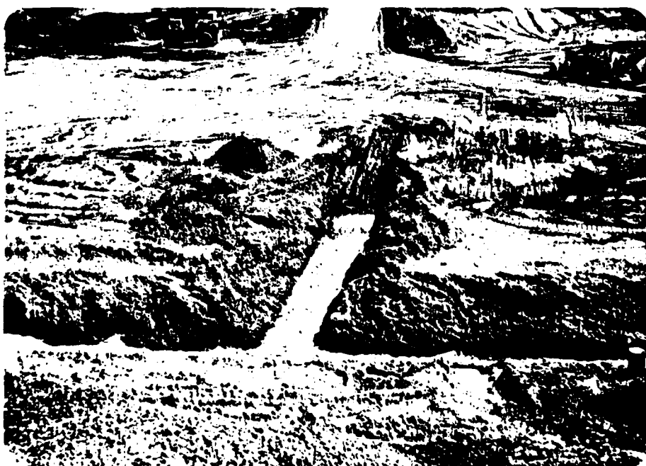
193. Harry S. Truman Dam, 22 September 1977, Neg. No. 77-537. Dewatering trench in basal gravel, closure area.
