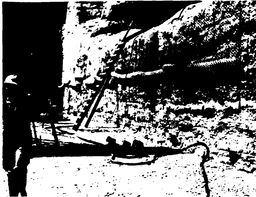
117. Harry S. Truman Dam, 26 June 1972, Neg. No. 965-4. Spillway-Powerhouse. Left wall of Monolith 13. Looking upstream. Ready for concrete lift 8.
