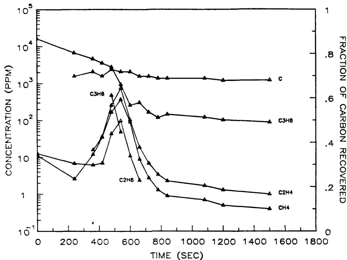
Figure 10. Transient exhaust gas hydrocarbon concentrations: Inlet temperature = 700°K, propane/air equivalence ratio = 0.35, reference velocity = 5 m/s.
