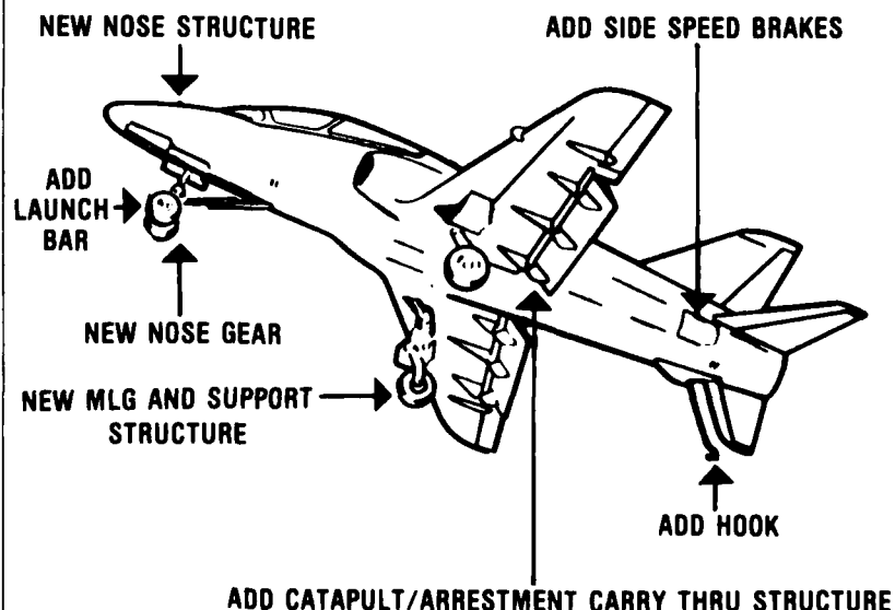
Figure 2. T45A Design Differences
