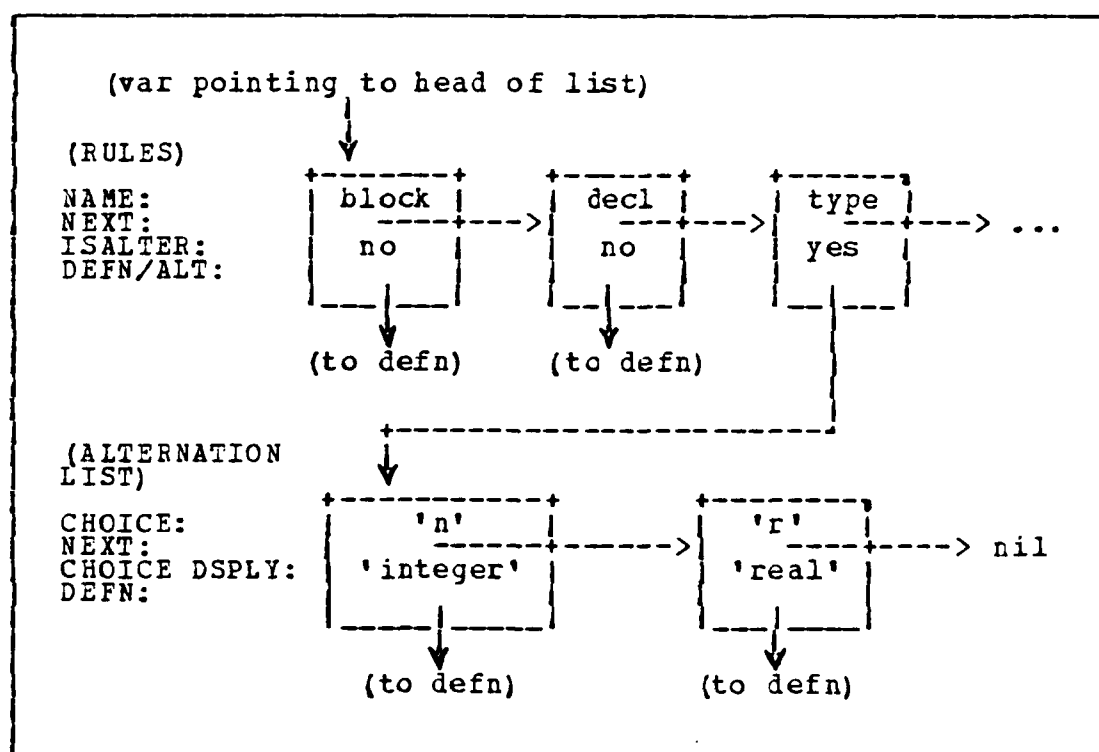
Figure 4.2 Storage of Rules in Minigol Grammar
