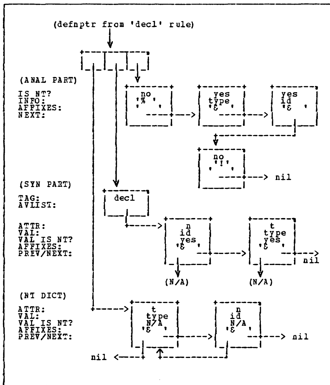
Figure 4.3 Definition Portion of "decl" Rule
