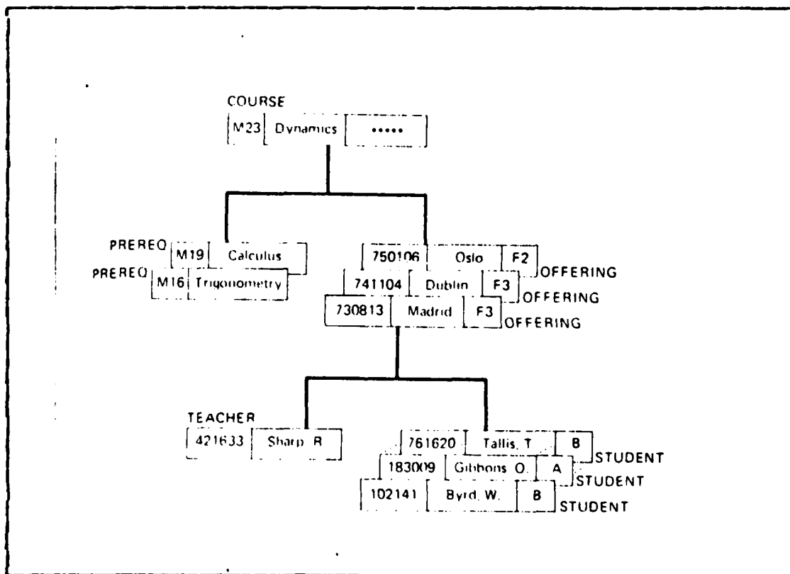
Figure 5.4 Hierarchical View of Database
