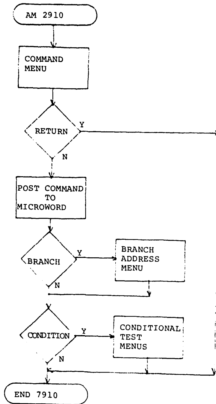
Figure 56 2910 Command Flow Chart
