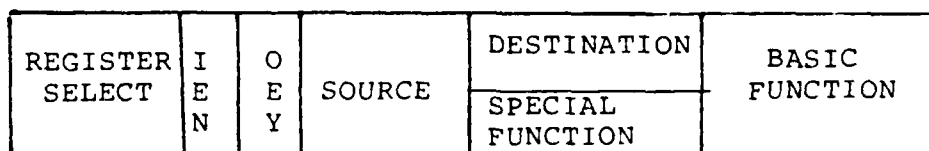
Figure 12 AN29293 ALU Portion of the Microinstruction
