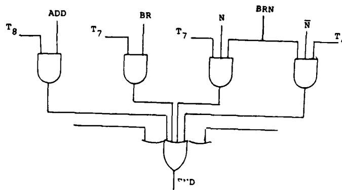
Figure 2 [Ref. 4: p 113] Implementation of Logic Equation
