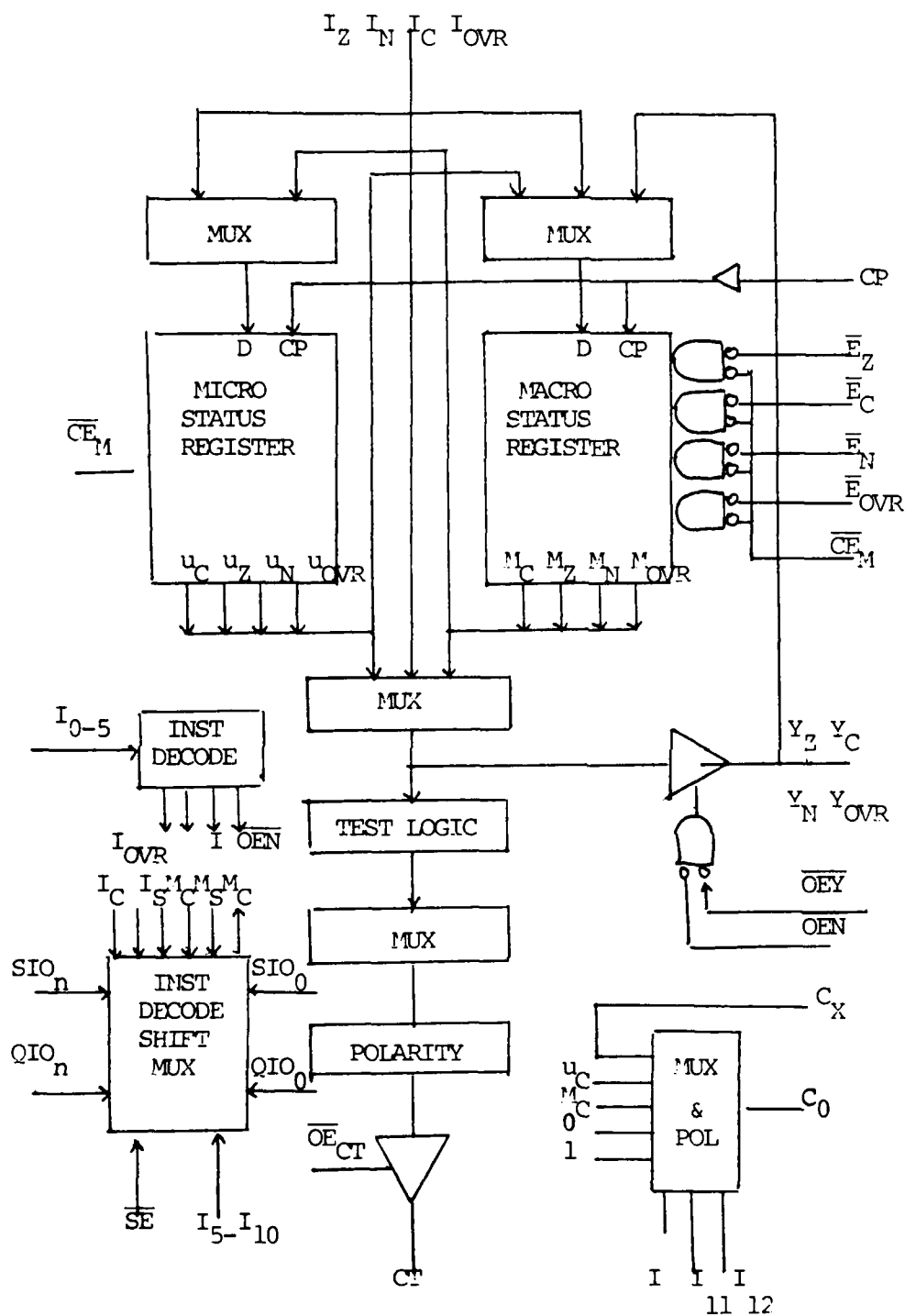
Figure 10 [Ref. 13: p. 8-2] Block Diagram AM2904
