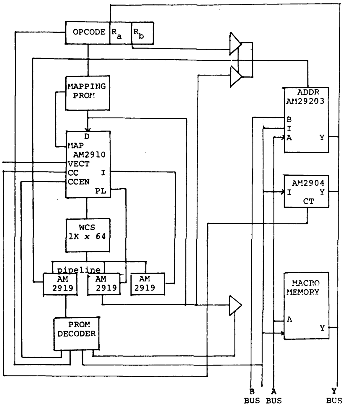
Figure 6 [Ref. 12: 9-2] Block Diagram of AM29203 Evaluation Board
