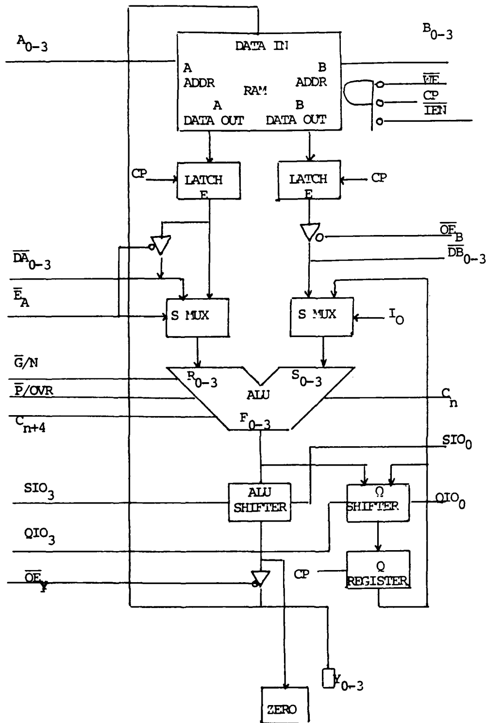
Figure 8 [Ref. 13: p. 2-16] Block Diagram of AM2903
