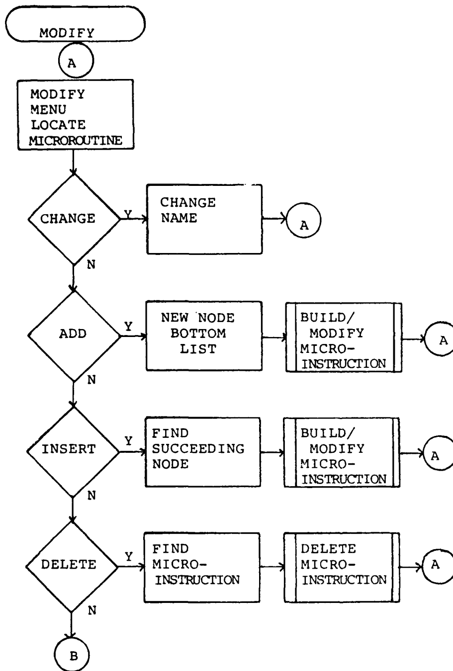
Figure 30 Modify Microroutine Logic
