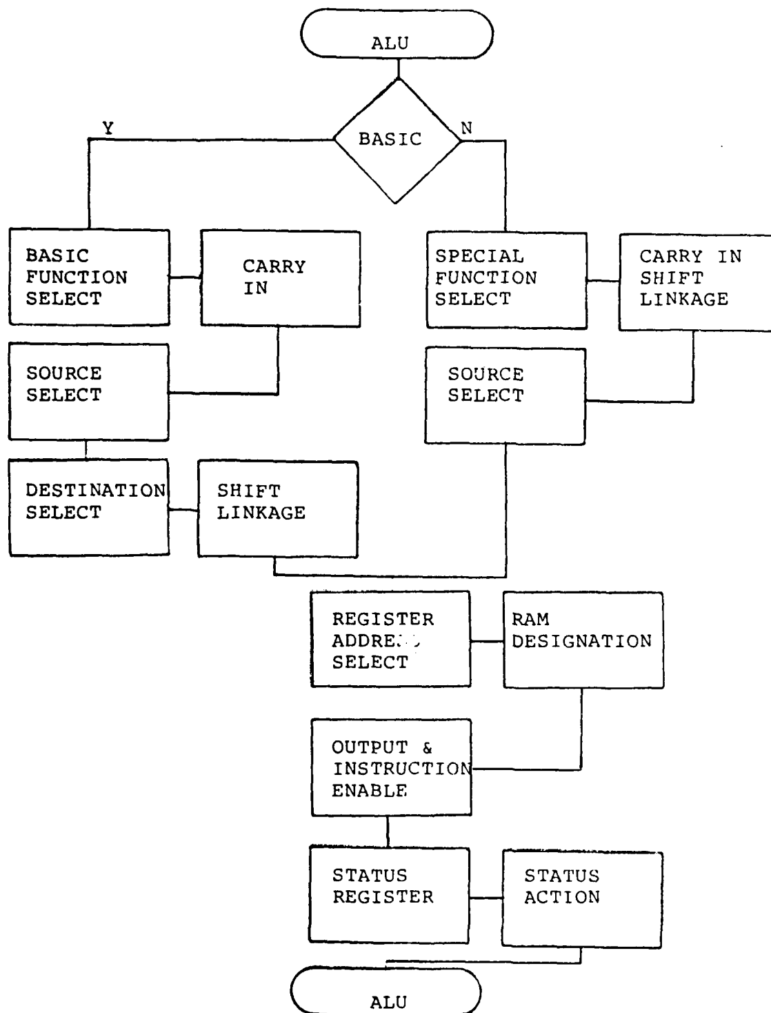
Figure 33 ALU Logic
