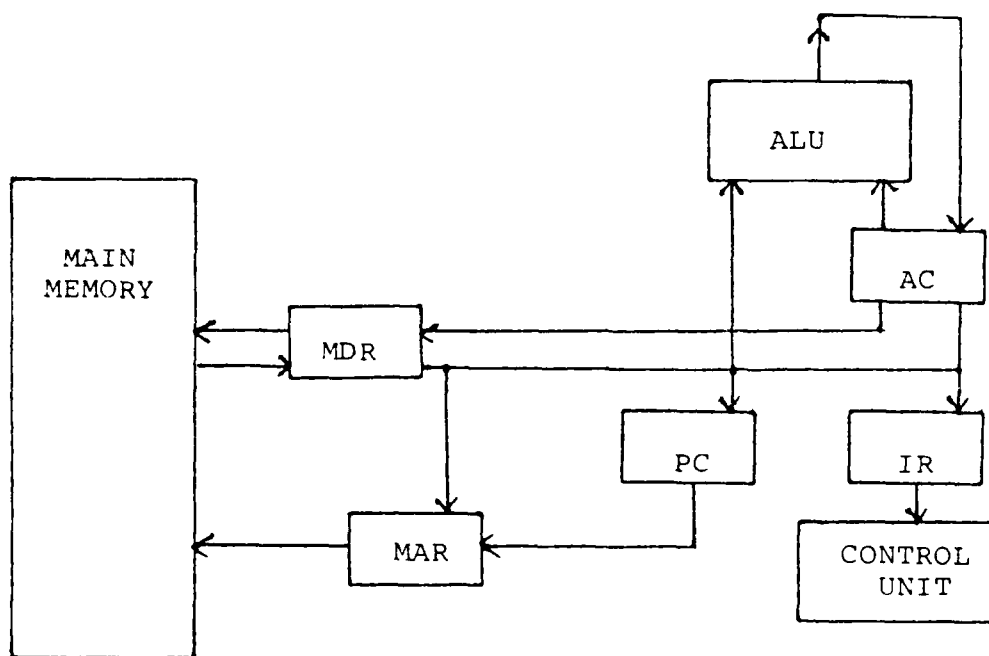
Figure 1 [Ref 5: p 269] Sample Hardware Configuration
