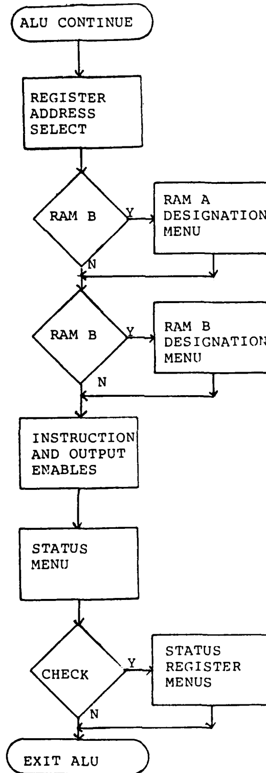
Figure 46 Remainder ALU Processing
