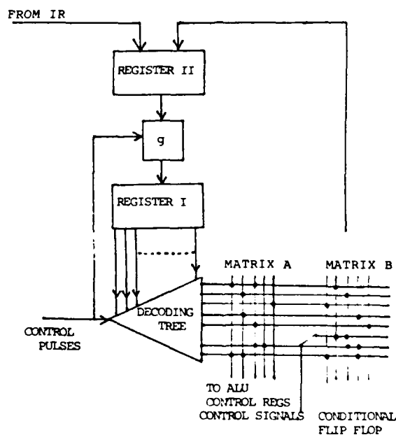
Figure 4 [Ref. 1: p 159] Wilkes' Original Design of a Microprogrammed Control Unit
