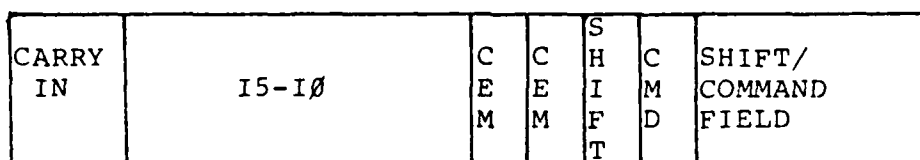
Figure 13 AM2904 Shift/Status Control Portion of Microinstruction
