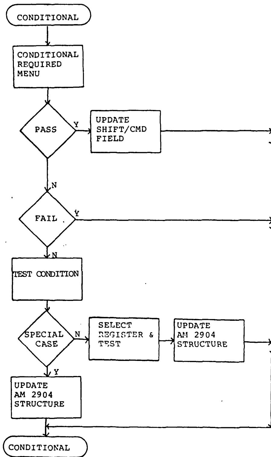
Figure 59 Conditional Test Select Flow Chart
