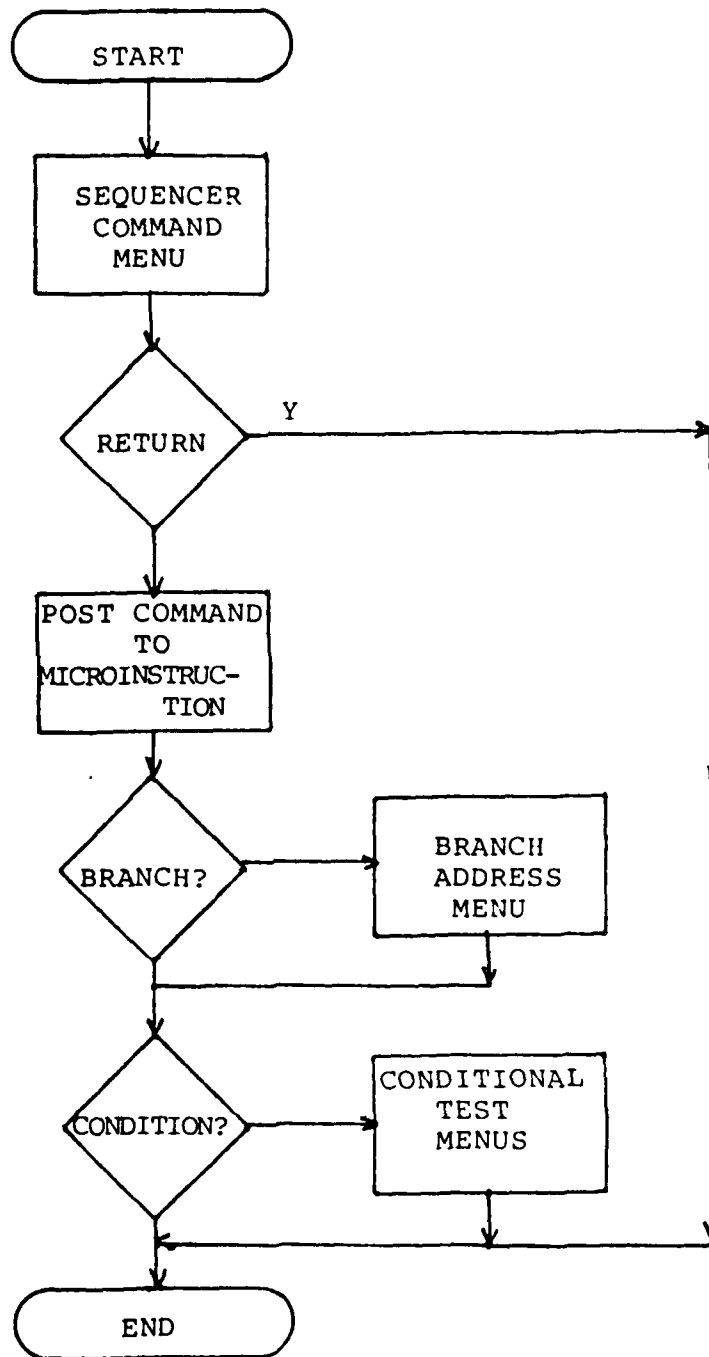
Figure 5 Next Microinstruction Address
