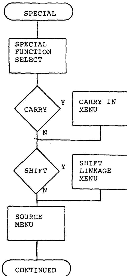
Figure 43 Processing of a Special ALU Function
