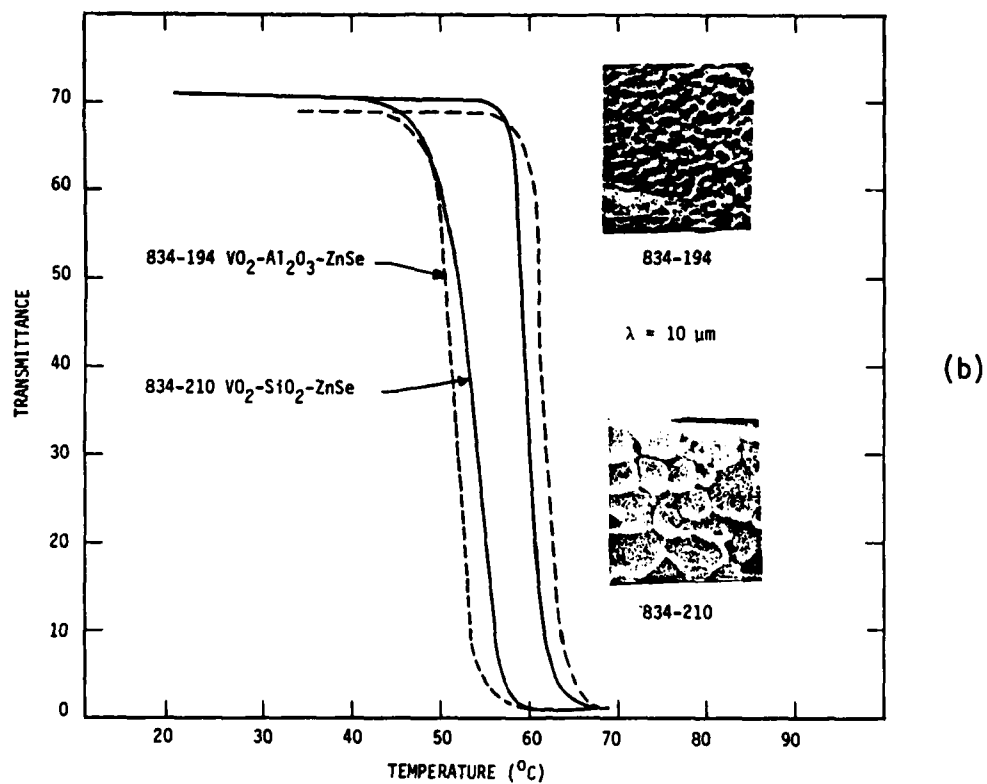
Figure 5: Transition Modification vs. Grain Size
