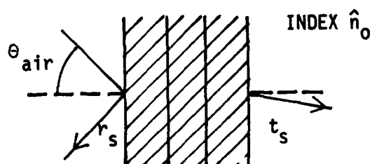
Figure 2. Separation of the Generic Configuration into Modules and Specification of Amplitude Reflection and Transmission Coefficients for Each Part.
