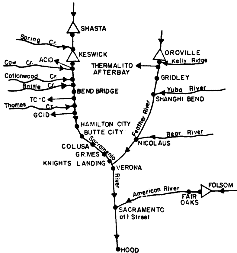
Figure 2 SACRAMENTO VALLEY RESERVOIR SYSTEM SCHEMATIC
