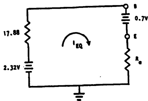
FIGURE 15b: Reflection of Base Into Emitter
