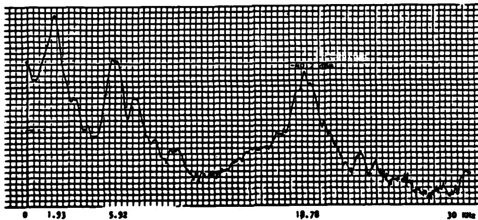
FIGURE 30a: Ground Return (by the HP3585A Spectrum Analyzer)
