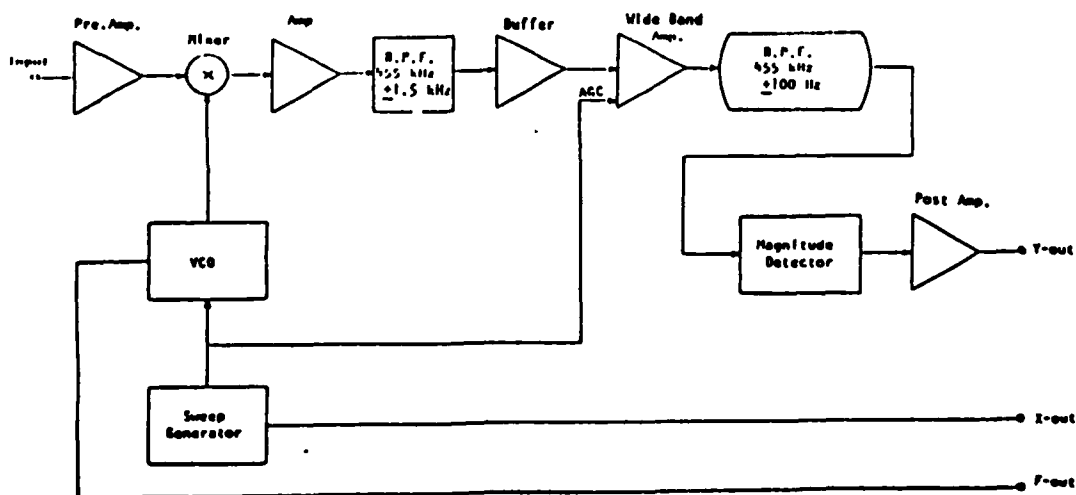
FIGURE 14: Block Diagram of the Spectrum Analyzer
