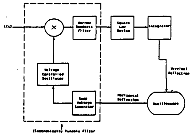
FIGURE 9a: Scanning Spectrum Analyzer
