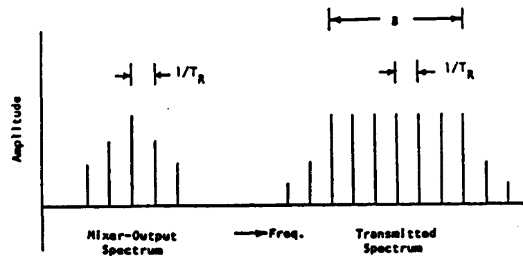
FIGURE 5: Spectrum of Received and Transmitted Signal
