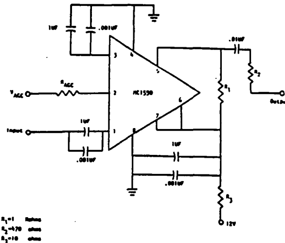
FIGURE 22b: The Wideband Amplifier (Swept Gain Stage)
