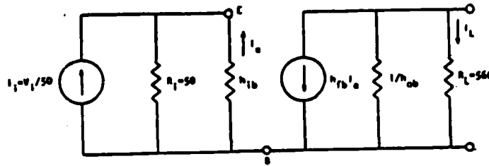
FIGURE 15c: Small Signal Circuit of Pre-Amp
