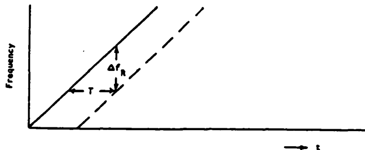
FIGURE 4: Expanded View of Part of Sweep
