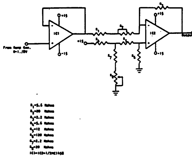
FIGURE 23: The Sweep Network for AGC
