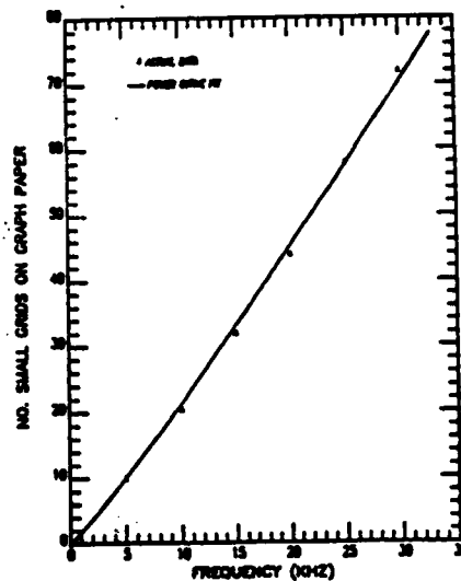
FIGURE 28: Frequency Calibration Curve
