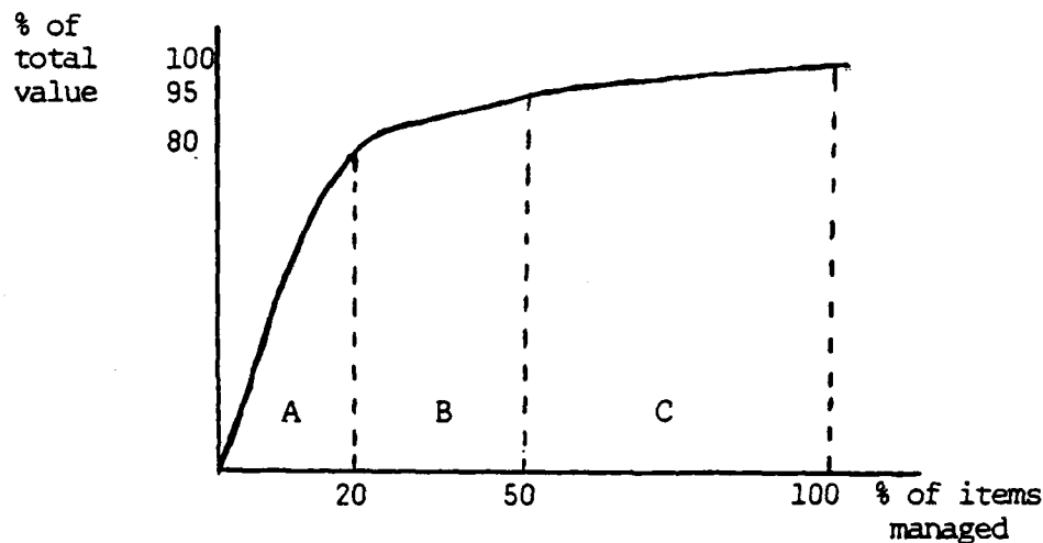
Figure 5. A Typical ABC Curve
