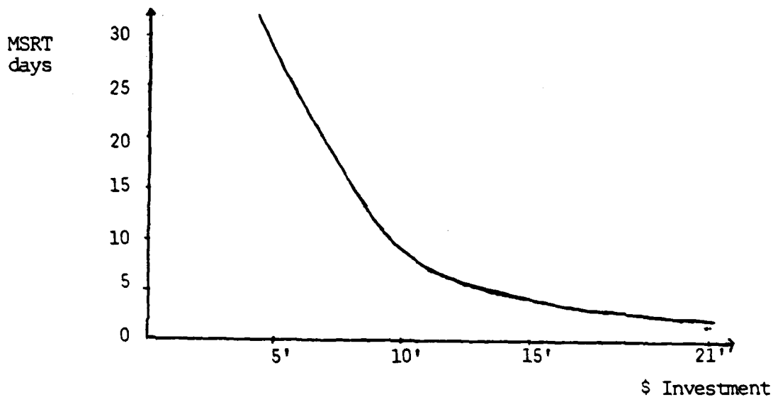
Figure 8. A Cost Effectiveness Curve for the MSRT Model for the Example Data
