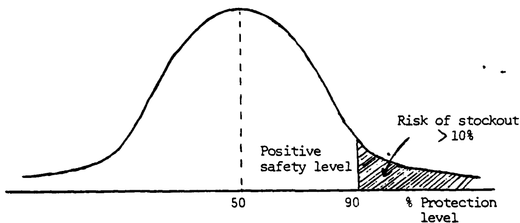
Figure 10. The Protection Level
