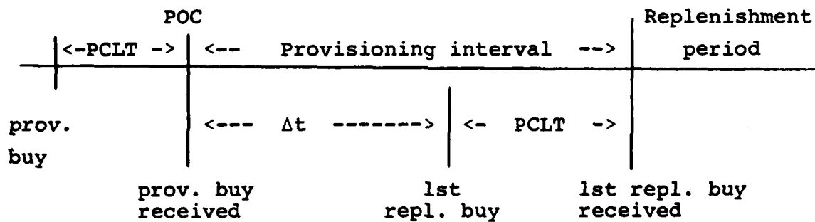
Figure 13. The Provisioning Interval
