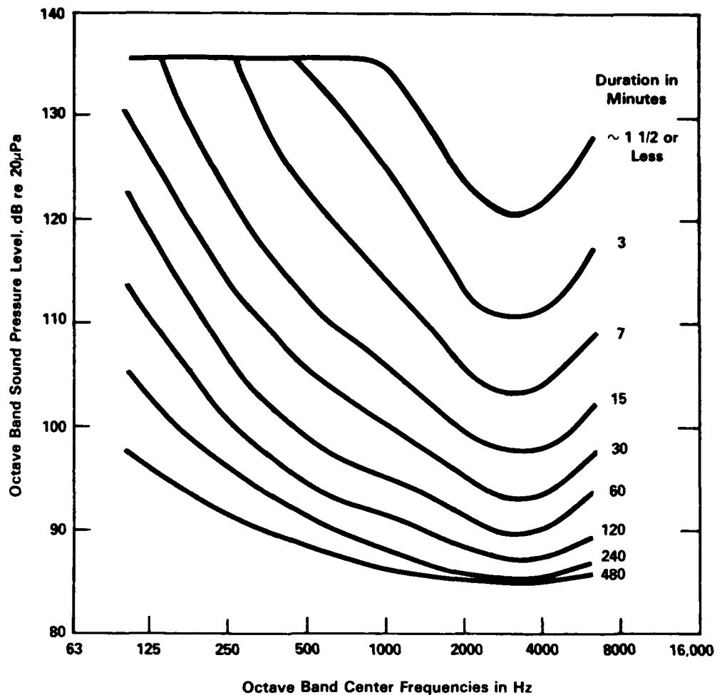
Damage Risk Contours for One Exposure Per Day to Octave Bands of Noise
