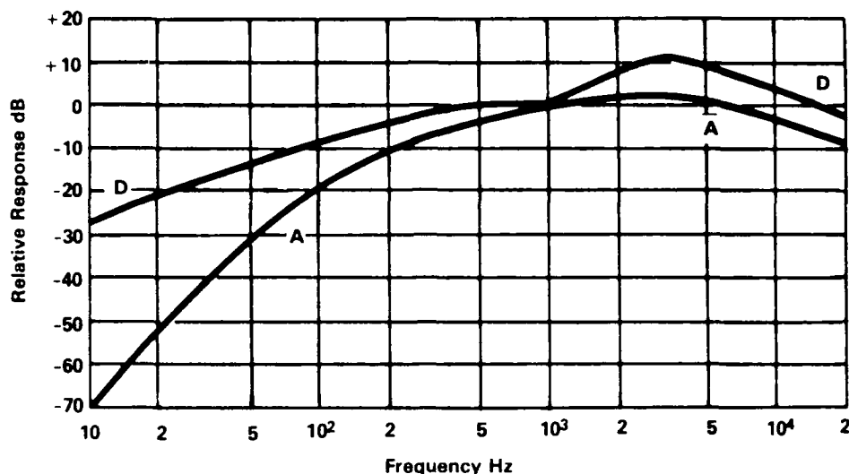
The Internationally Standardized "A" and "D" Weighting Curves for Sound Level Meters
