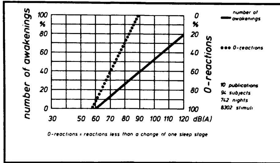
Sleep disturbances by noise—number of reactions and noise level.
