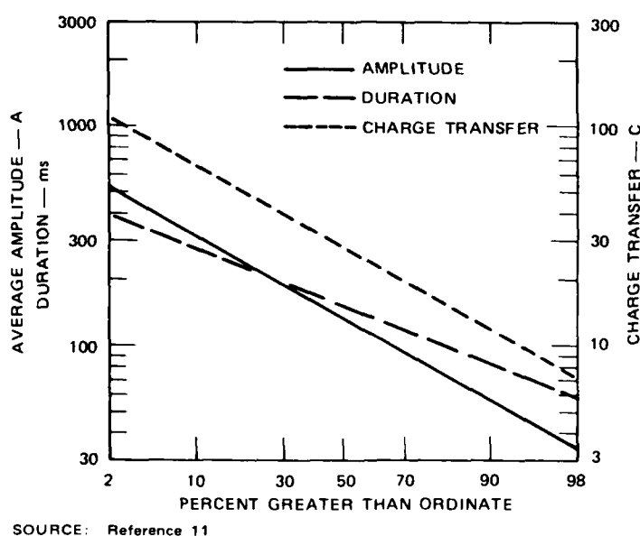
FIGURE 5 STATISTICS FOR CONTINUING CURRENTS--NEGATIVE FLASHES TO GROUND (after Pierce)
