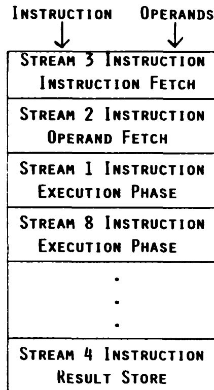
MIMD PIPELINE
