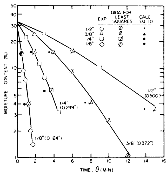
Figure 6.—Douglas-fir heartwood integral press drying curves at various thicknesses. Temperature = 375° F; pressure = 50 lb/in. 2 ; veneer = 1 x 12 x 48 inches; vented caul. (ML 84 5659)
