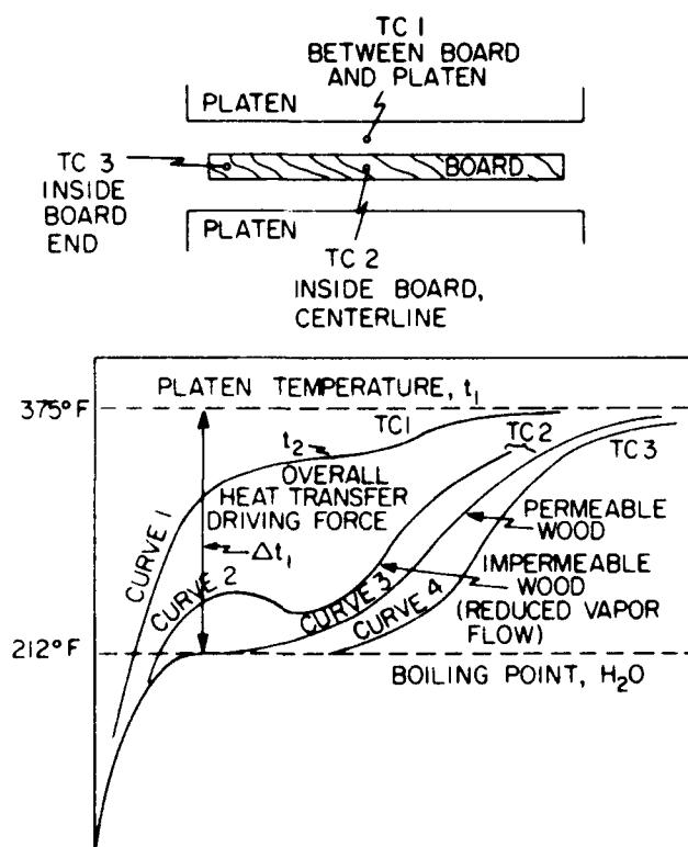
Figure 2.—Thermocouple (TC) locations and schematic temperature-time response of veneer in press drying. (ML 84 5661)
