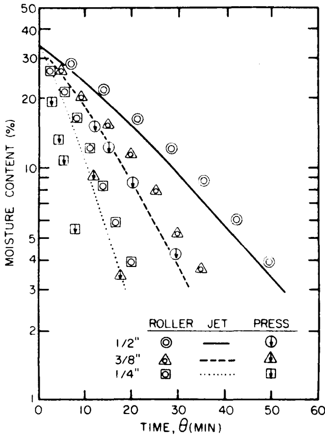
Figure 10.—Douglas-fir heartwood integral drying curves for a single group of veneers dried in roller, jet, and press dryers. Actual average thicknesses were: 1/4" = 0.259"; 3/8" = 0.389"; and 1/2" = 0.516". (ML 84 5665)
