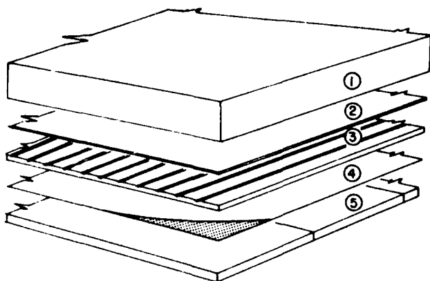
Figure 1.—Caul designs for drying presses.
