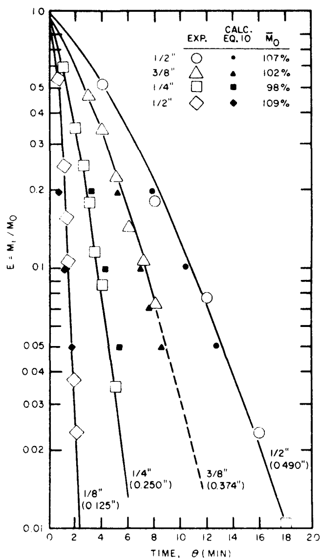
Figure 4.—Southern pine integral press drying curves at various thicknesses. Temperature = 375° F; pressure = 50 lb/in. 2 ; veneer = 1 × 12 × 48 inches (t (decimal) = actual average measured thickness; fraction = thickness class); vented caul. (ML 84 5663)
