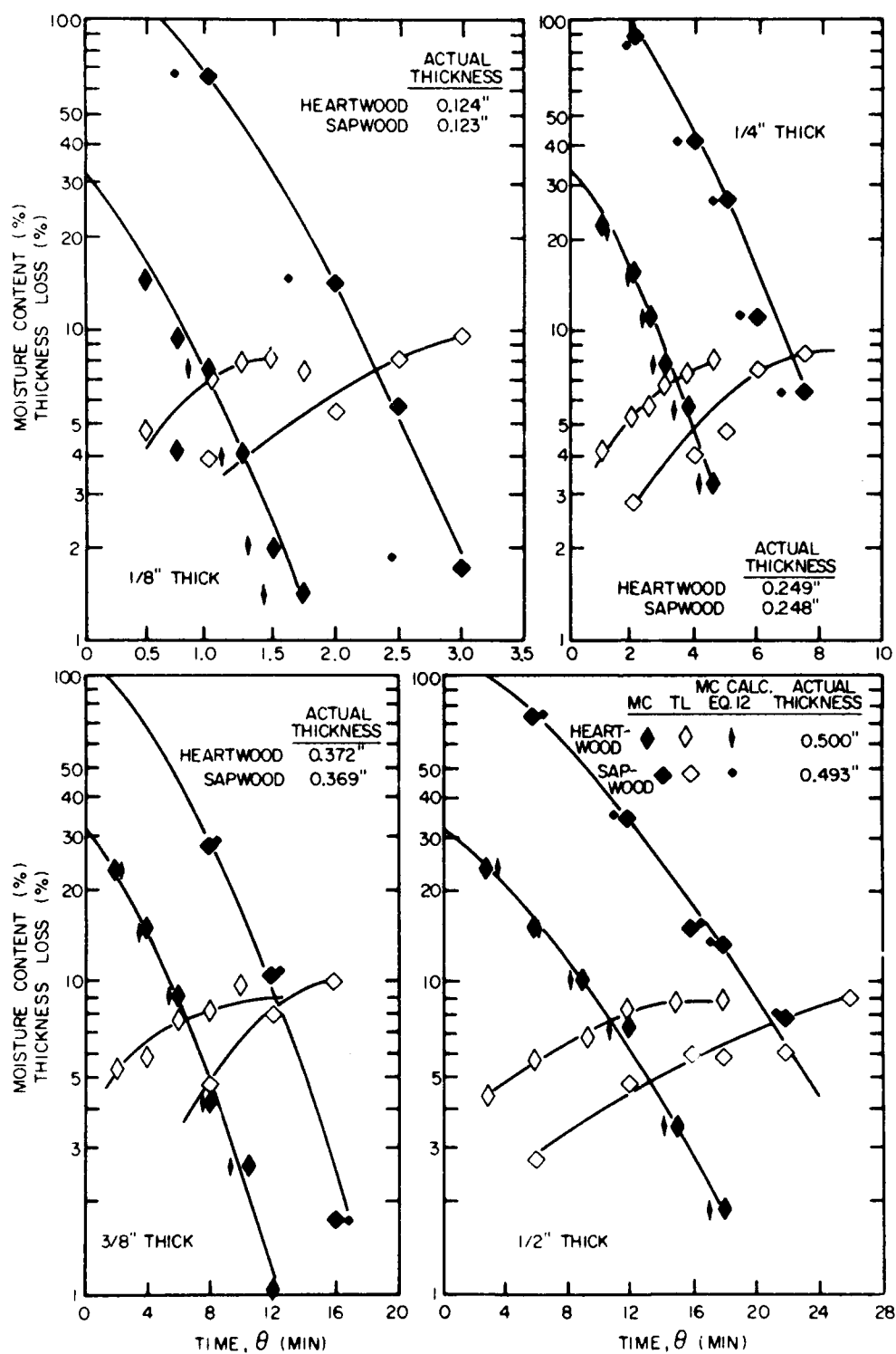
Figure 8.—Douglas-fir integral press drying curves (moisture content) and percent thickness loss, for heartwood and sapwood, for four thickness classes. (ML 84 5666)
