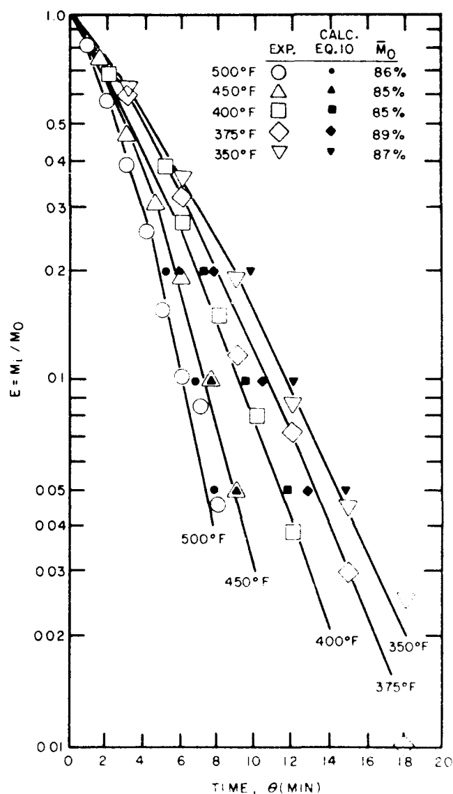
Figure 5.—Southern pine integral press drying curves at various temperatures. Pressure = 50 lb/in. 2 ; veneer = 0.5 × 12 × 24 inches; unvented caul. (ML 84 5662)
