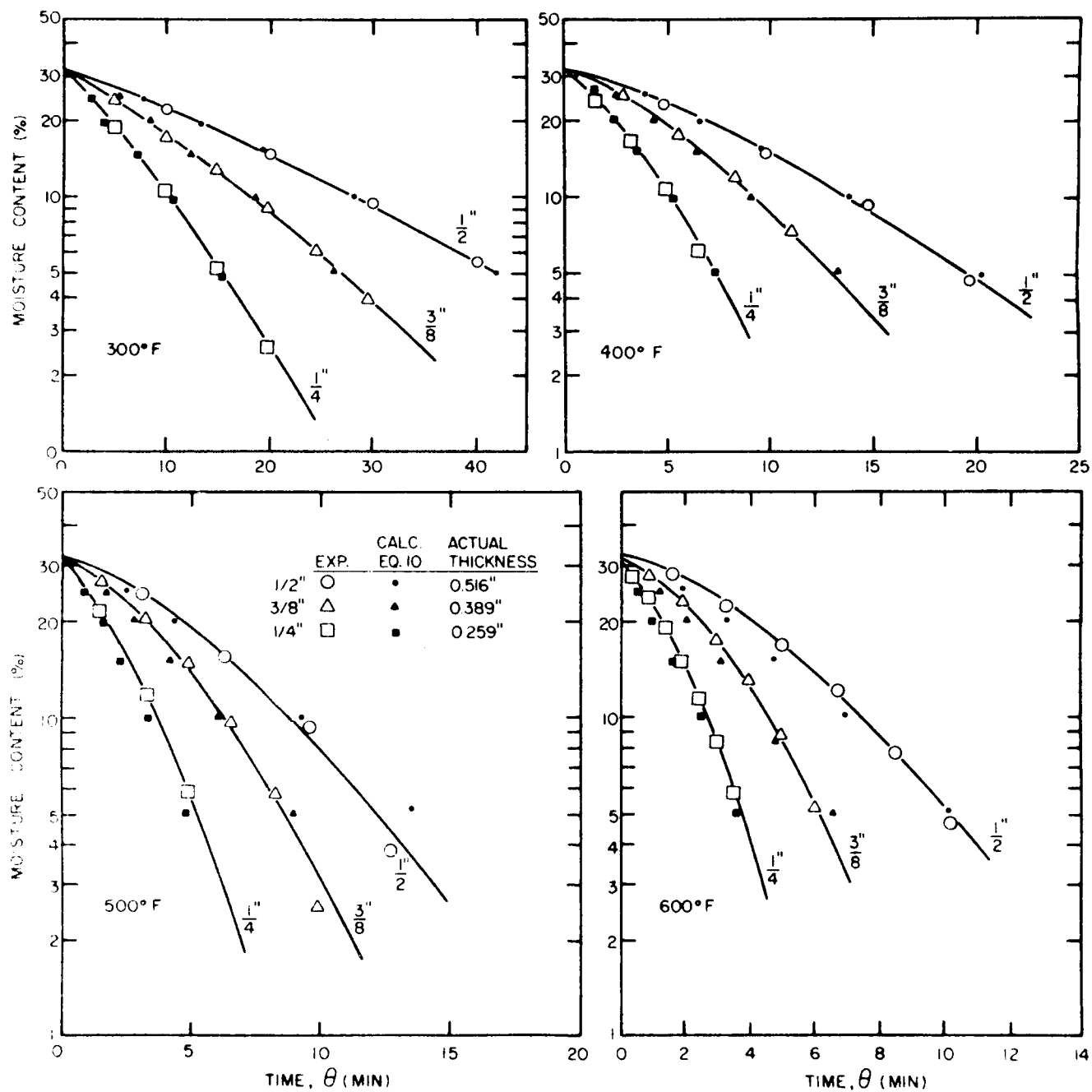
Figure 9 — Douglas-fir heartwood integral jet drying curves, for three thicknesses, at four temperatures. (ML 84 5667)
