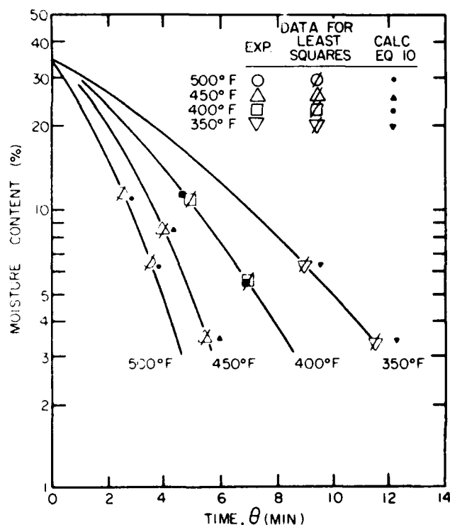
Figure 7.—Douglas-fir heartwood integral press drying curves at various temperatures. Pressure = 50 lb/in. 2 ; veneer = 0.42 x 12 x 24 inches; unvented caul. (ML 84 5660)
