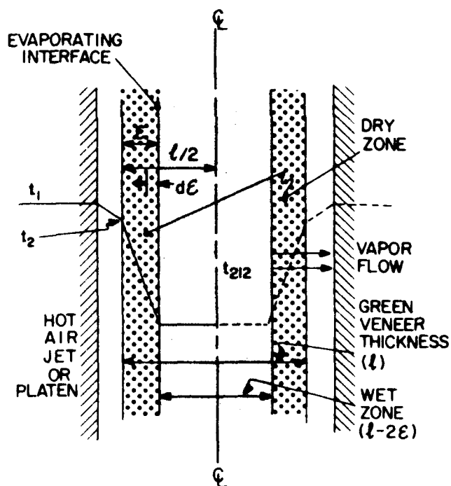
Figure 3.—Model for heat transfer and vapor flow in press drying thick veneer. (ML 84 5664)
